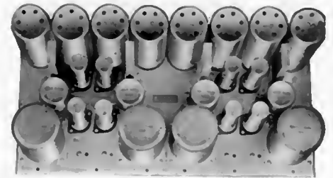
116B Pre-amplifier — Used in 124F, 124G and other amplifiers. Employs dc bias gain control.
