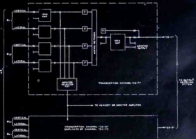
TRANSCRIPTION CHANNELS
