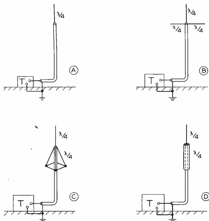
Fig. 5—Evolution of the coaxial antenna.
