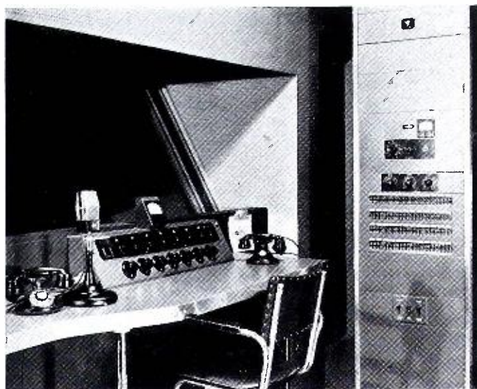
Cabinet type racks house the Western Electric 104A, 105A and 94C amplifiers with which each studio is equipped. The design of the control console permits, full, unobstructed view of the studio.
