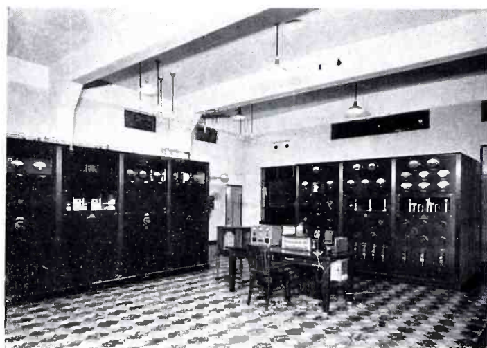
Two views of the Western Electric 50 kw. transmitter at KSL.
