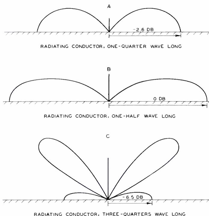
Fig. 3—Vertical directivity patterns for grounded vertical antennas.
