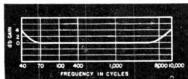
Fig. 5. Preamplifier gain characteristic for overall equalization.
