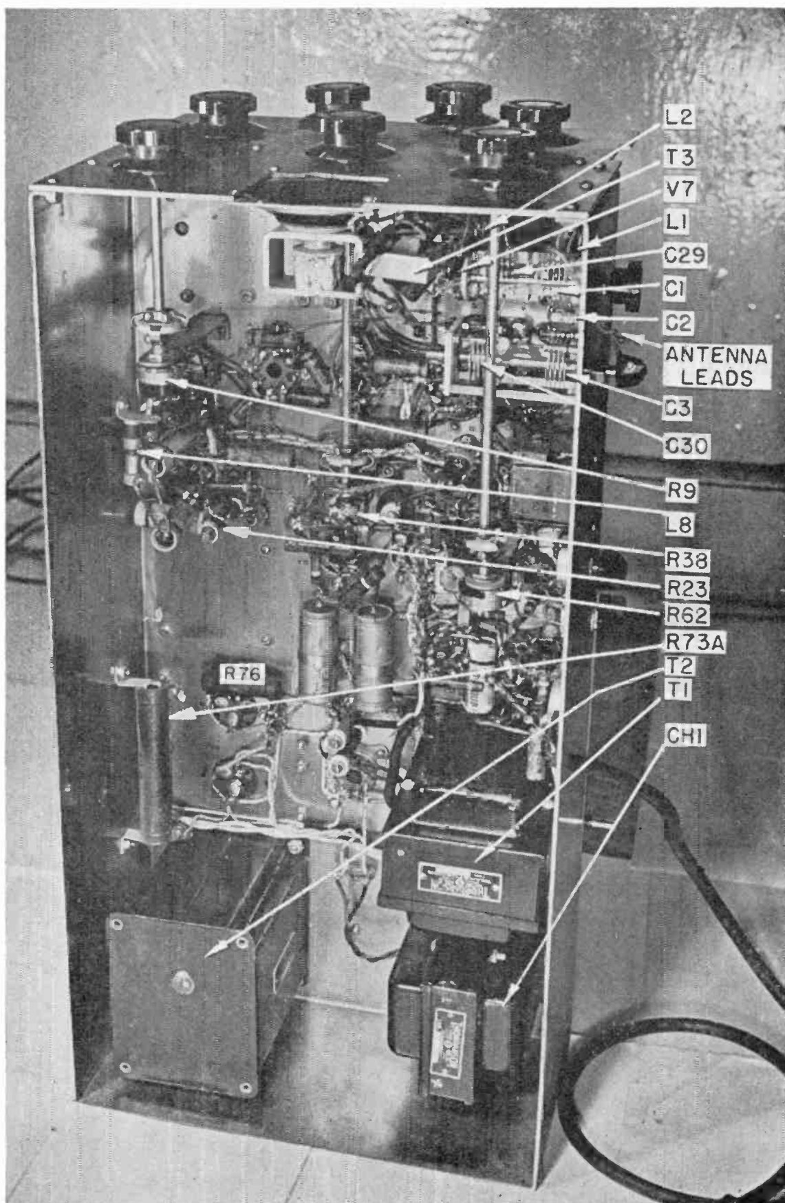
Fig. 3. Under-chassis view of completed receiver. Note that all components are grouped closely to form their respective stages. Sound trap, L_4 (not visible in the photo), is mounted directly under the tuning condensers, C_3 , C_{30} .
