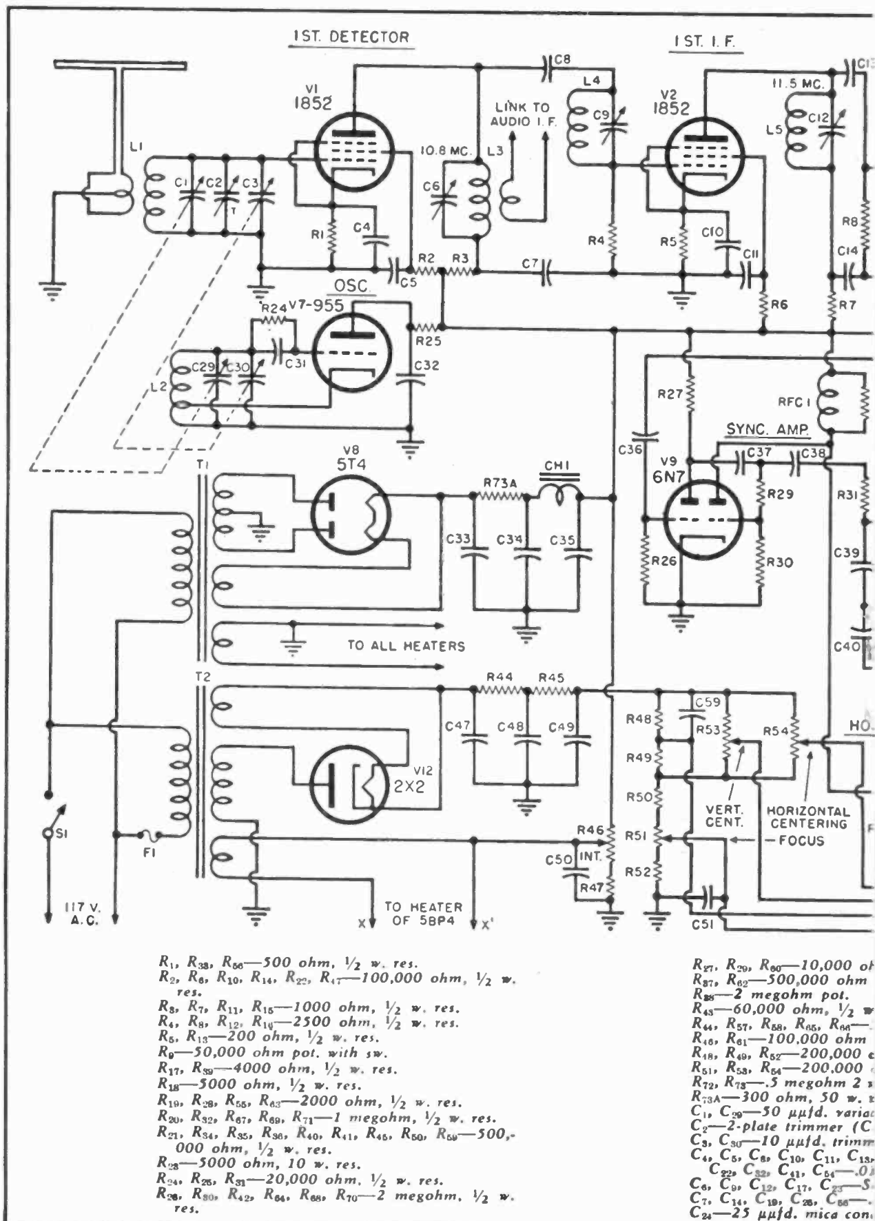
Fig. 2. Complete schematic diagram of the video section of the home-built television r
