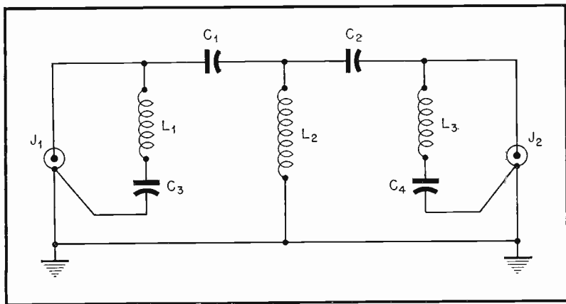
Fig. 3. High-Pass Filter for Coaxial Lead-in.
