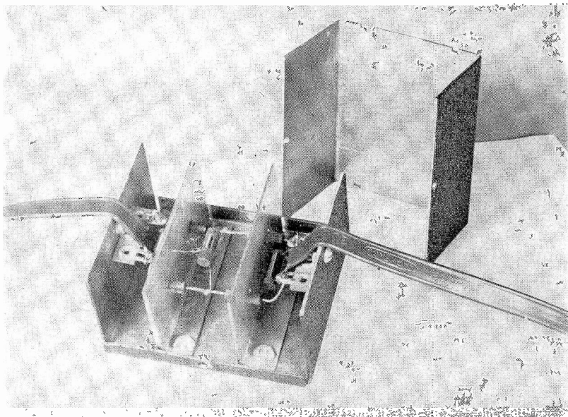
Fig. 1. High-Pass Filter for 300-ohm Antennas and Receivers.
