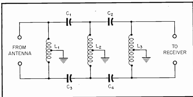
Fig. 2. High-Pass Filter for 300-ohm Lead-in.
