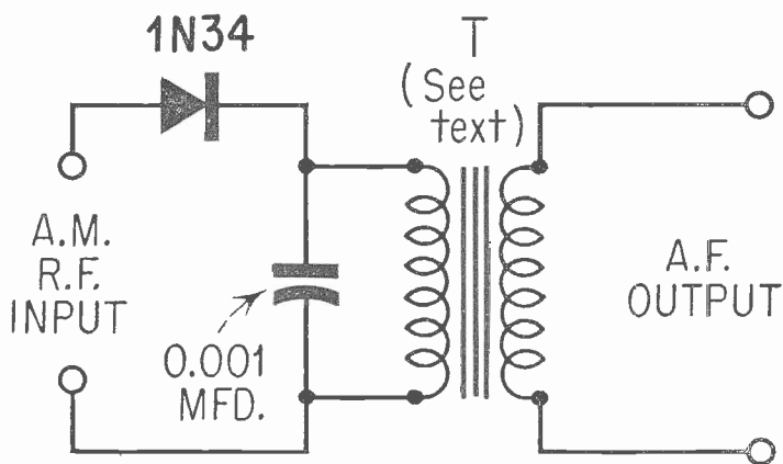
(B) TRANSFORMER TYPE
