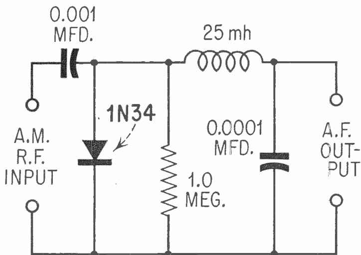
(A) R-C TYPE
