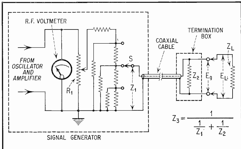
Fig. 2. Signal Generator Output Circuit.
