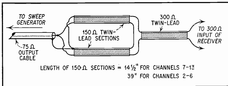
Fig. 4. Matching Section for 75 - 300 Ohms.
