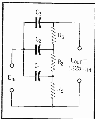
Fig. 4. Roddam's Rearrangement of the "Phase-Shift" Circuit of Figure 3(A).
