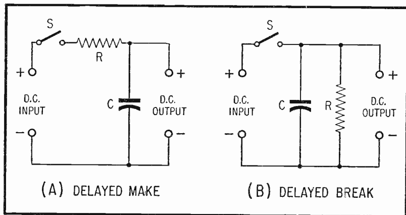
Fig. 1. Basic RC Timing Circuits.
