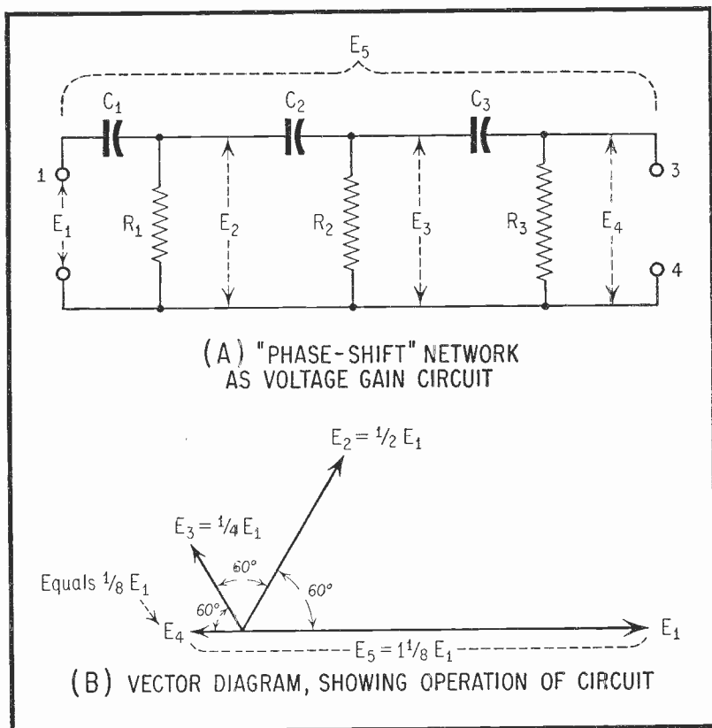
Fig. 3. Illustration of Voltage Gain in RC Circuit.
