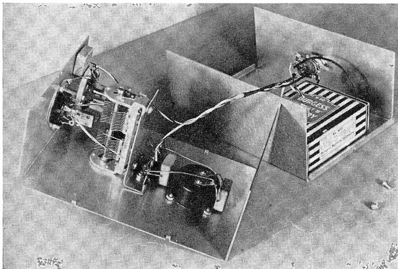
Fig. 2. Internal View, showing construction and wiring. Compare with the layout sketch, Fig. 4, for identification of parts and battery location with respect to meter and tuning capacitor.
