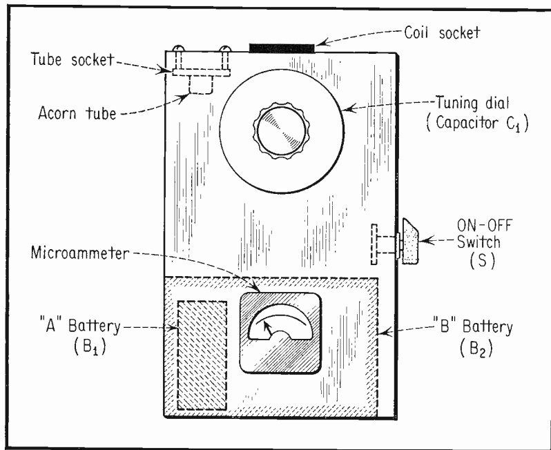
Fig. 4. General Layout of Grid-Dip Meter.
