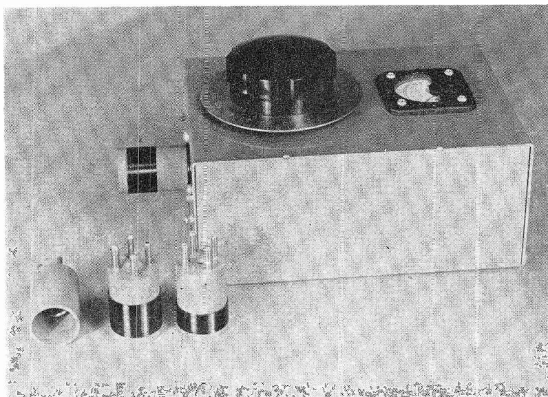
Fig. 1. External View of the Grid-Dip Meter with Experimental Coils. The small, battery-operated instrument is light enough to be held in one hand while being operated.
