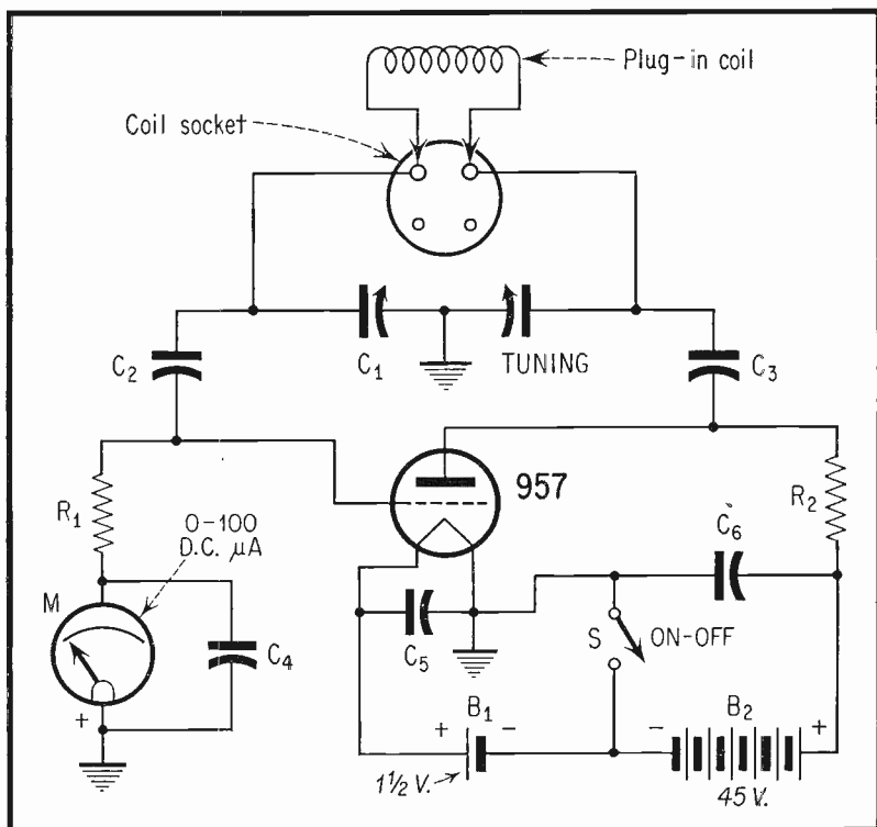
Fig. 3. Complete Circuit of the Grid-Dip Meter.
