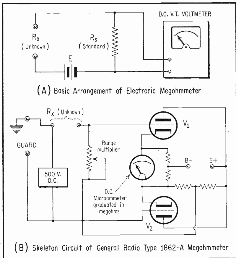
Fig. 3. Laboratory-Type Megohmmeter.
