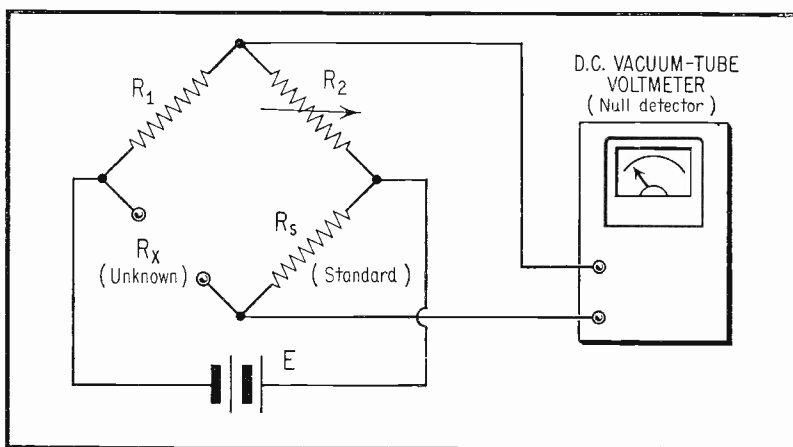
Fig. 4. Basic Resistance Bridge for High Values.
