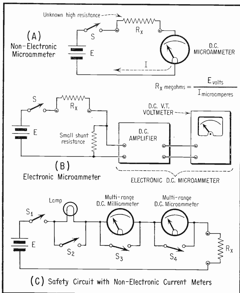
Fig. 1. Current-Meter Measurement Circuits.
