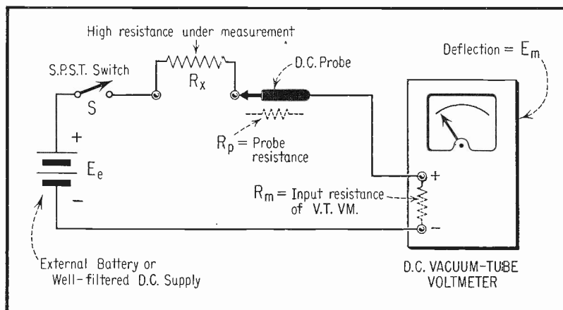
Fig. 2. Arrangement for High-Resistance Measurements with D.C. Vacuum-Tube Voltmeter.
