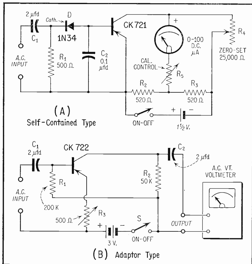
Fig. 3. Audio-Frequency Millivoltmeters.
