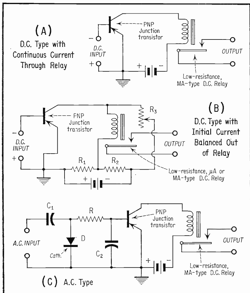
Fig. 1. Basic Transistorized Relays.
