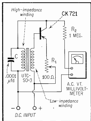
Fig. 4. DC-AC Converter.
