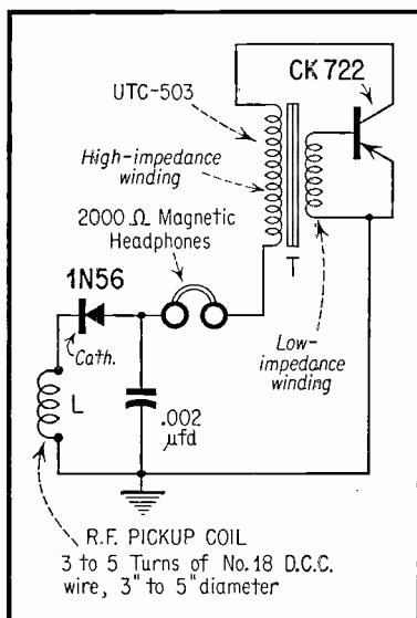
Fig. 5. C.W. Keying Monitor.
