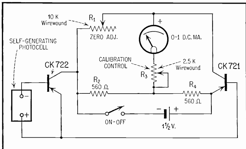
Fig. 6. High-Sensitivity Light Meter.
