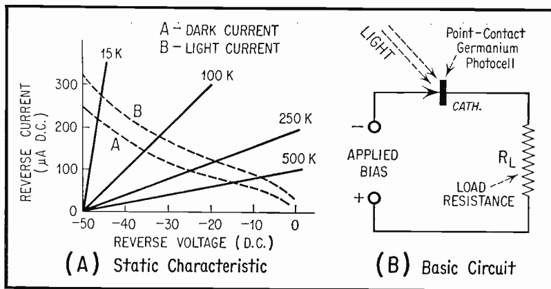
Fig. 2. Point-Contact Germanium Photocell.
