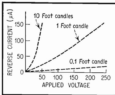
Fig. 3. Cadmium Sulphide Photocell Characteristics.
