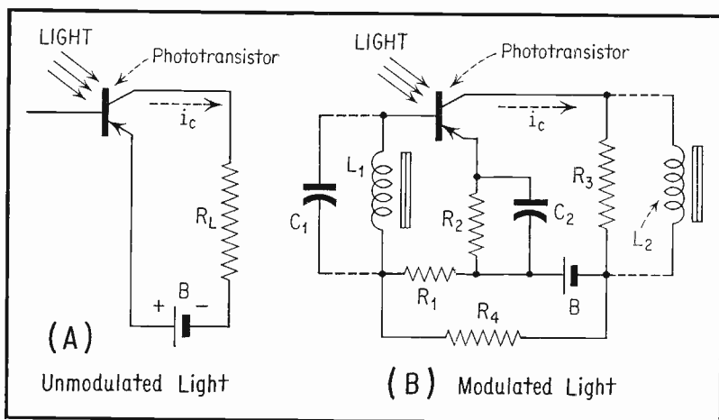
Fig. 6. Phototransistor Circuits.
