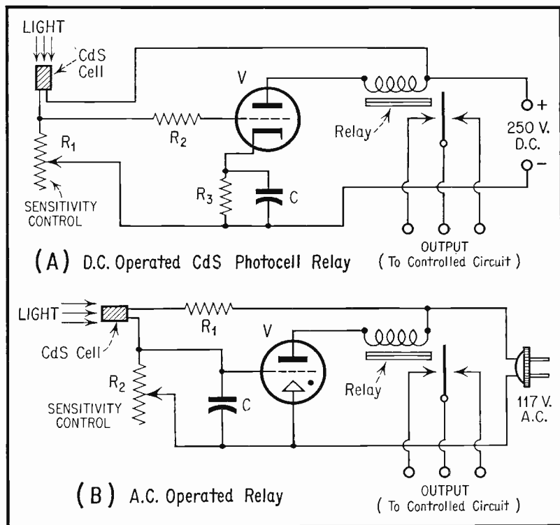
Fig. 4. Cadmium Sulphide Photocell Circuits.
