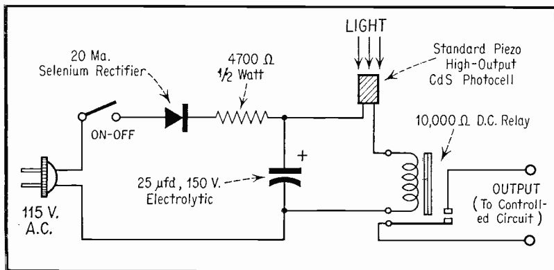
Fig. 5. High-Output CdS Photocell Relay.
