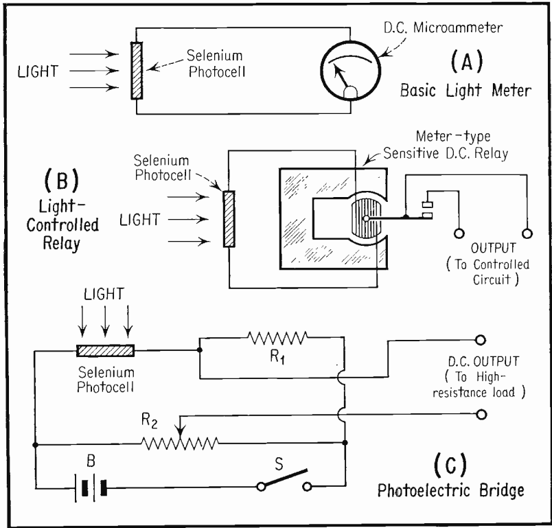
Fig. 1. Selenium Cell Circuits.
