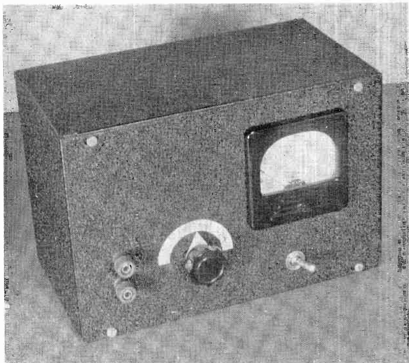
Fig. 1. The Completed Frequency Meter. Only the signal-input terminals, range switch, meter and ON-OFF switch appear on the front panel.
