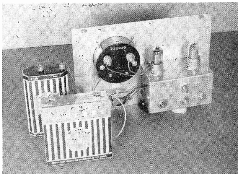
Fig. 2. Inside Construction. Calibration rheostats are seen on the rear of the chassis box.
