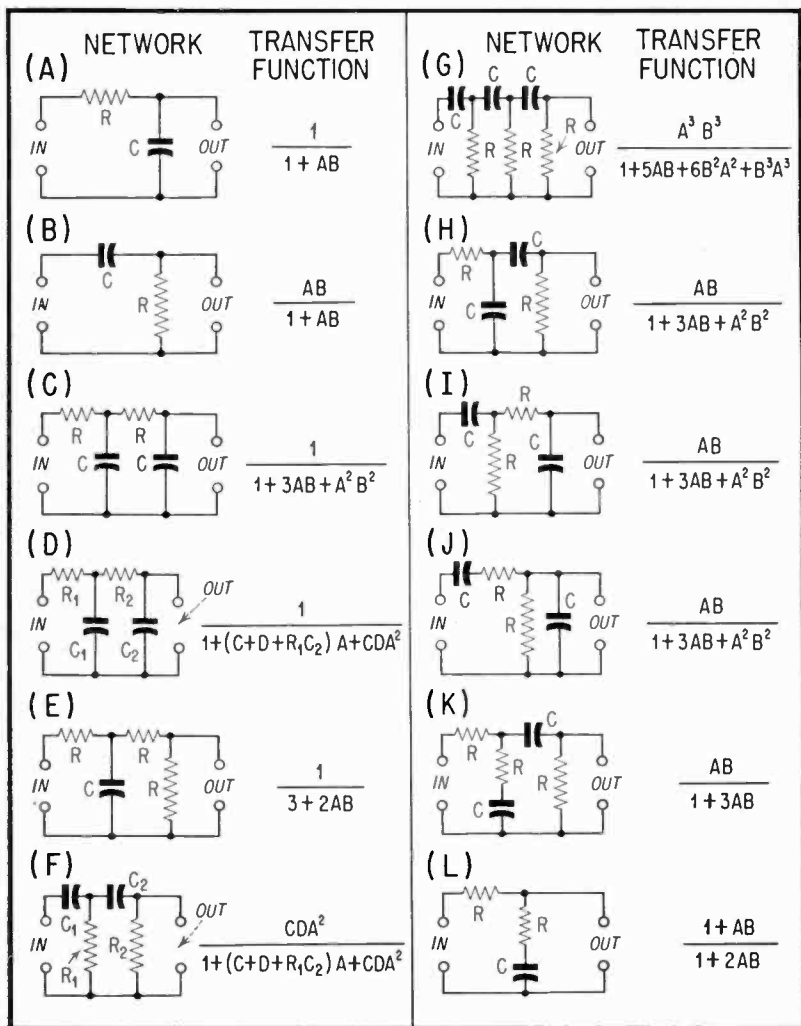
Fig. 4. Typical Networks Obtainable with the Synthesizer.
