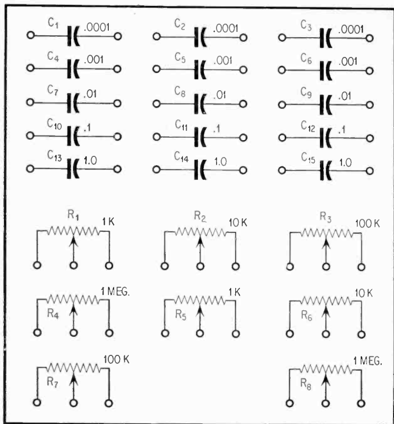
Fig. 2. Circuit of RC Network Synthesizer.
