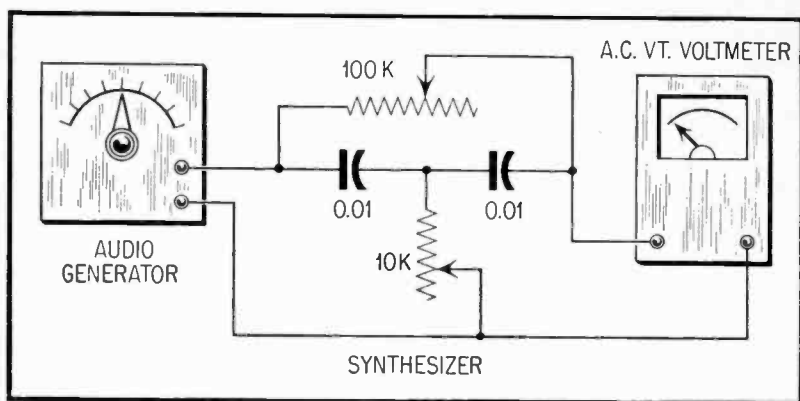
Fig. 5. Bridged-T Network set up in Figure 3.
