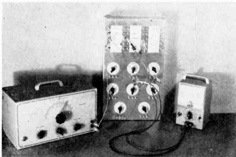
Fig. 3. Synthesizer Set Up as a Bridged-T Network, with Audio Generator and A-C VT Voltmeter Connected for Performance Checks. See Fig. 5 for Circuit.
