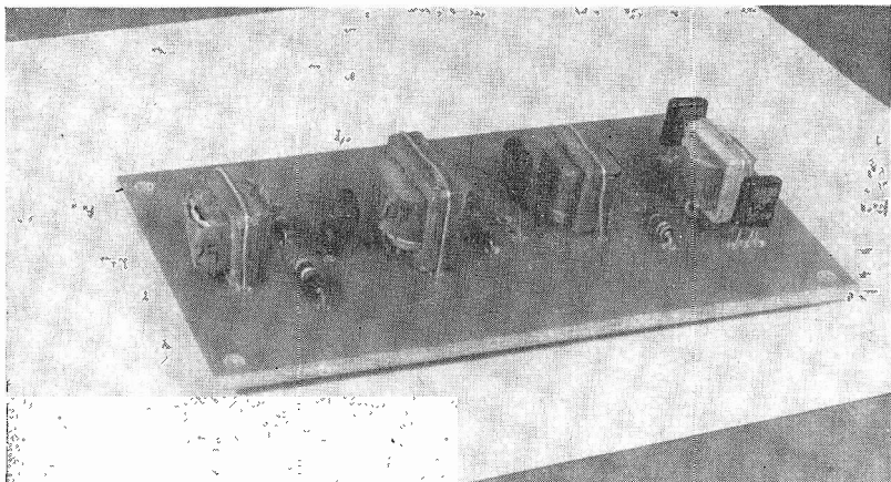
Fig. 2. Transistorized, High-Gain, High-Output Amplifier. This amplifier, built on a 6" x 3" bakelite subpanel, is the heart of the intercom. All components except coupling capacitors and switches are visible on the top of the subpanel.
