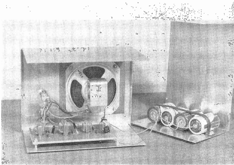
Fig. 3. Completely Assembled Intercom. The amplifier (Figure 2) is screw-mounted to the floor of the box. The ON-OFF switch and PUSH-TO-TALK switch are on the front panel (seen here to the left above the amplifier subpanel). In this photo, the 3-wire cable has not yet been connected.
