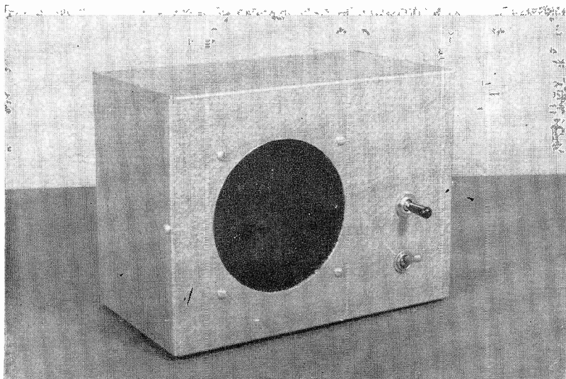
Fig. 1. The Completed, Transistorized Intercom. Entirely self-contained, this unit is built into an 8" x 6" x 4½" aluminum chassis box.
