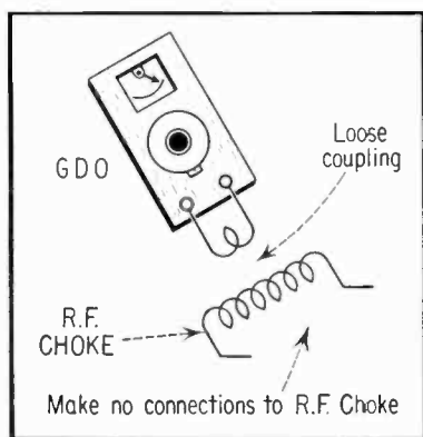
Fig. 7. Checking R-F Choke Resonant Points.
