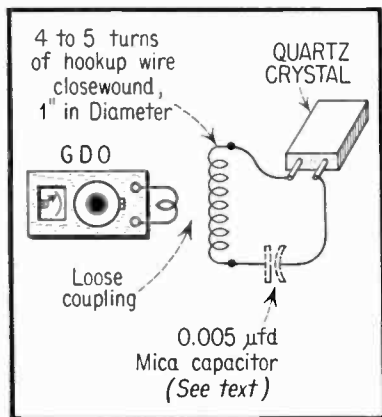
Fig. 5. Checking Crystal Frequency.
