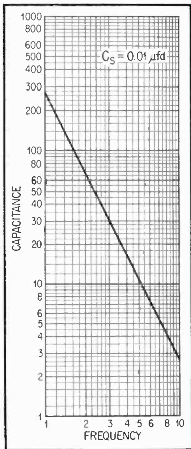
Fig. 4. Inductance Chart.
