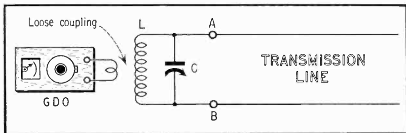
Fig. 6. Transmission Line Checking.
