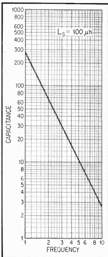
Fig. 2. Capacitance Chart.
