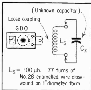
Fig. 1. Capacitance Measurement.
