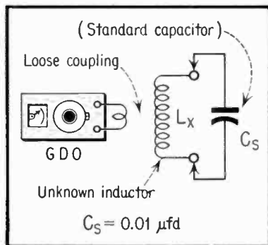
Fig. 3. Inductance Measurement.
