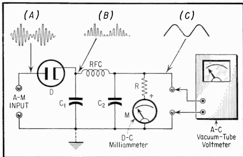
Fig. 2. Basic Circuit of Modulation Monitor.
