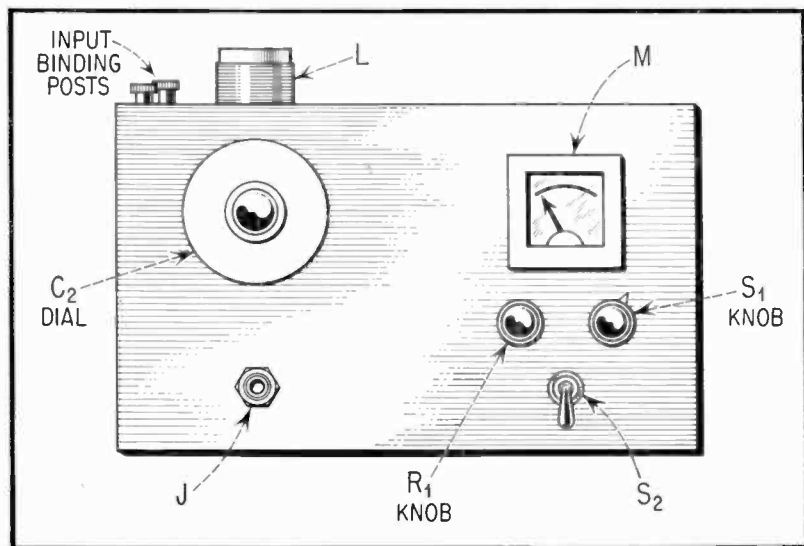
Fig. 4. Front-Panel Layout of Instrument. (Compare with Figures 1 and 3.)
