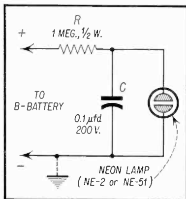
Fig. 2. Flashing Neon Pilot Light.
