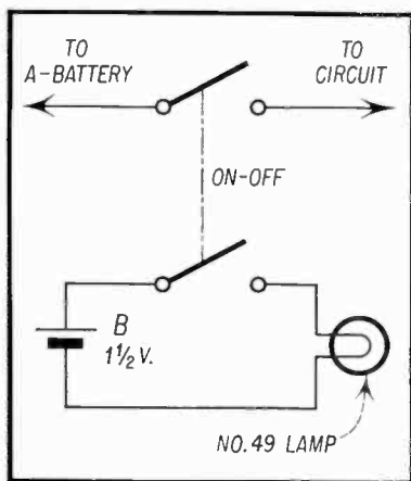
Fig. 1. Use of Pilot-Light Battery.
