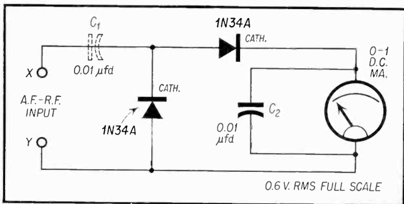
Fig. 3. AF-RF Output Meter.
