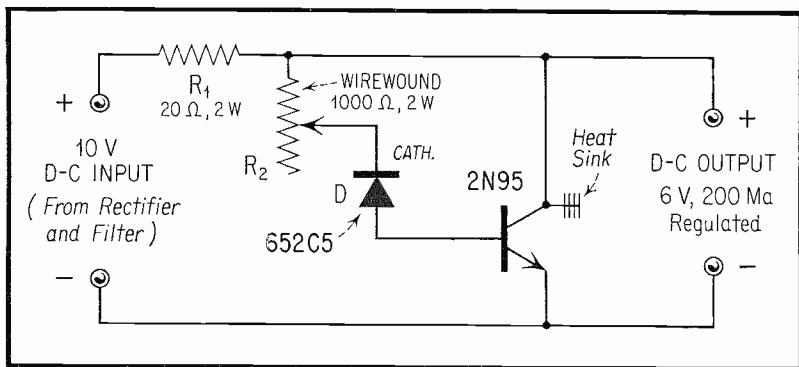
Fig. 3. Shunt Transistor-Type Voltage Regulator.
