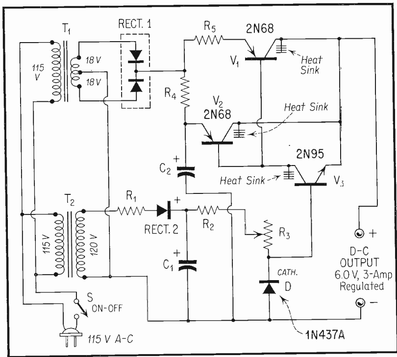
Fig. 4. Low-Voltage 3-Amp. Regulated Supply.
