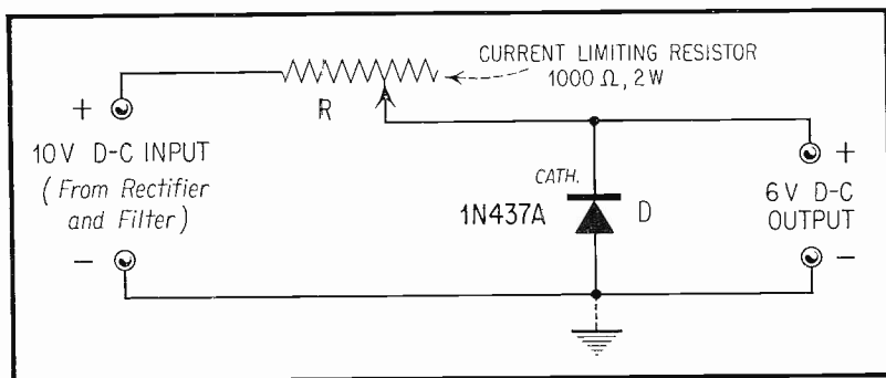
Fig. 2. Simple Diode-Type Voltage Regulator.
