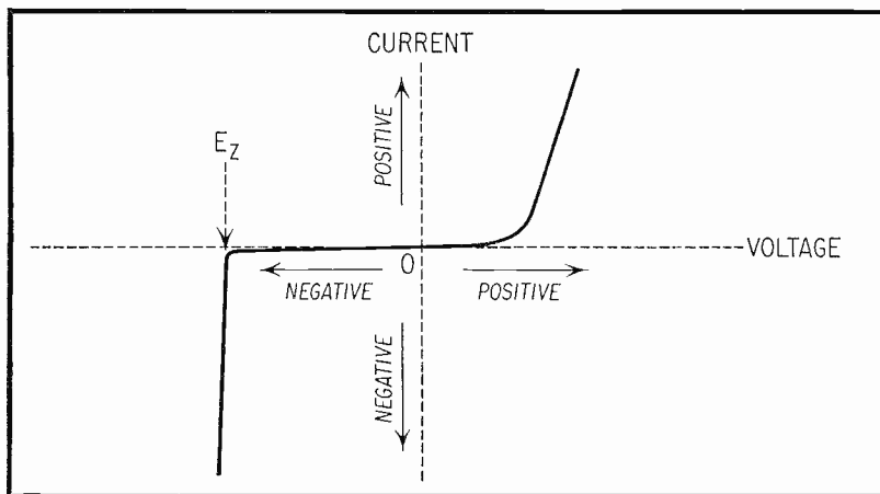
Fig. 1. Silicon Junction Diode Characteristic.
