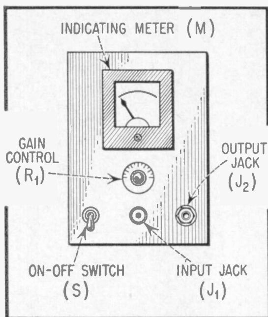
Fig. 8. Front Panel Layout.
