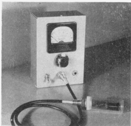
Fig. 1. Transistorized Hum Stethoscope Ready for Use. The hum probe is shown plugged into the input jack, J 1 . See Figure 8 for identification of components.
