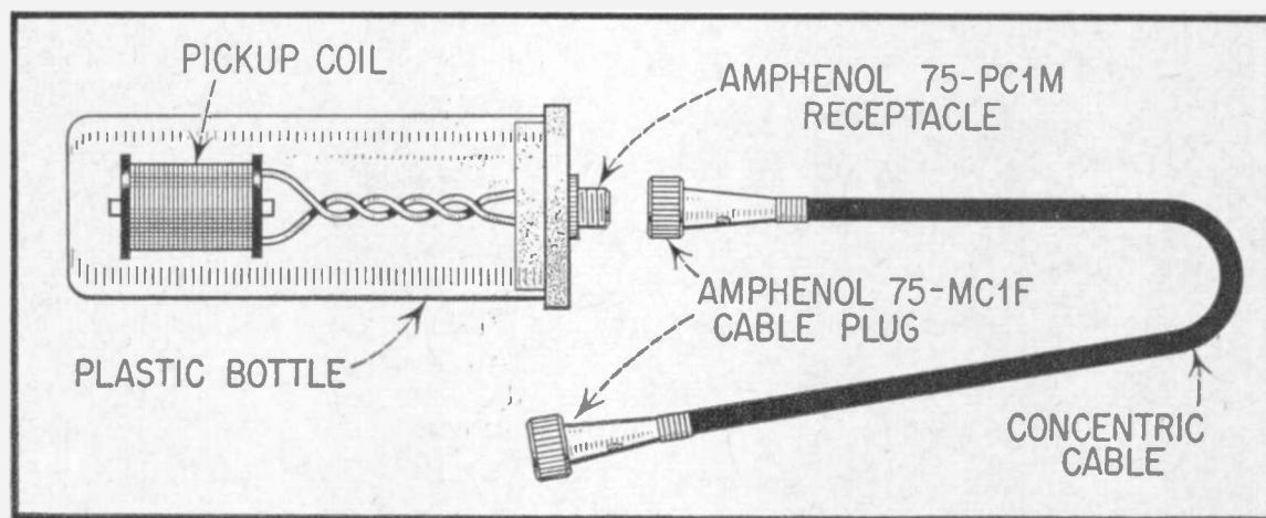
Fig. 7. Details of Hum Probe.
