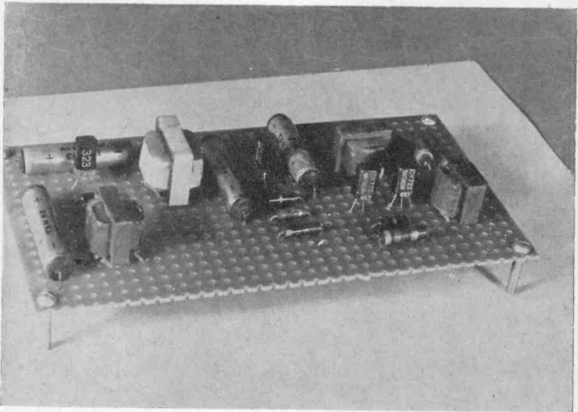
Fig. 3. Completed Circuit Board. Most of the circuit components are mounted on this 6\frac{1}{2}'' \times 3\frac{1}{2}'' perforated phenolic board. See Figure 4 for identification of components.
