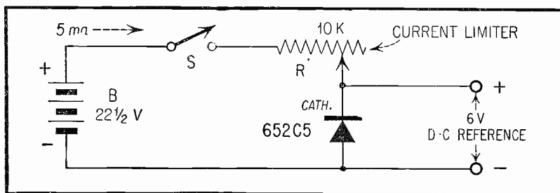
Fig. 2. D-C Voltage Reference.
