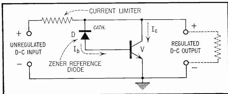
Fig. 5. Diode-Referenced, Transistorized D-C Regulator.
