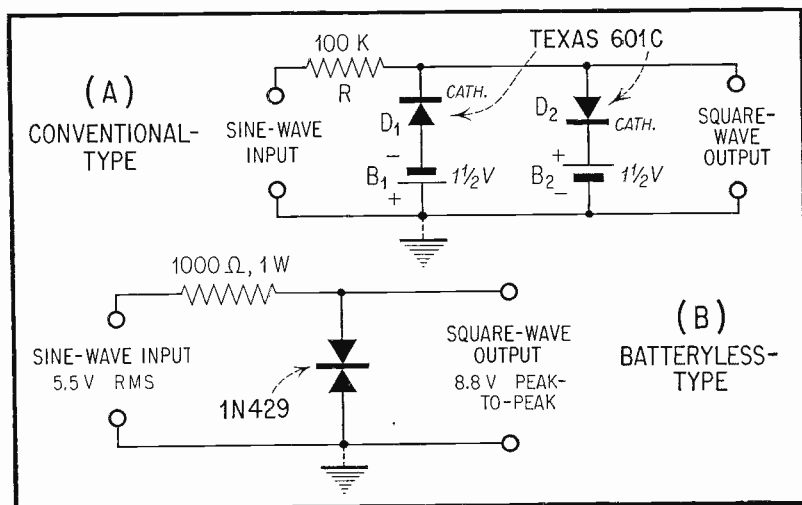
Fig. 6. Limiters (Square-Wave Converters).
