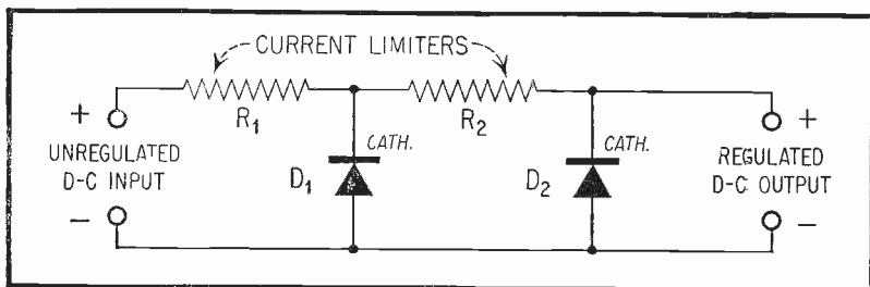
Fig. 3. 2-Stage D-C Voltage Regulator.
