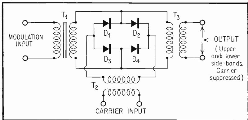
Fig. 7. Bridge Modulator.
