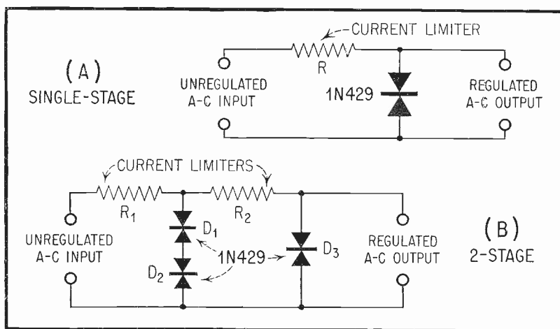
Fig. 4. A-C Voltage Regulators.
