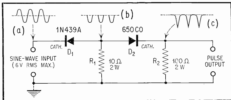
Fig. 8. Pulse Generator.
