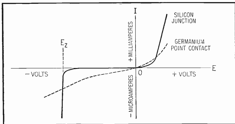
Fig. 1. Conduction Characteristic.
