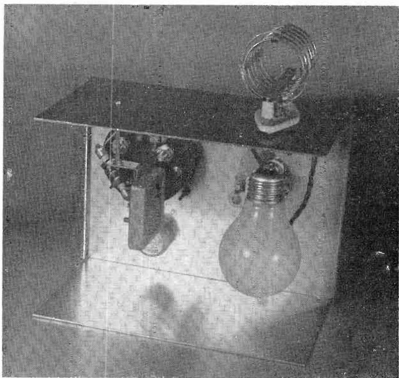
Fig. 5. Inside view of the completed instrument. The photocell is mounted on a right-angle bracket held from the top of the case by a long screw behind the meter. The 25-watt lamp is attached by means of stout pigtail leads to the tuning capacitor (C.) and coil socket.
