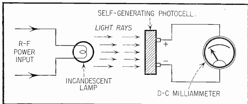
Fig. 2. Principle of Photoelectric Wattmeter.
