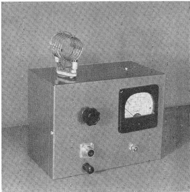
Fig. 1. Completed Photoelectric R-F Wattmeter. The instrument is built in an aluminum chassis box 8\frac{1}{4} " long, 6" high, and 4\frac{1}{2} " deep, and is link-coupled to the transmitter under test. Compare with Figure 4 for identification of components.
