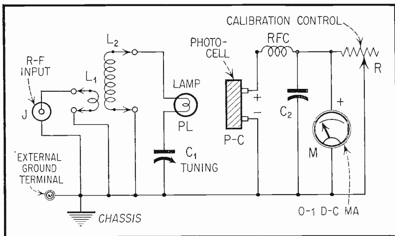
Fig. 3. Complete Circuit of Wattmeter.
