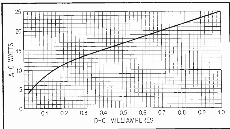
Fig. 7. Typical Instrument Calibration.
