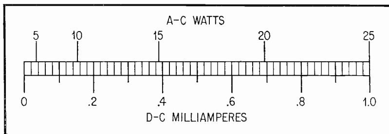
Fig. 8. Comparison of Current and Power Scales on Meter.
