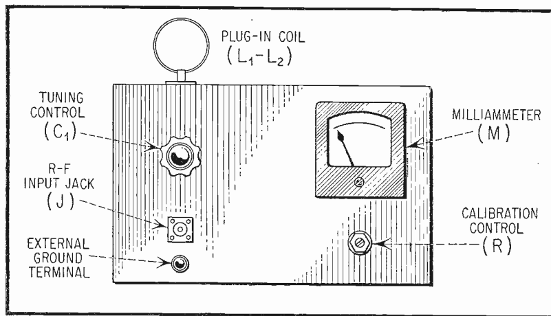
Fig. 4. Front-Panel Layout.
