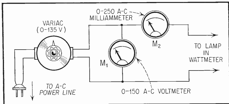
Fig. 6. Calibration Circuit.
