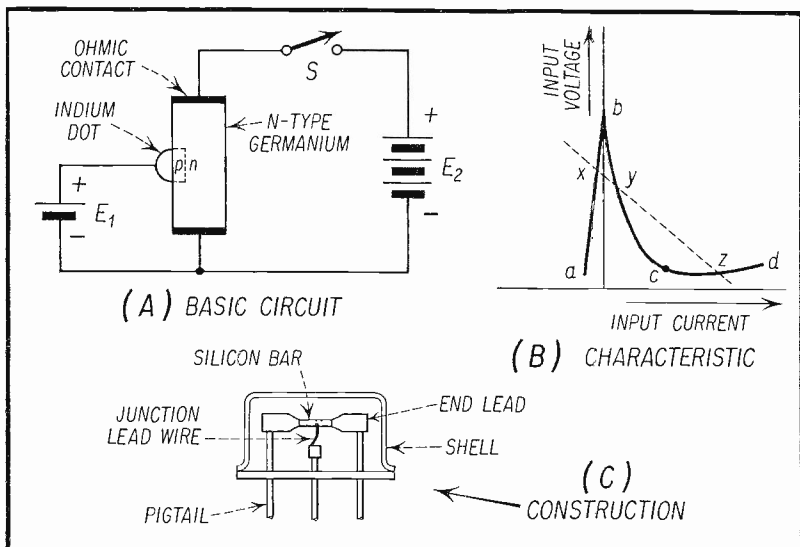
Fig. 3. Unijunction Transistor.
