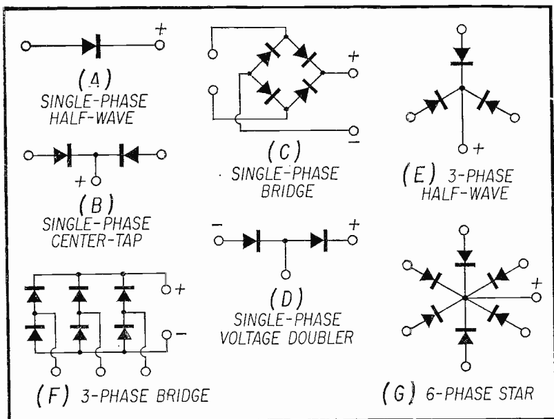
Fig. 1. Stack Configurations of Silicon Rectifiers.
