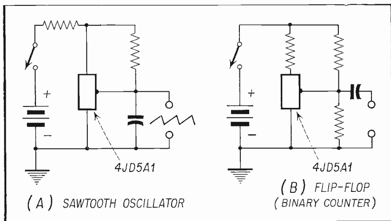
Fig. 4. Unijunction Transistor Circuits.
