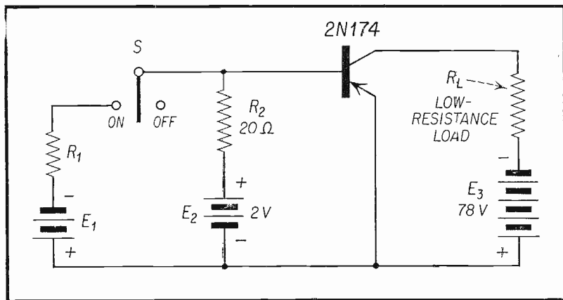
Fig. 2. One-Kilowatt Transistor Switch.
