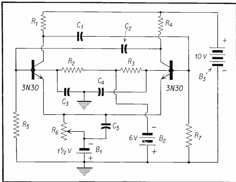
Fig. 6. Tetrode Multivibrator.
