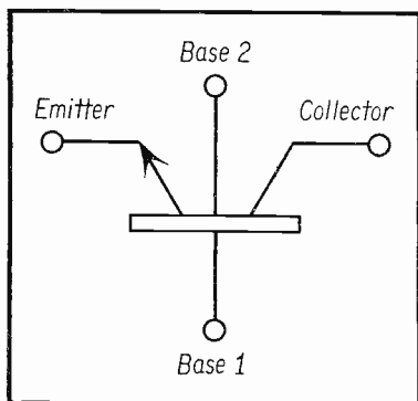
Fig. 5. Tetrode Transistor.
