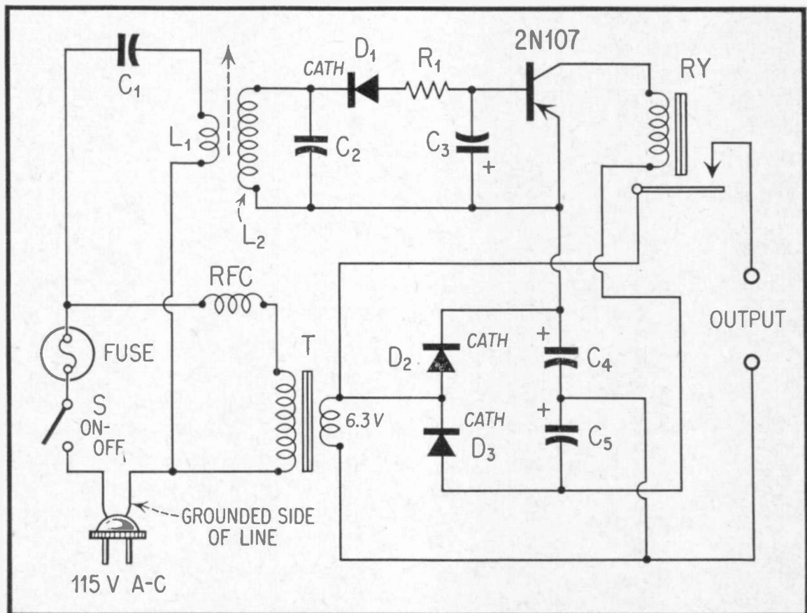
Fig. 4. Diode-Transistor-Type Wired-Radio Receiver.
