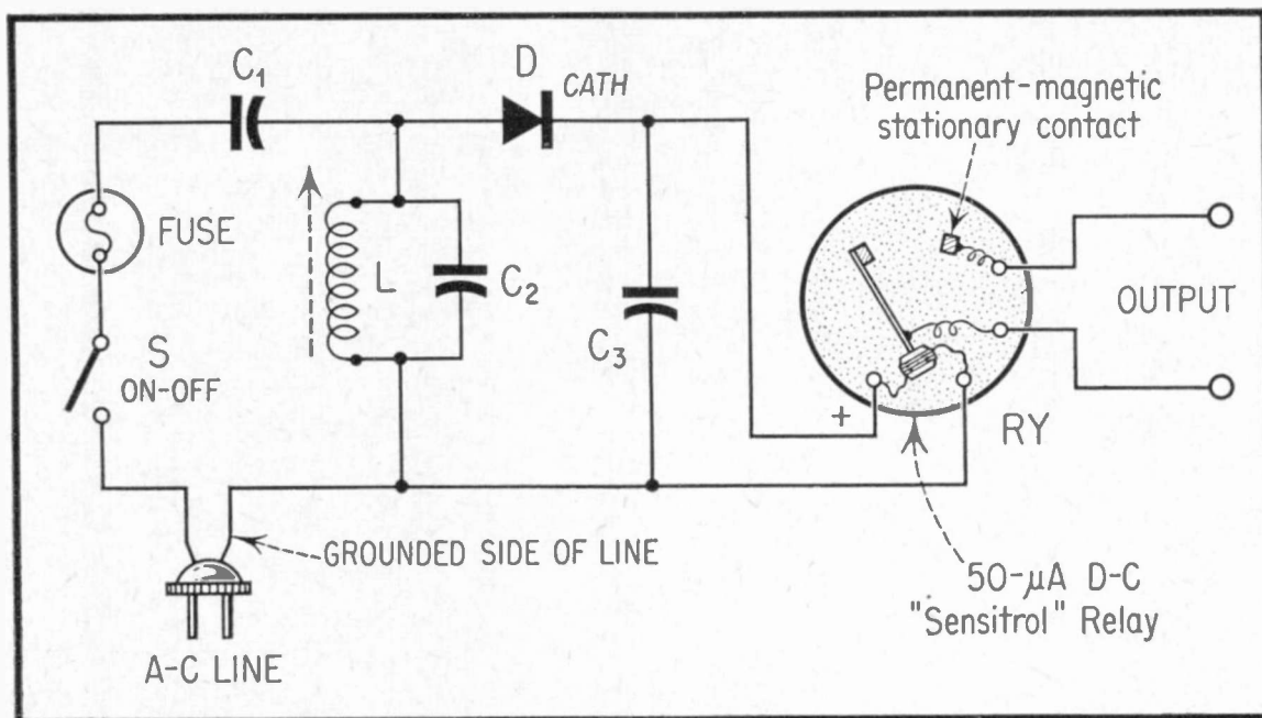
Fig. 3. Diode-Type Wired-Radio Receiver.
