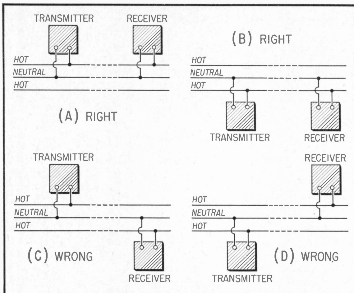
Fig. 5. Connections To 3-Wire Service.
