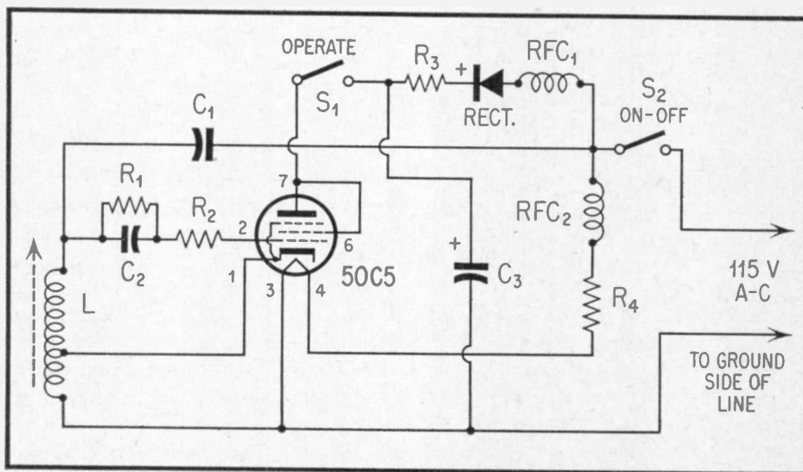
Fig. 2. Transformerless Wired-Radio Transmitter.
