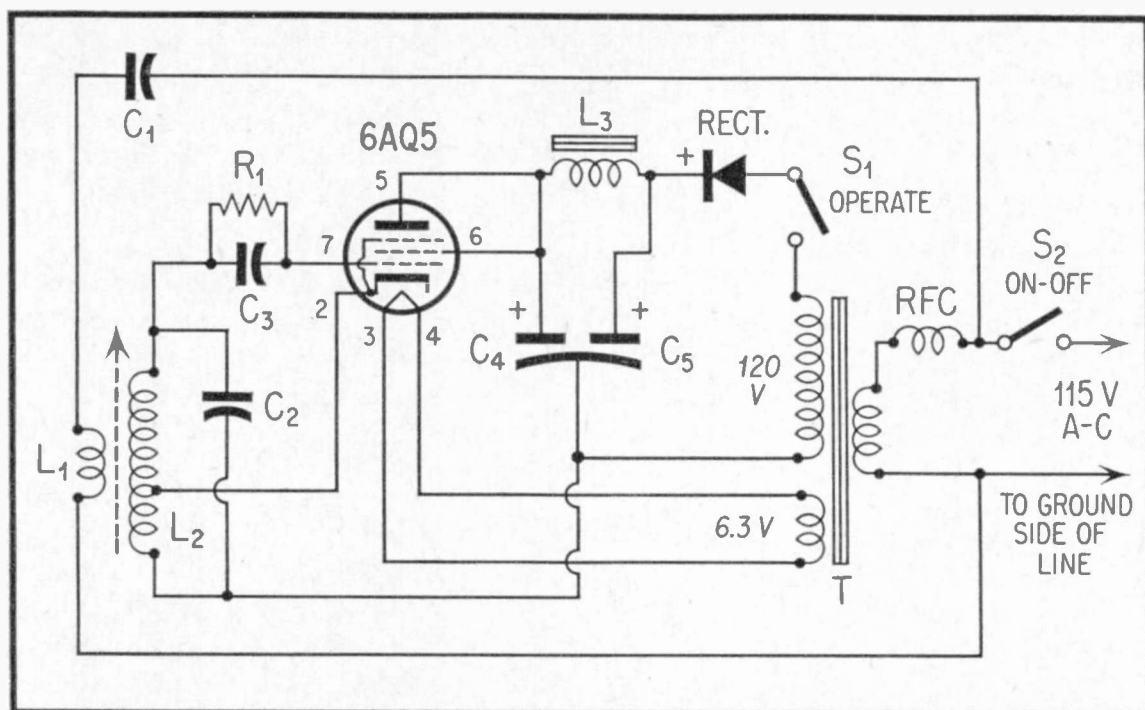
Fig. 1. Transformer-Coupled Wired-Radio Transmitter.
