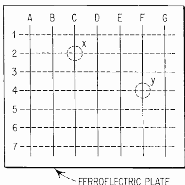
Fig. 5. Arrangement of Ferroelectric Memory.
