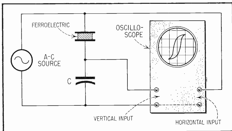
Fig. 3. Setup for Checking Ferroelectric Hysteresis.
