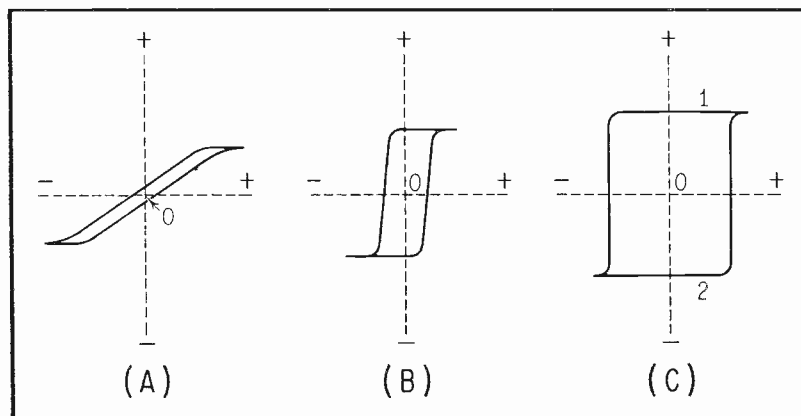
Fig. 4. Ferroelectric Hysteresis Loops.
