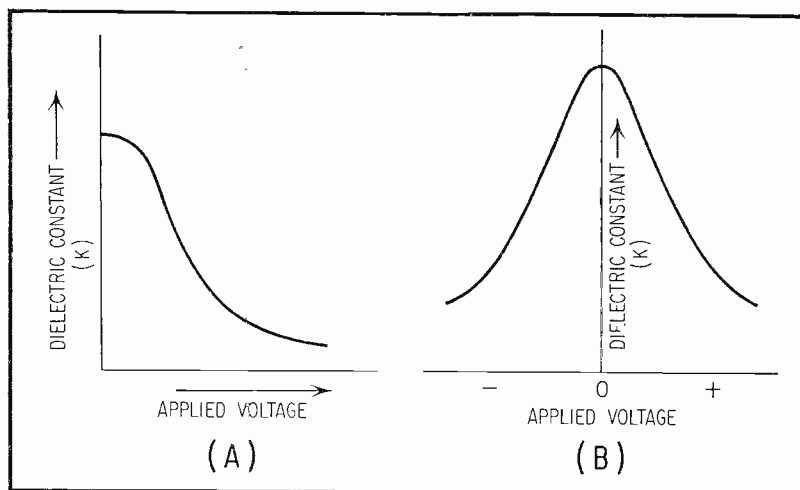
Fig. 1. Variation of Dielectric Constant with Applied Voltage.
