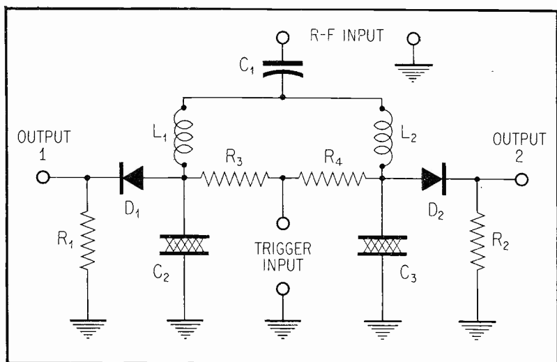
Fig. 6. Ferroresonant Circuit Employing Ferroelectric Capacitors.
