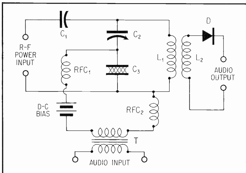
Fig. 7. Dielectric Amplifier.
