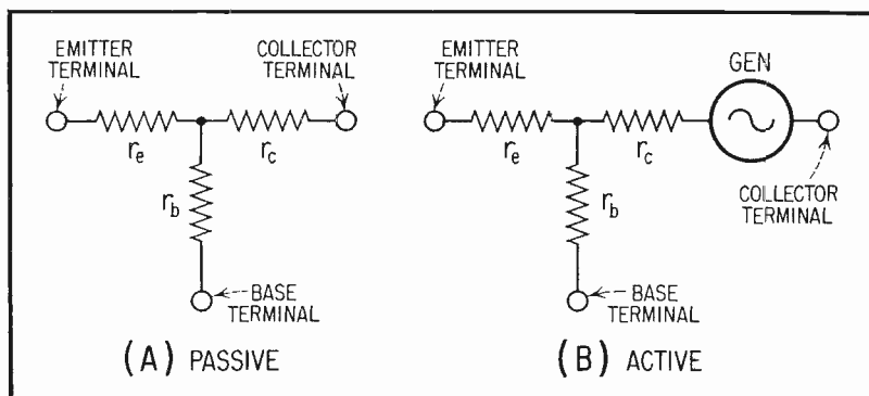
Fig. 1. Equivalent T-Networks of Transistor.
