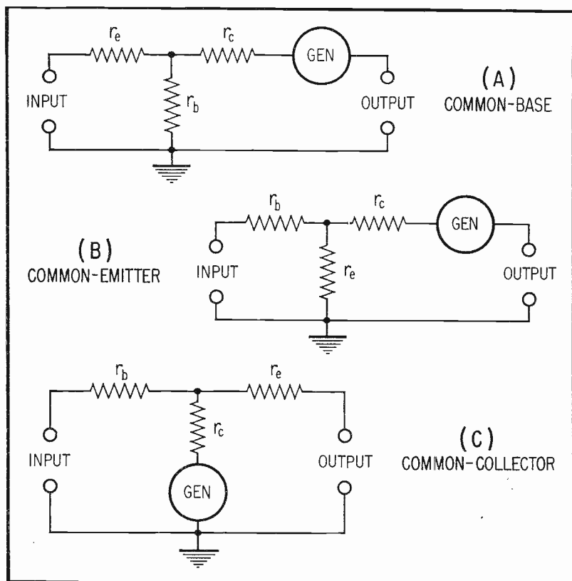
Fig. 2. Equivalent T-Networks of Amplifying Transistors.
