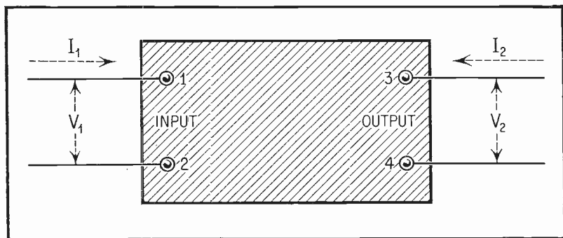
Fig. 3. Equivalent Black Box of Transistor.
