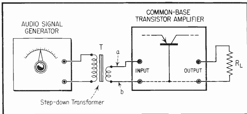
Fig. 1. Use of Impedance-Matching Generator Transformer.
