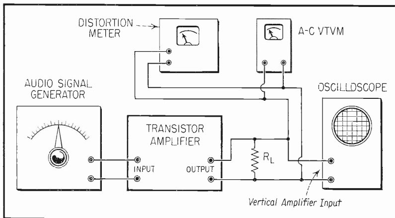
Fig. 5. Test Setup for Distortion Measurement.
