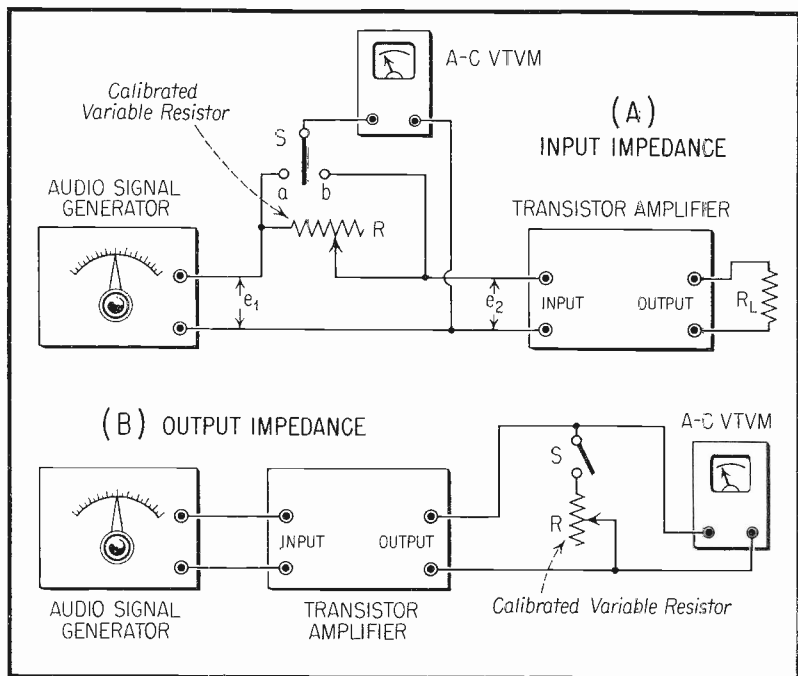
Fig. 4. Test Setups for Impedance Measurements.
