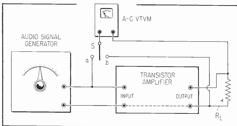
Fig. 2. Test Setup for Frequency Response and Voltage Gain.
