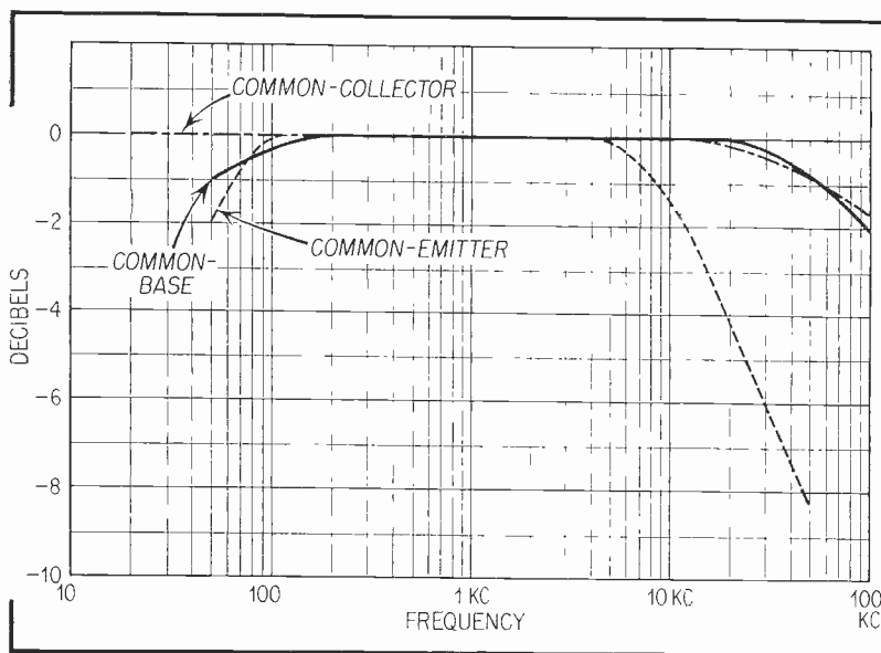
Fig. 3. Comparative Frequency Response of Uncompensated Transistor Amplifiers.
