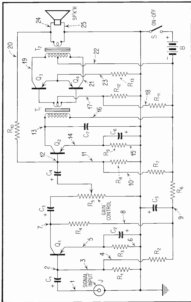
Fig. 7. Typical Transistor Amplifier.
