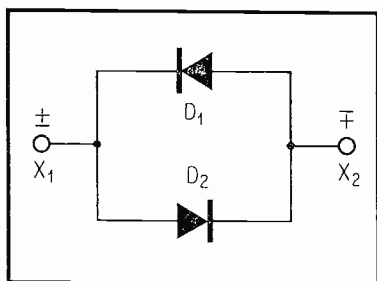
Fig. 4. Dual-Diode Non-Linear Resistor.
