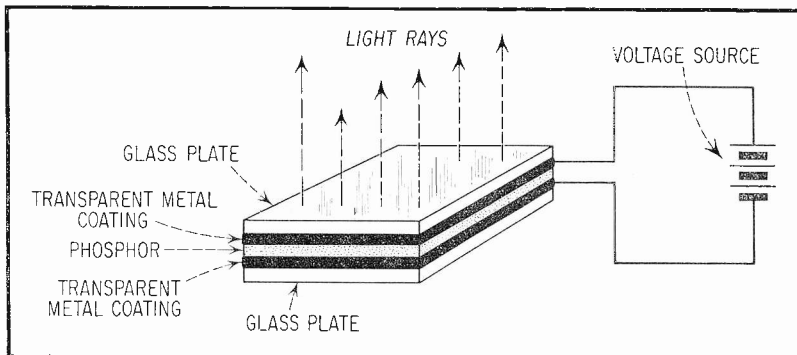
Fig. 9. Electroluminescent Cell.
