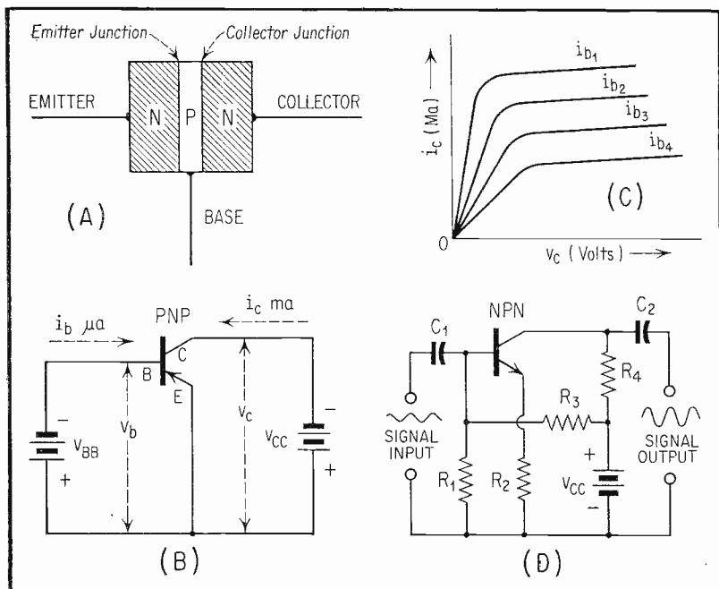
Fig. 2. Transistor Characteristics.
