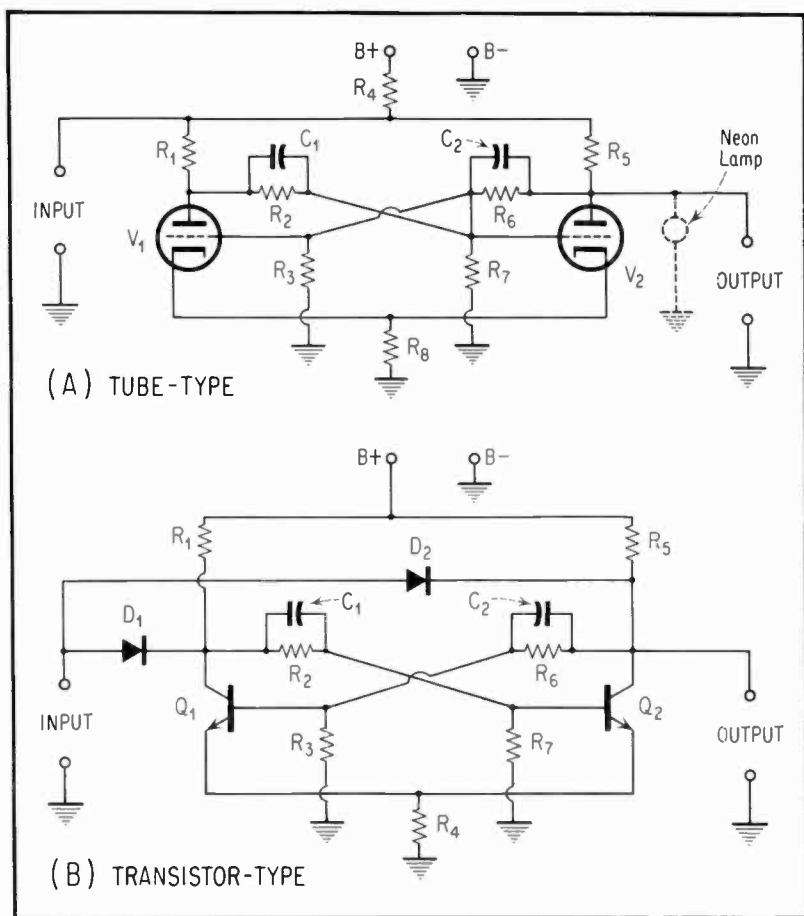
Fig. 1. Basic Flip-Flops.
