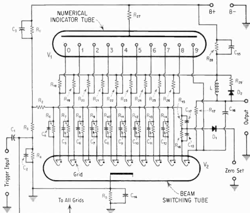
Fig. 6. Beam-Switching Counter Decade.
