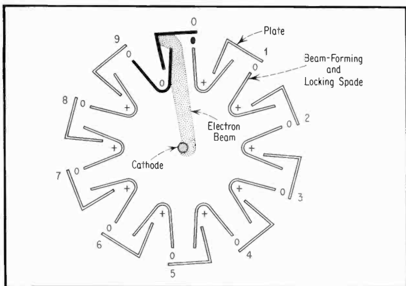
Fig. 5. Details of Beam Switching Tube.
