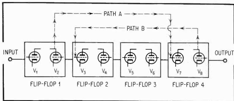
Fig. 2. Arrangement of Decimal Scaler.
