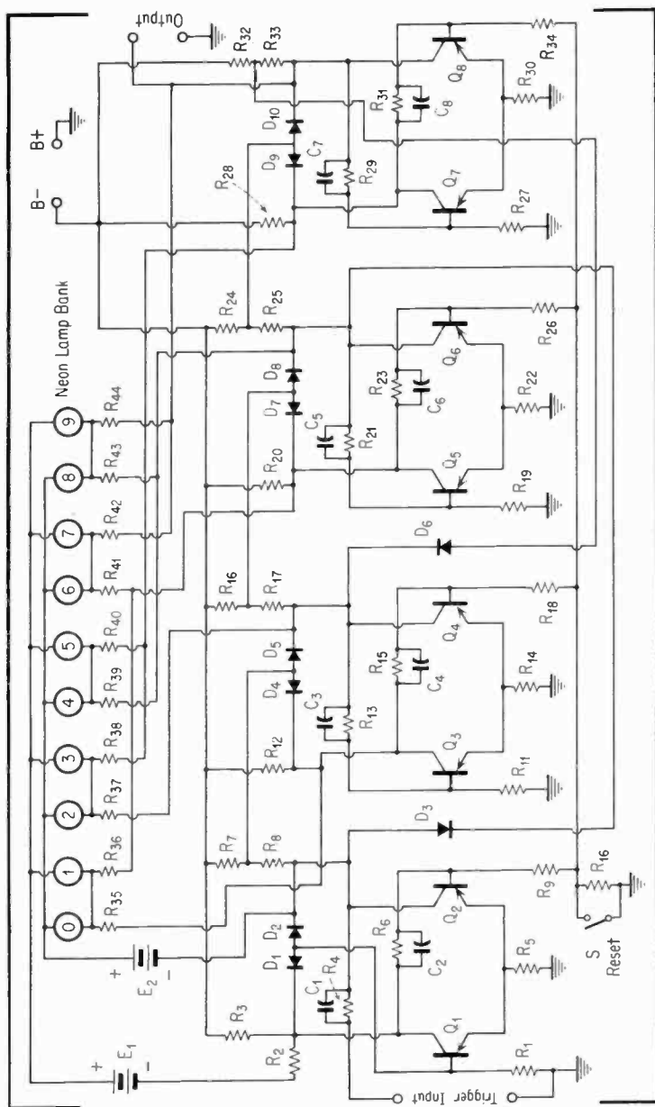
Fig. 4. Transistorized Decimal Scaler.
