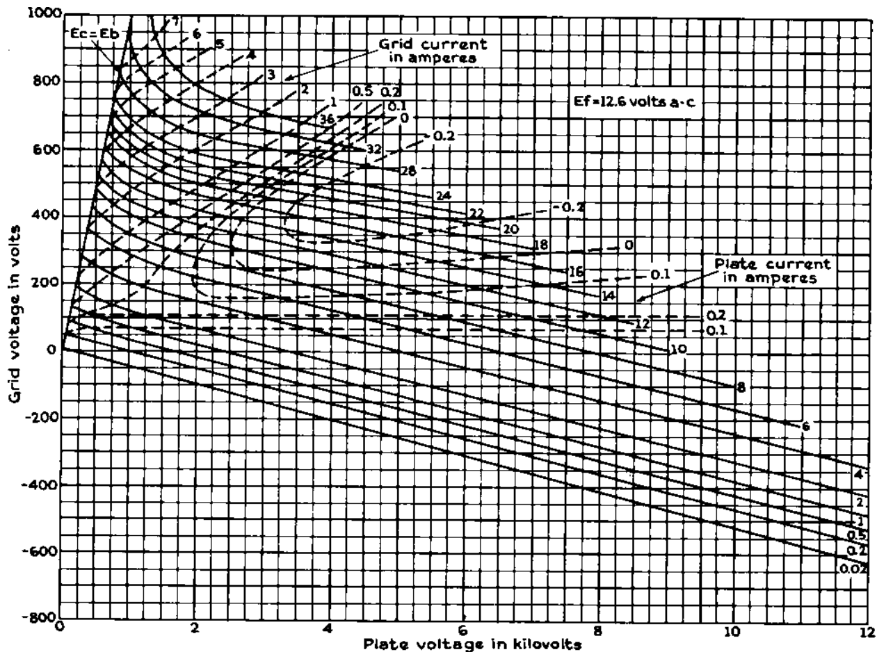
Characteristic Curve K-7050613 9-1-38
