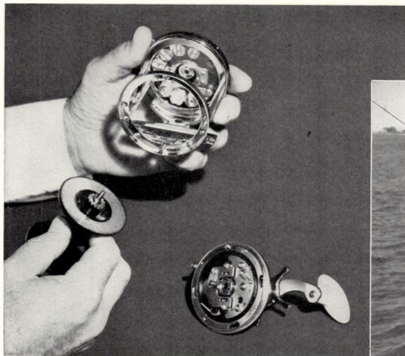
Alnico magnets in the reel (left hand) and a copper disk in the spool (right hand) are the working parts of the magnetically braked reel. The ends are made of G-E plastics.
