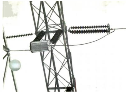
Figure 8. Very elaborate coupling capacitor (right) and frequency trap (above) is required for power lines. Cost may exceed that of a high capacity microwave terminal, particularly on very high voltage lines.
