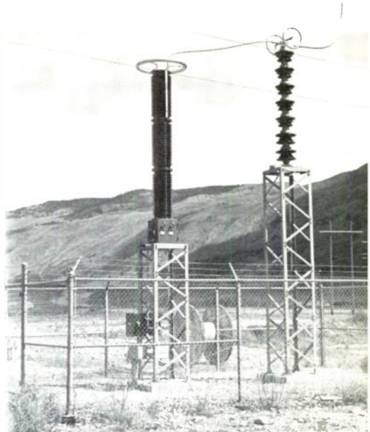
Figure 8. Very elaborate coupling capacitor (right) and frequency trap (above) is required for power lines. Cost may exceed that of a high capacity microwave terminal, particularly on very high voltage lines.
