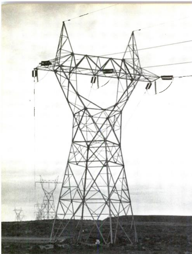
Figure 1. High-voltage transmission lines sweep across country, bringing cheaper power for industry and home use than could be possible in most locations if power had to be produced near the consumer. Like most long lines, these carry power at a potential of 230,000 volts in order to lower transmission losses due to high current flow.
