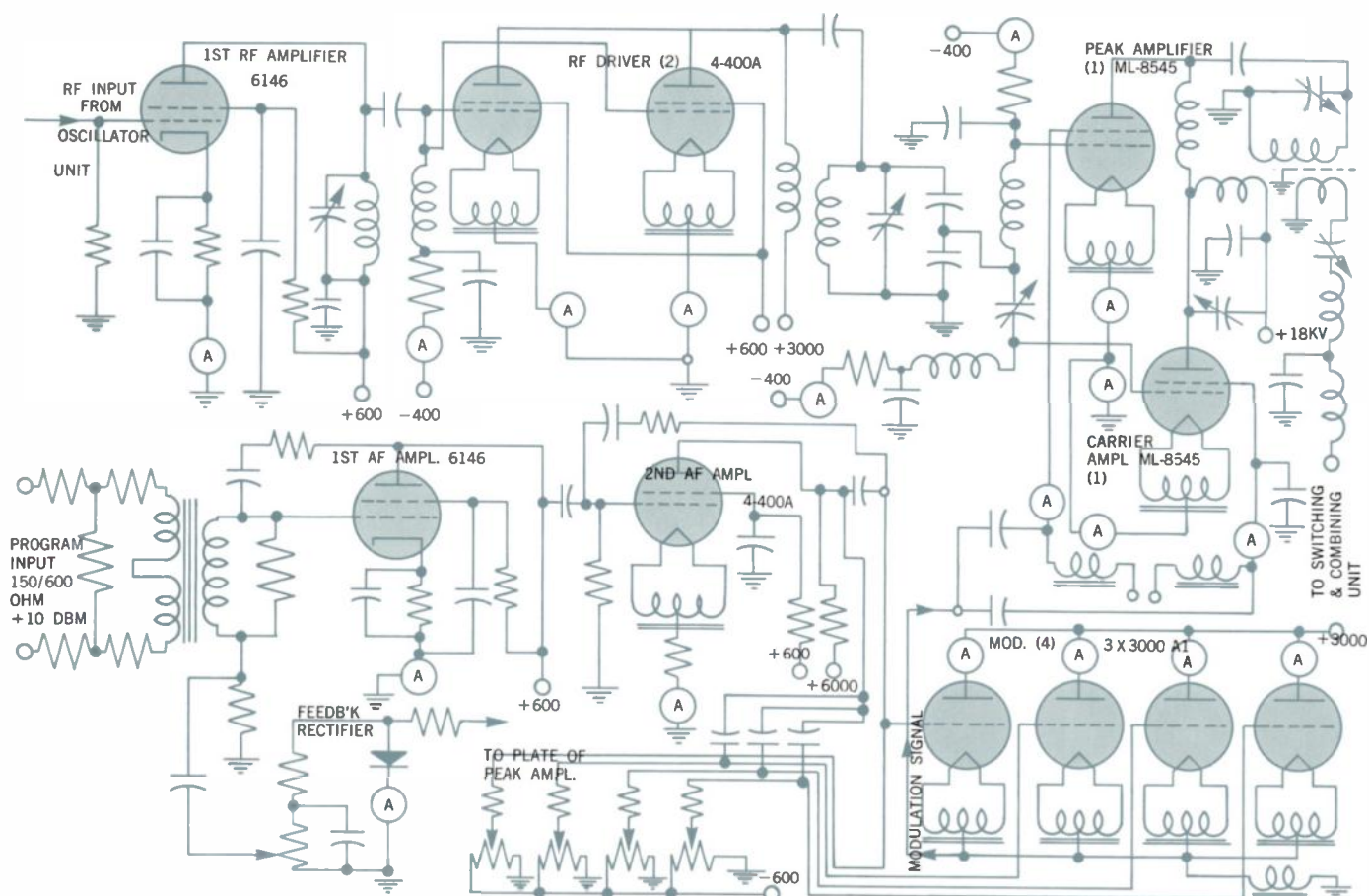
Figure 2 — Simplified Schematic 250 kW MF Broadcast Transmitter.
