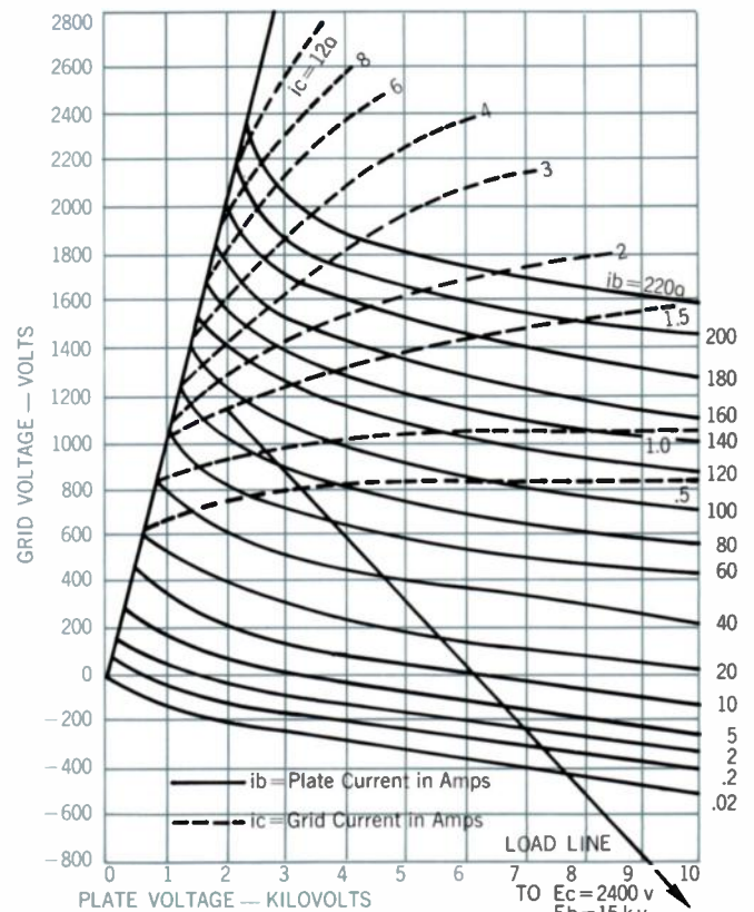
Figure 7 — Constant Current Characteristics for the ML-8618.
