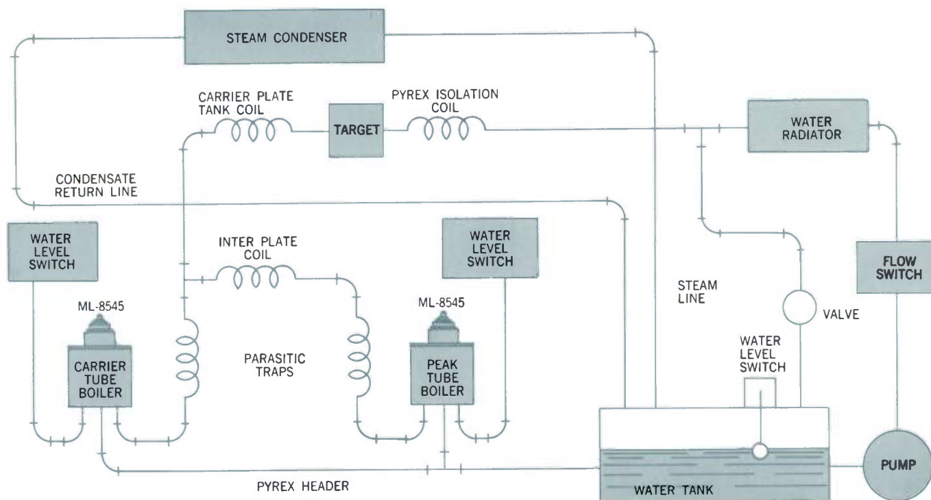
Figure 3 — Vapor Cooling System for 250 kW MF Broadcast Transmitter.
