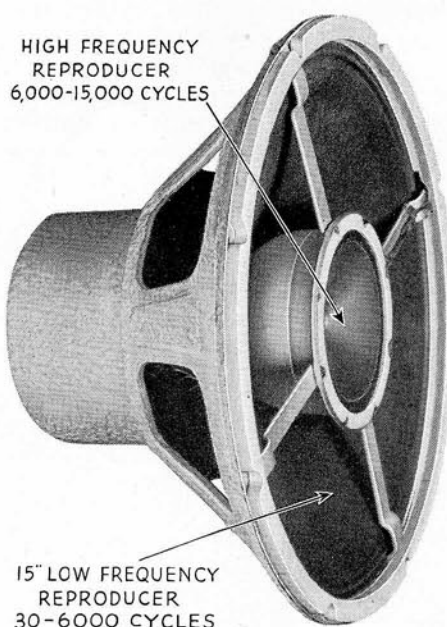
The New Three Unit Co-Axial High Fidelity Speaker—with 15" Low Frequency combined with High Frequency Reproducer (dividing network not shown)
