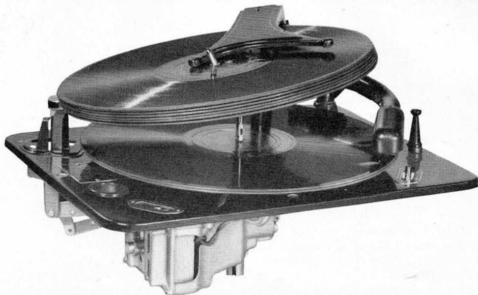
THE GARRARD PRECISION BUILT AUTOMATIC RECORD CHANGER
