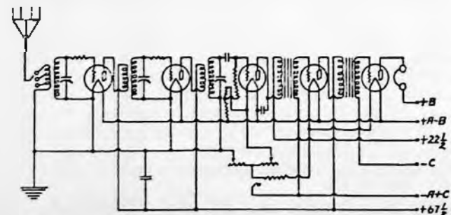
FIG. 18. SCHEMATIC WIRING DIAGRAM OF MODEL 20 COMPACT SET.
