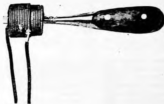
FIG. 22. MAGNETIZING A SCREW DRIVER.
