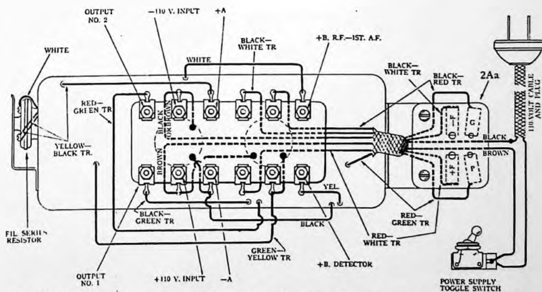
FIG. 102. SHOWING CONNECTIONS AND APPROXIMATE POSITION OF LEADS FROM SEALED CONTAINER IN 3RD TYPE OF POWER UNIT.
