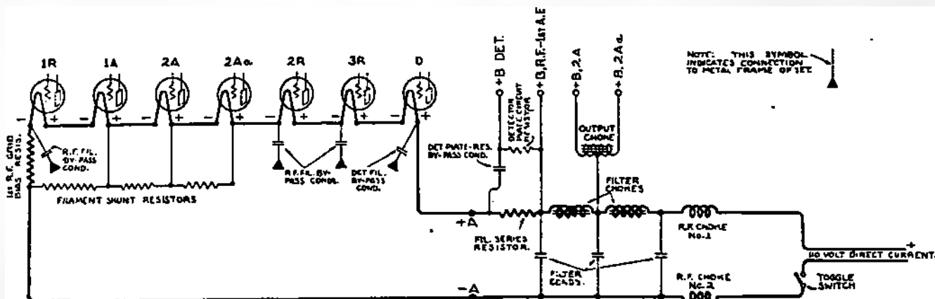
FIG. 86. SIMPLIFIED DIAGRAM OF POWER UNIT AND FILAMENT CIRCUIT IN MODEL 41 RECEIVER.
