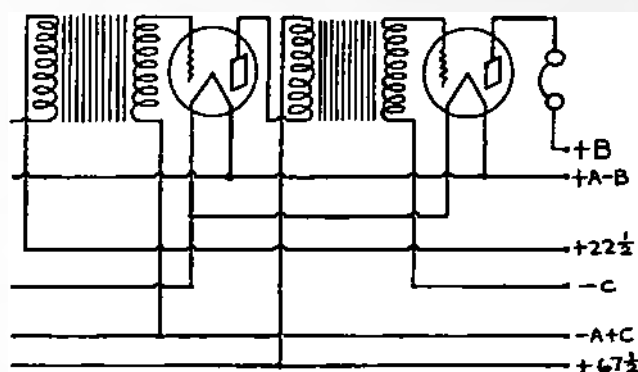
FIG. 16. AUDIO FREQUENCY CIRCUIT.
