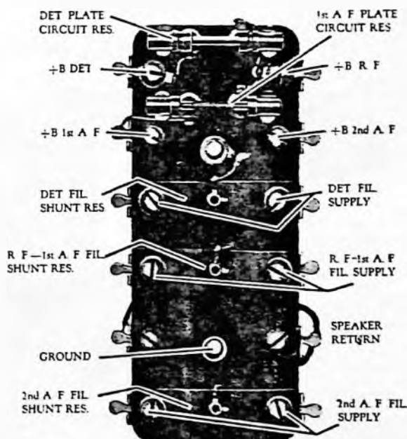
FIG. 76. BOTTOM VIEW OF PANEL ASSEMBLY USED IN POWER UNIT OF MODELS 40, 42, 44 AND 52
