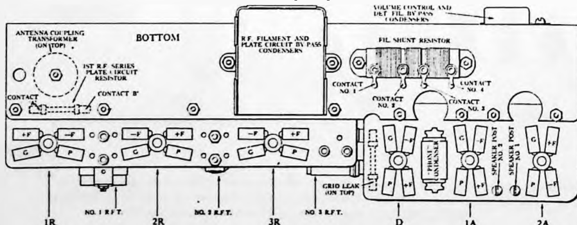
FIG. 99. TESTING CHART FOR MODEL 41.
