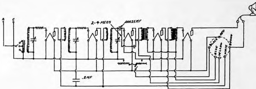
FIG. 36. MODEL 20 COMPACT SET No. 7570. WIRING DIAGRAM.
