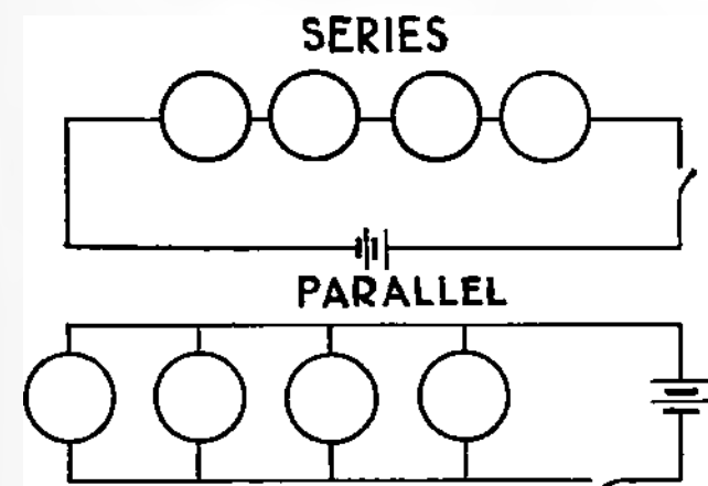
FIG. 17. THE TWO FUNDAMENTAL METHODS OF CONNECTING SEVERAL ELECTRICAL UNITS TOGETHER.
