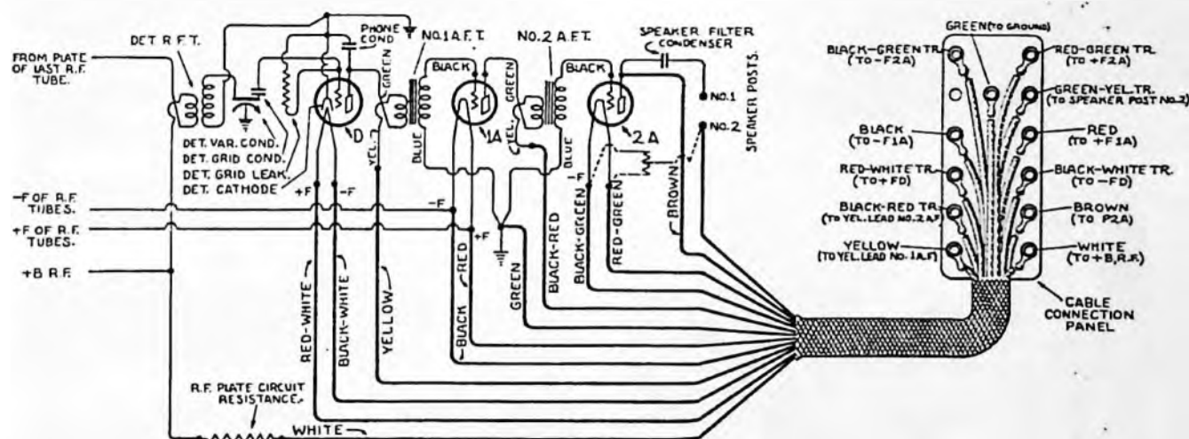
FIG. 78. DETECTOR AND TWO STAGE AUDIO FREQUENCY AMPLIFYING CIRCUIT USED IN LATER MODEL 36, AND IN MODELS 37, 38, 40, 42, 44 AND 53
