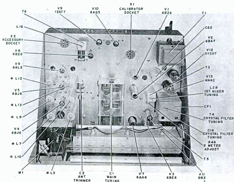
Figure 6. Component Locations, Top View of Receiver
