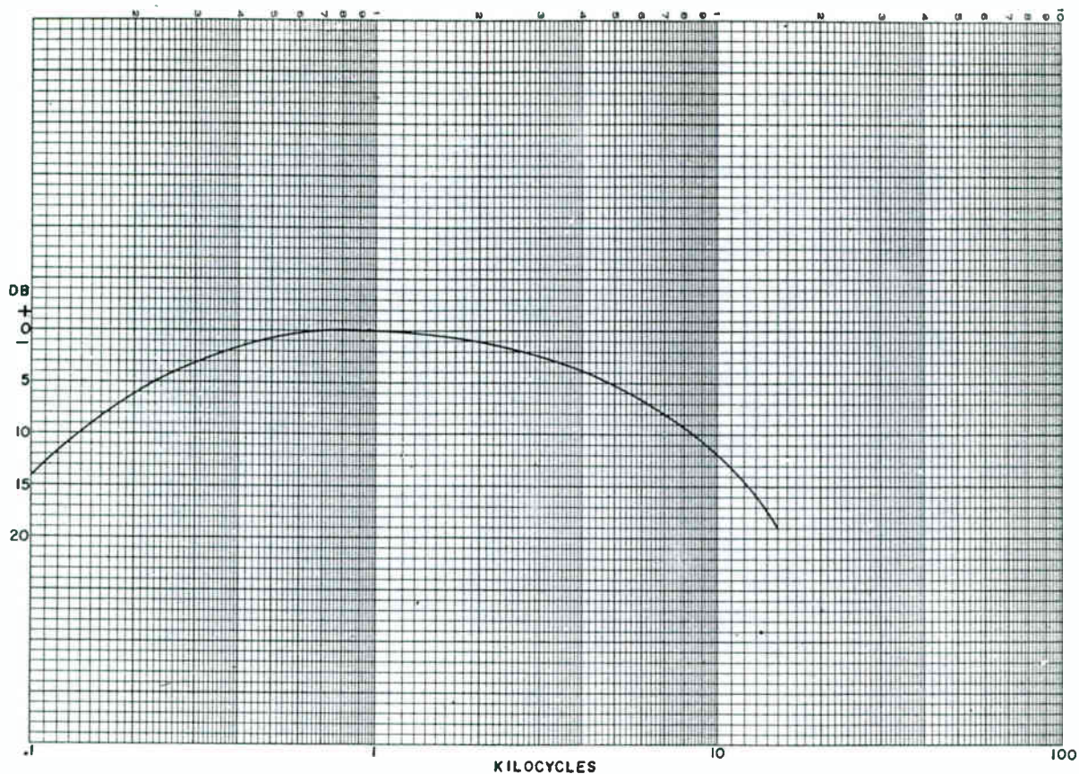
Figure 4. Audio Response
