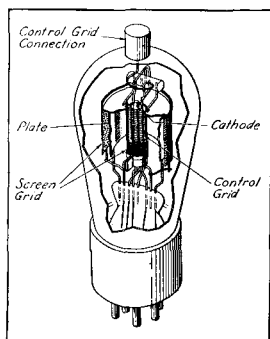
Interior View of '24-A
