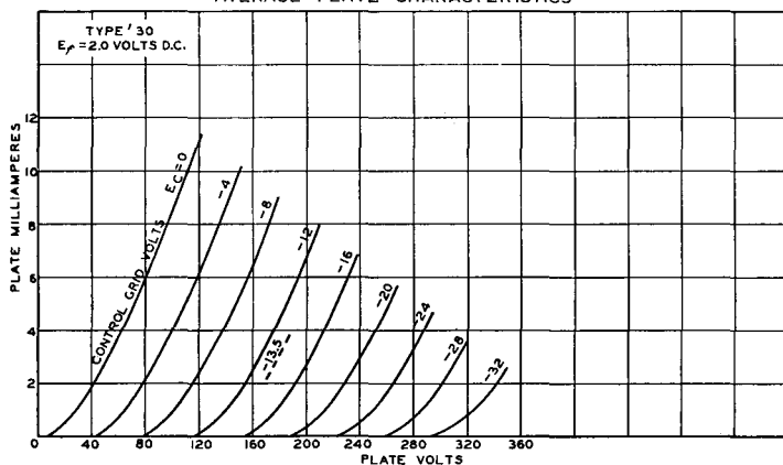
AVERAGE CHARACTERISTICS
