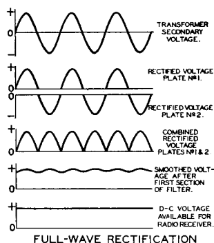
FULL-WAVE RECTIFICATION
