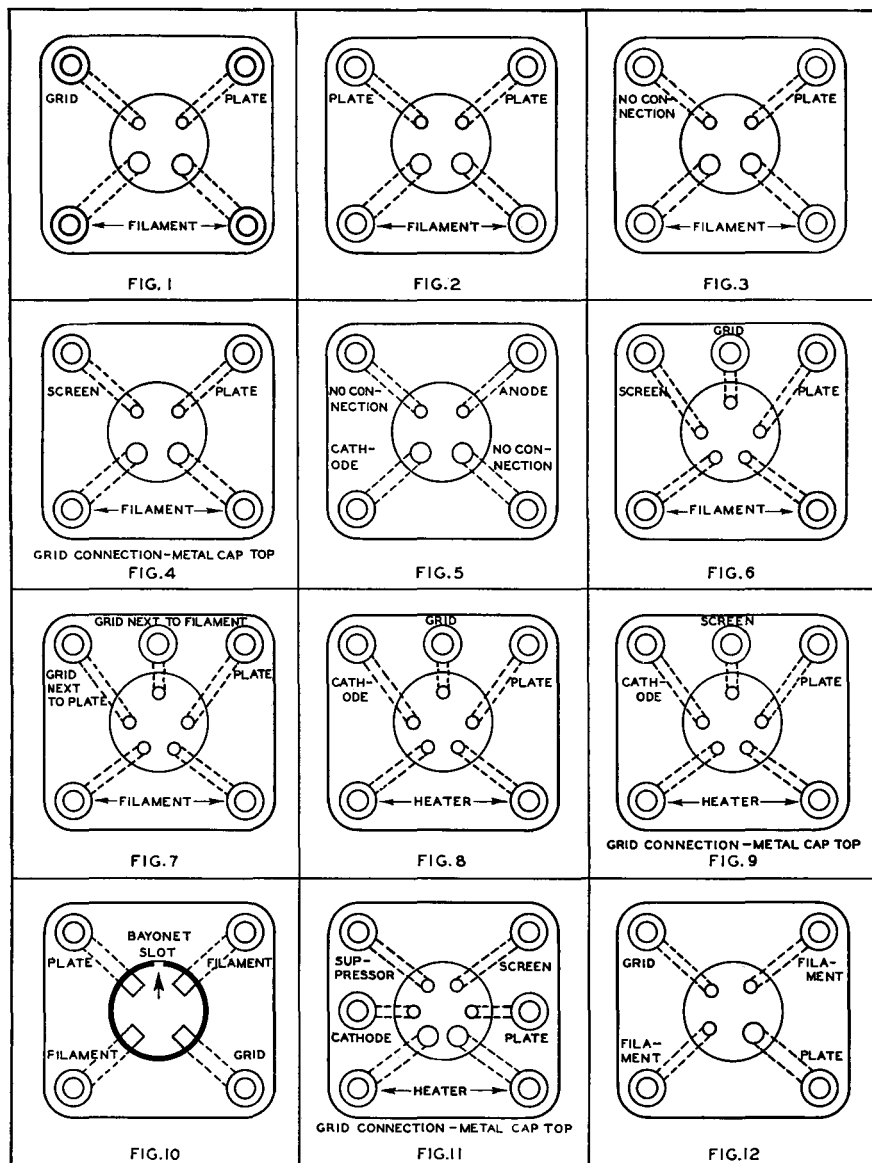
TOP VIEWS OF SOCKETS
