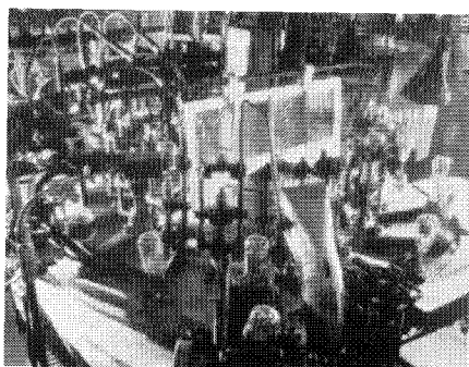
Bulb Sealing and Exhausting
