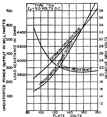
AVERAGE CHARACTERISTICS
