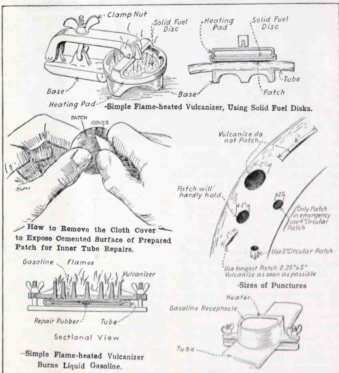
Fig. 6—Methods of patching inner tubes and size of patch to use for various sized breaks in tube
