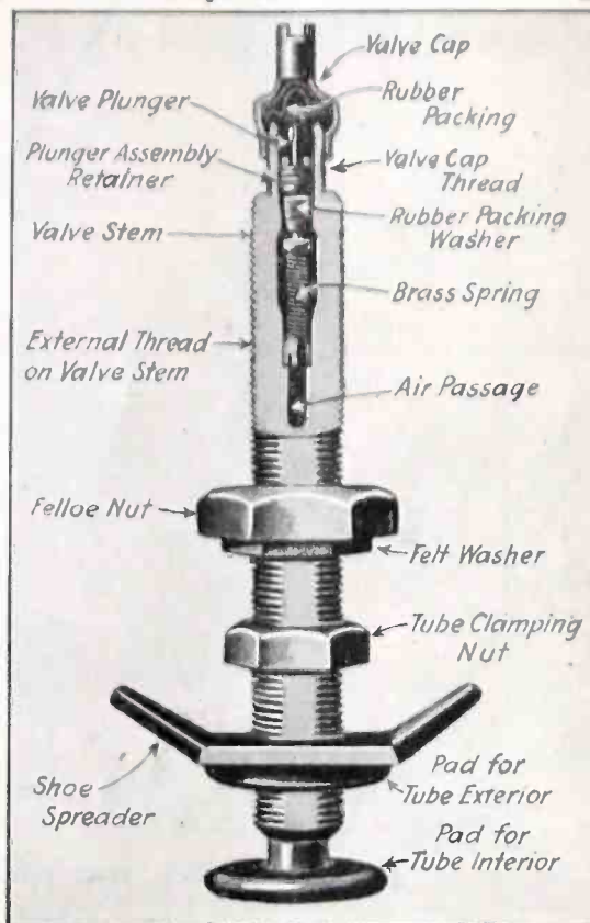
Fig. 1—Construction of Schrader universal valve
