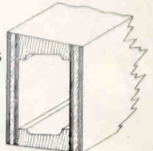
FIG. G HOLLOW SPAR Multi-Ply Sides
