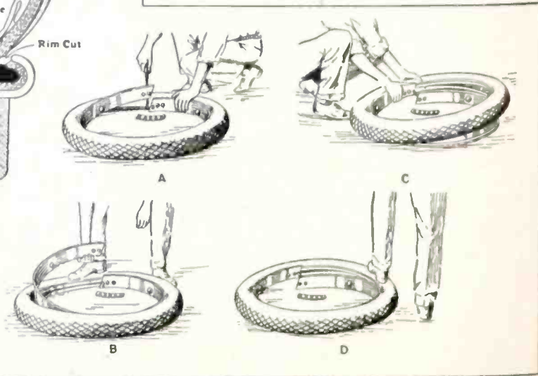
Fig. 4—Demountable split rims make the removal and application of tire casings easier and facilitate tube repairs
