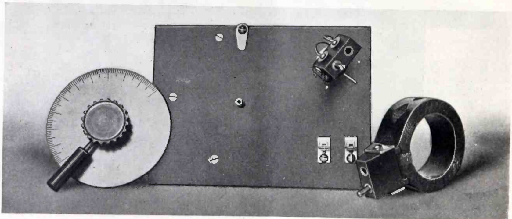
Fig. 2. Showing the mounting for the honeycomb coil and the indicating dial with its auxiliary handle
