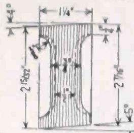
FIG. 1A TOP WING FRONT BEAM 2 Ash-12 1/2" Long-Rand L.
