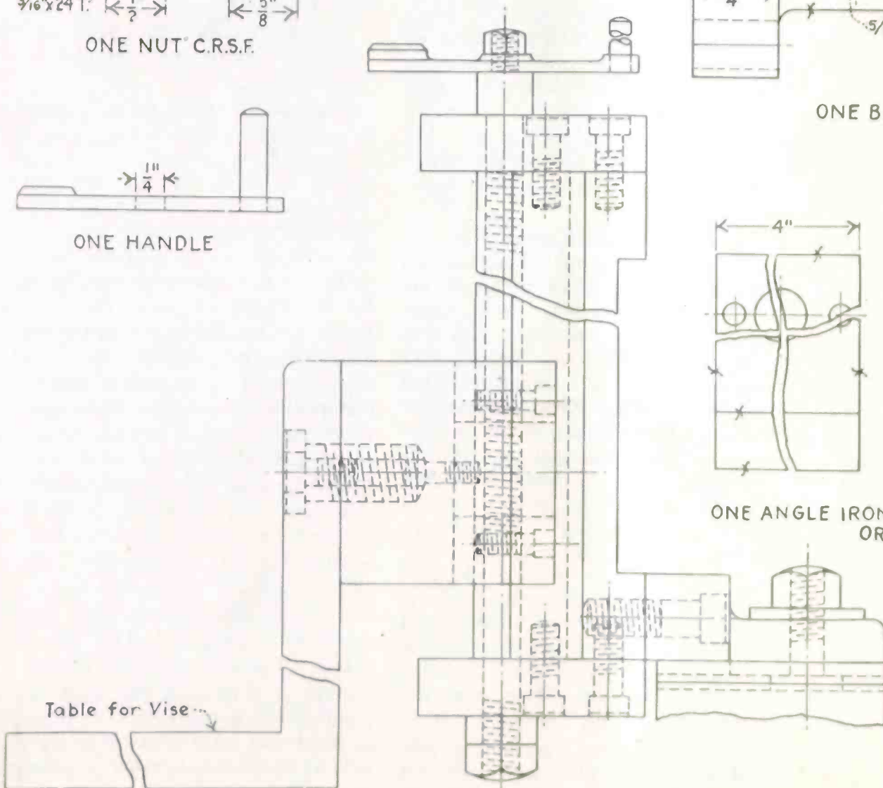
LATHE CROSS SLIDE
