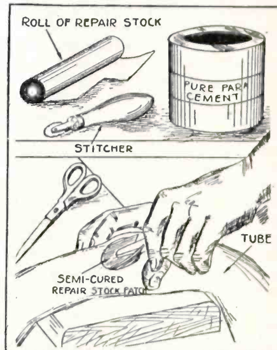
Fig. 8—Inserting semi-cured repair stock patch, curved face down. When in place, uncured stock is placed in hole and stitcher used to roll in place
