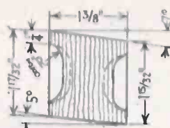
FIG. 2A TOP WING REAR BEAM 2 Ash-12 1/2" Long-Rand L.
