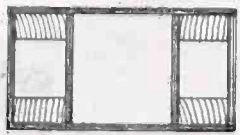
FIG. J TWIN BOX SPAR FOR LARGE WINGS
