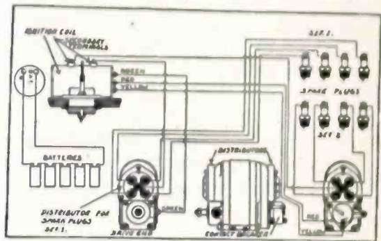
Fig. 4. Double distributor magneto for two-spark ignition
