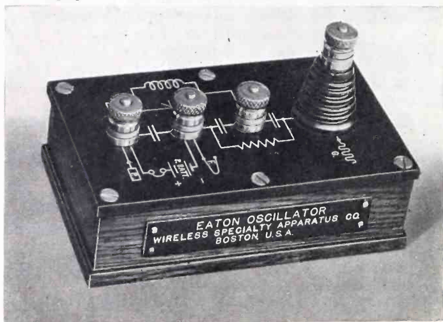
Fig. 1. A new instrument for undamped wave reception or generation of oscillation
