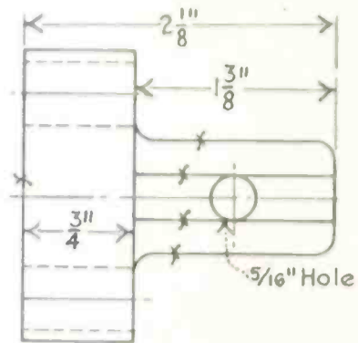
ONE BRACKET C.I.F.
