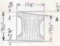
FIG. 4A LOWER WING REAR BEAM 2 Ash-9 1/2" Long-Rand L.
