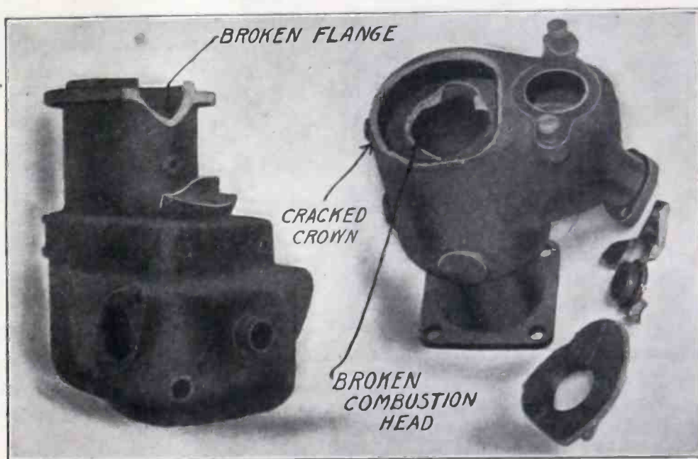
Fig. 1. Examples of defective cylinders that were repaired by autogenous process. The cylinder flange at the left was repaired at a cost of $7.50 while the cracked crown and water jacket at the right were restored at a cost of $12.00, both being a material saving over the purchase price of new replacement units
