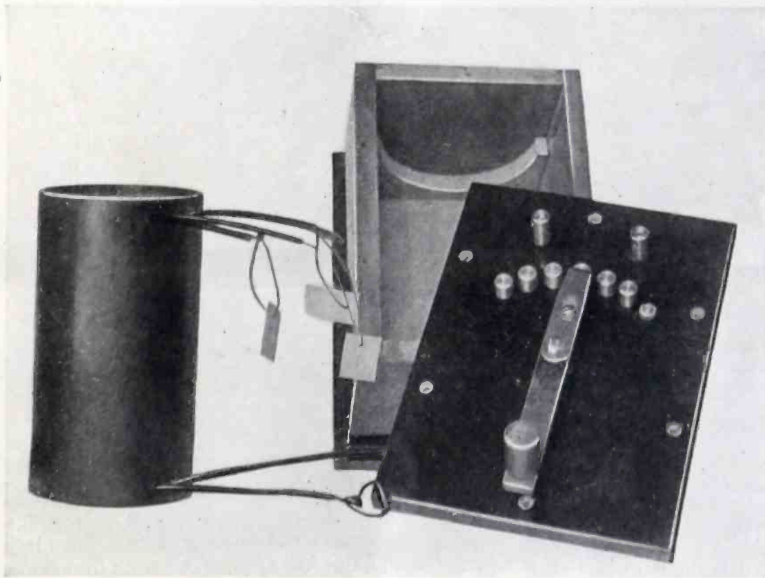
Above: The reactance coil assembled and ready for use. Below: The coil and the box it is mounted in
