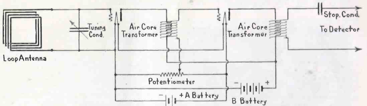
Fig. 35. A radio frequency amplifier using air core transformers between the tubes. Signals are made audible by a detector connected to the last step
