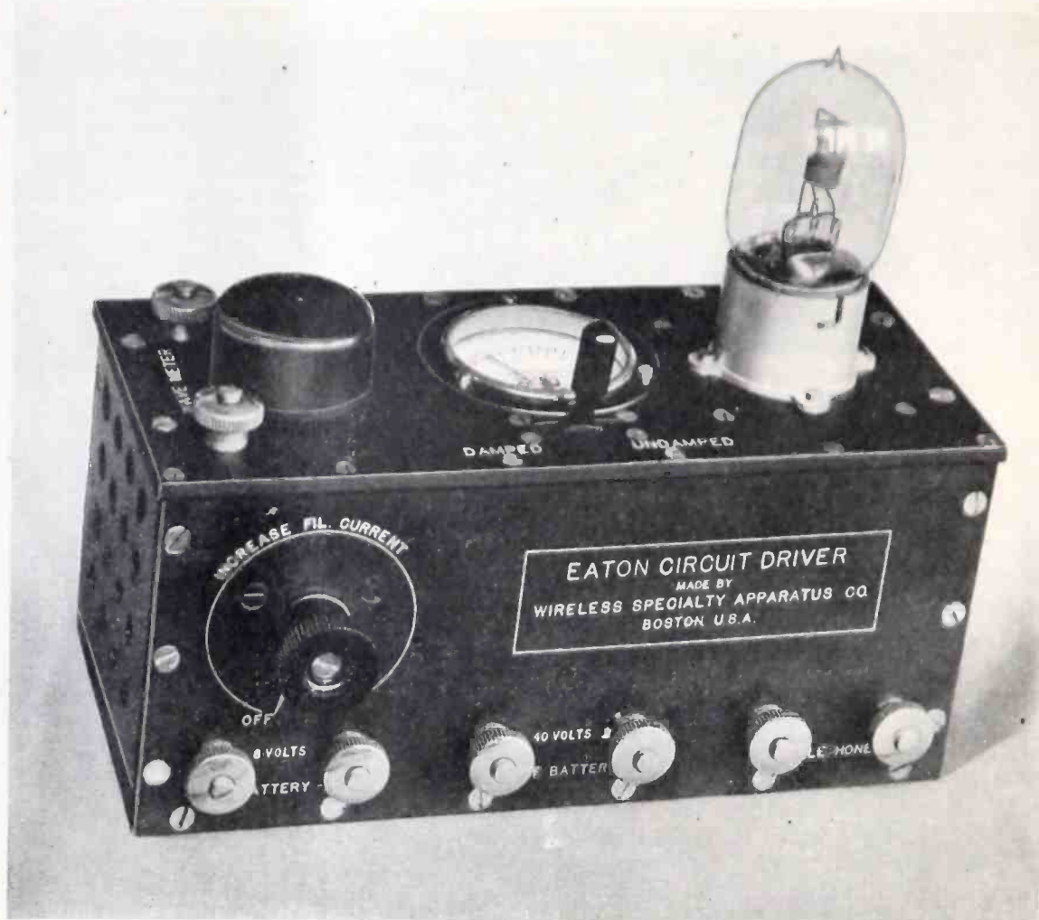
Fig. 3. A more complete set for undamped wave work
