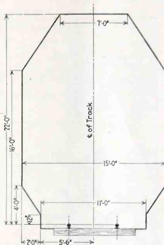
Bridge and tunnel clearance of standard practice
