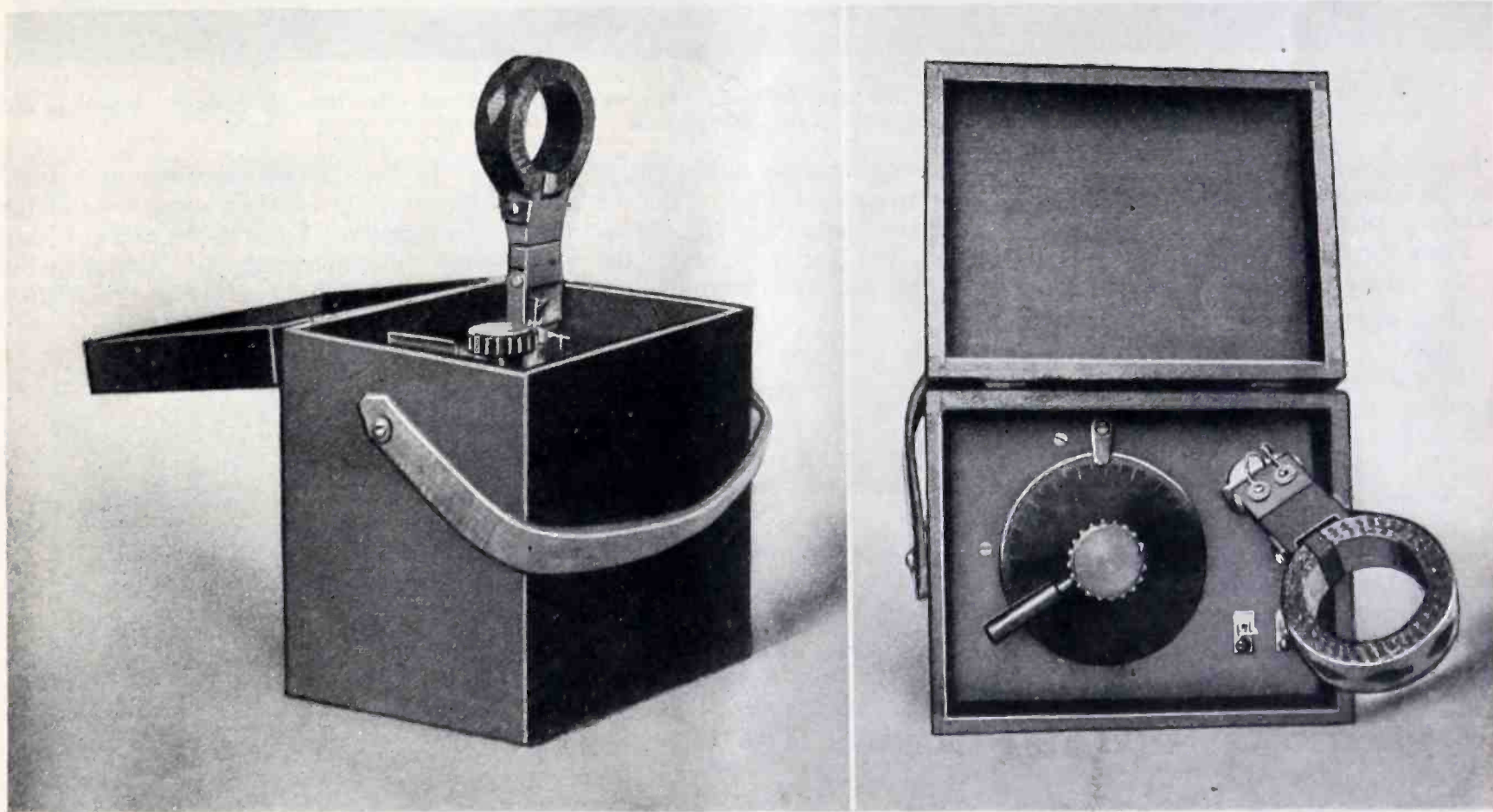
Fig. 1. The completed meter, mounted in the carrying case, ready for use
