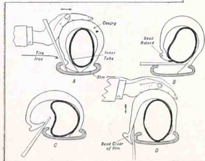
Fig. 3—How clincher casings such as used on motorcycles and Ford cars are removed from the wheel rim
