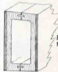
FIG. F HOLLOW SPAR Stiffened with veneer
