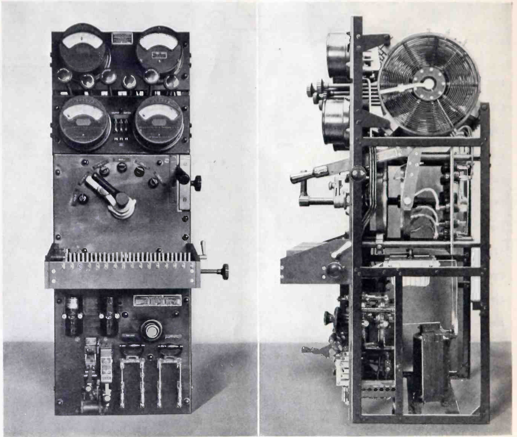
A creditable example of American radio engineering is this 500-cycle transmitter
