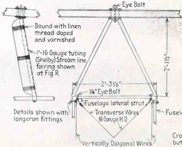
FIG. A-A CABANE STRUTS FOR SEAPLANE
