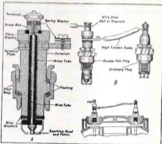
Fig. 3. Two pole spark plug for two-spark ignition
