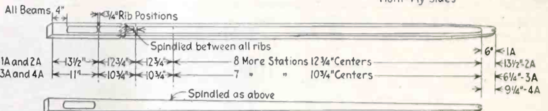
FIG. K TAPERING AND SPINDLING WING BEAMS STANDARD If wing beams are bevelled, allow for right and left when tapering. Method now seldom used.
