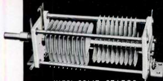
'HFB' SPLIT-STATOR TRANSMITTING CONDENSER
