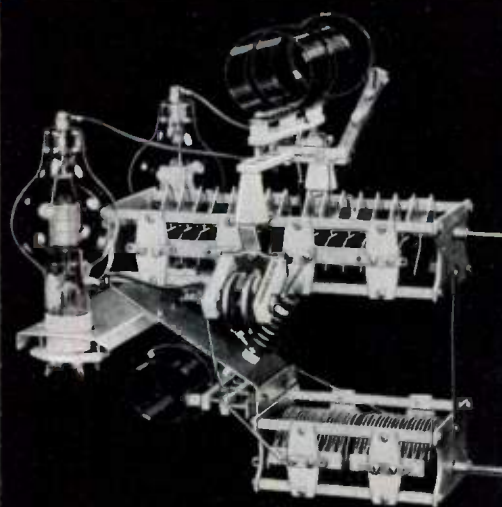
PA-500 PUSH-PULL POWER AMPLIFIER
