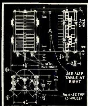
'TCD' SPLIT-STATOR TRANSMITTING CONDENSER
