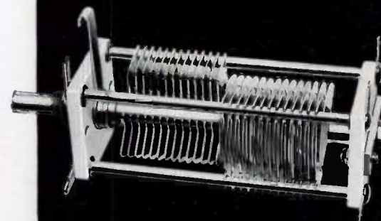
'HFA' SPLIT-STATOR CONDENSER
