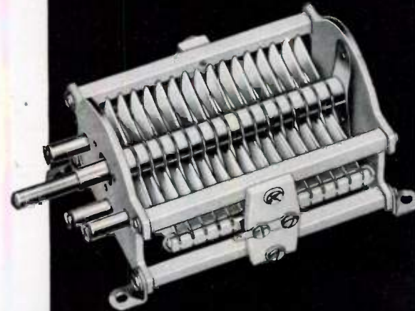
'MTC' TRANSMITTING CONDENSER
