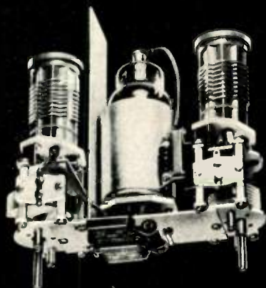
"BD-40" BUFFER-DRIVER
