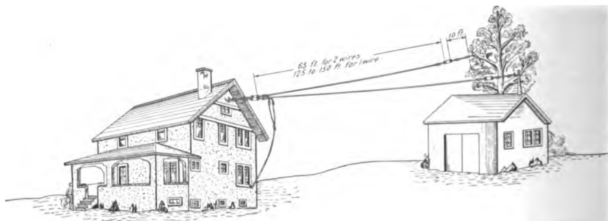
Fig. 1—Illustrating method of installing a one or two wire antenna for broadcast reception.
