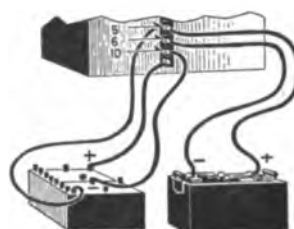
Method of connecting Filament and Plate Batteries.
