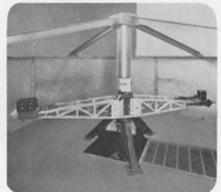
Acceleration Testing
