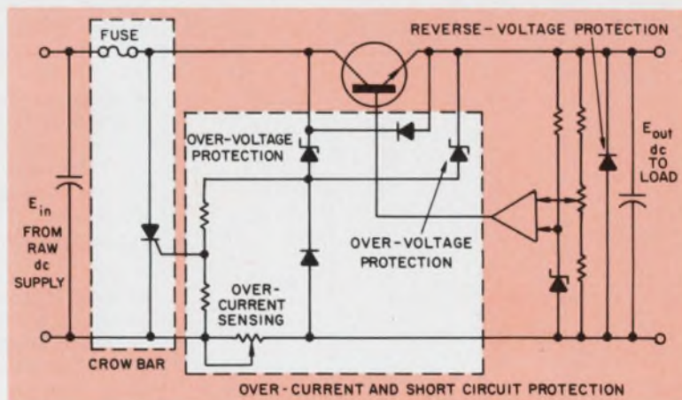
2. Fused crowbar
