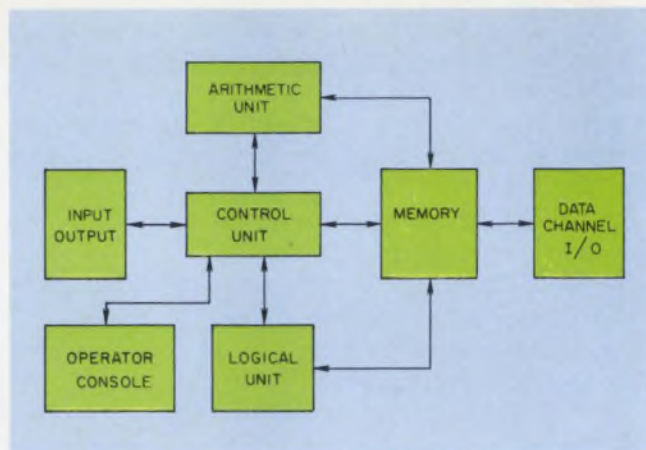
1. The system performance is keyed directly to the memory's operation in minicomputers typically organized with a centralized memory and control unit.
