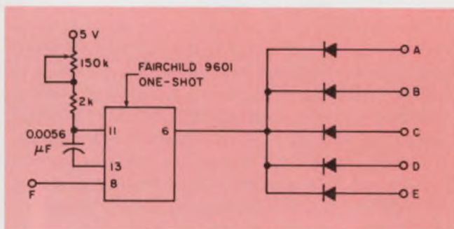
4. Use pulse-width modulation to vary display brightness. You can change display intensity from full brightness to complete blanking by adjusting the potentiometer of this diode-coupled circuit.
