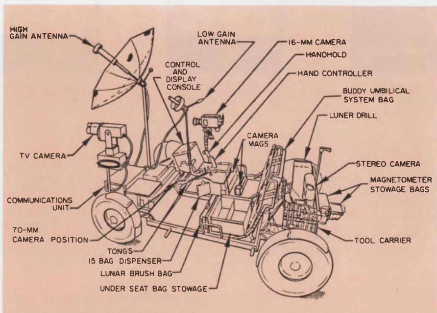
Color TV and audio signals will be transmitted directly to earth from the lunar rover. The vehicle was built by the Boeing Co.'s Aerospace Group.
