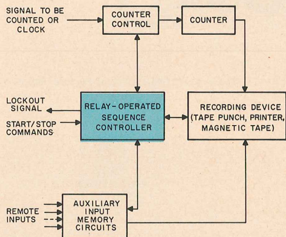
1. Basic data-processing system uses a relay-operated sequence controller as the key element in the programing sequence.
