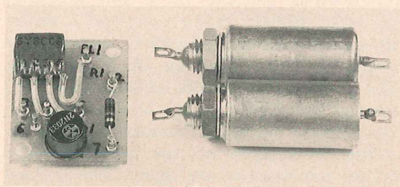
Run interference into the ground . . . Transistor-driver suppressor network (left) is more effective than heavy and bulky, conventional brute-force filter suppressor (right).
