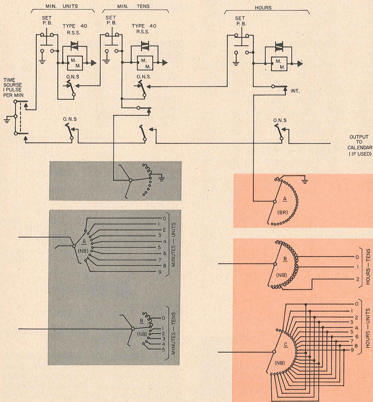
Digital clock uses rotary stepping switches to count time pulses and give 24-hour readout.
