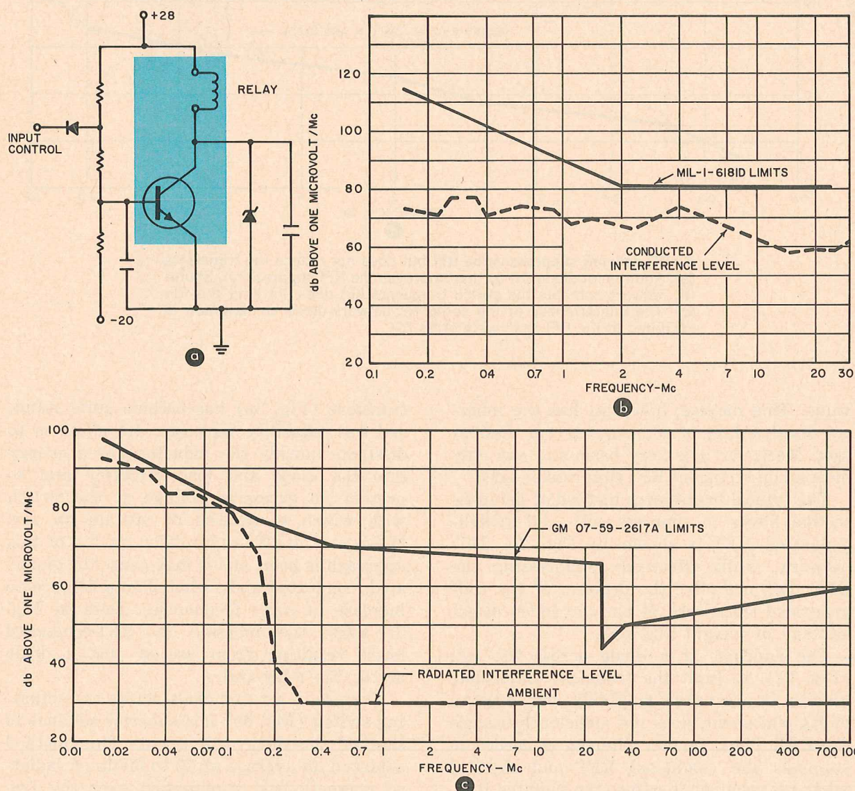
6. Typical transistor relay driver (a) is logic-operated. Conducted interference level (b) at the high side of the coil shows that even without an rf filter, the RFI level is within specifications. Radiated interference level (c) was also within specs, although shielded wiring was not used.
