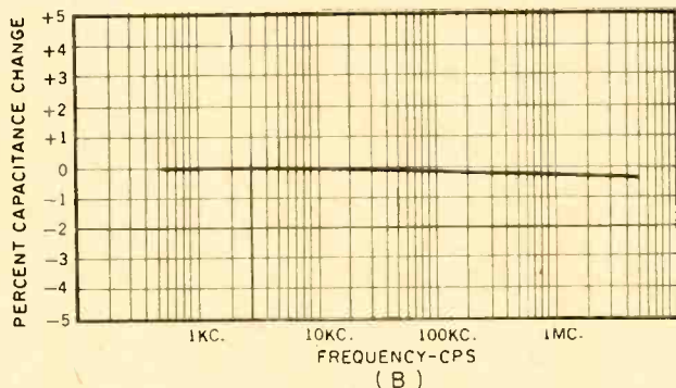
Fig. 2. (A) Quality and dissipation factor and (B) percent capacitance change with frequency for glass dielectrics.
