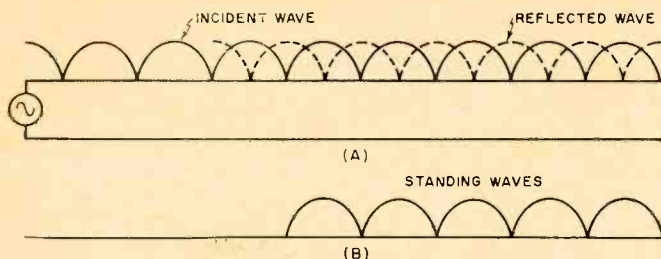
Fig. 4. When both ends of a transmission line are not terminated in the correct impedance, standing waves are set up.
