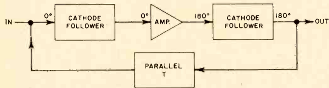
Fig. 9. Single-loop regenerative selective audio amplifier.
