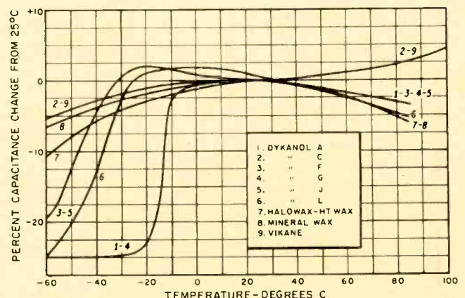
Fig. 1. Capacitance change with temperature for kraft paper dielectric material showing effects of various impregnants.
