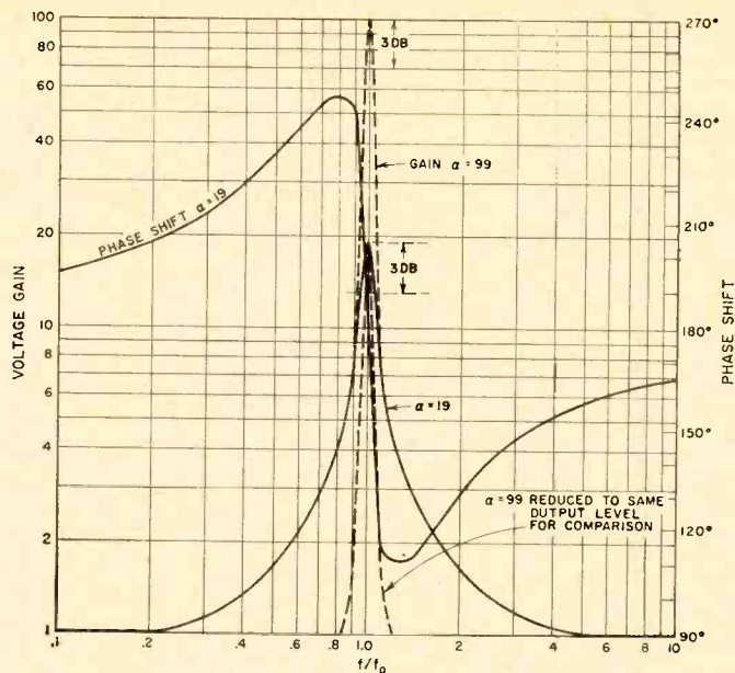
Fig. 5. Gain and phase shift of amplifier discussed in the text.
