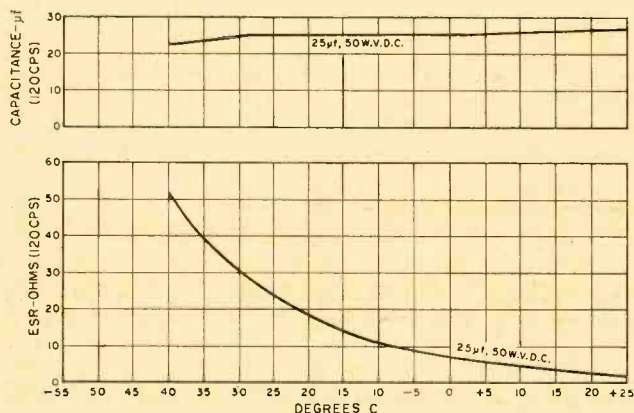
Fig. 3. Typical stability of electrical characteristics vs temperature for same type of industrial-grade capacitor.
