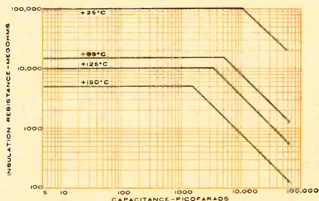
Mica capacitance insulation resistance varies with the environmental temperature present during its operation.
