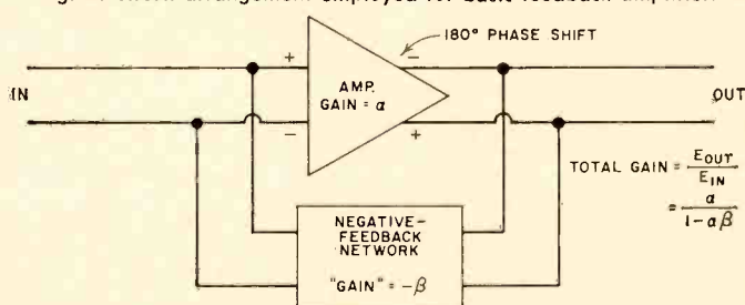
Fig. 2. Circuit arrangement employed for basic feedback amplifier.
