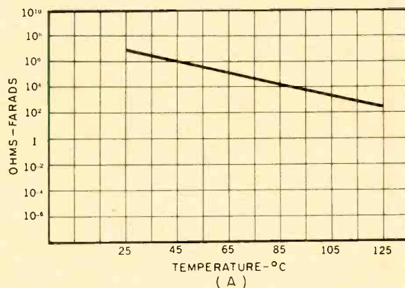
Fig. 3. (A) Insulation resistance and (B) capacitance change with frequency for glass-dielectric capacitors.
