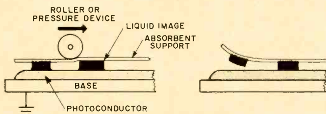
Fig. 2. Image-transfer techniques. For electrostatic transfer, the paper is given a charge opposite in polarity to that of the toner which makes the image on the photoconductor. The image is thus attracted or transferred to the copy paper. In the adhesive method, the paper to which the image is to be transferred is coated with a sticky substance to which the toner adheres. In the absorptive technique, the image on the photoconductor is liquid and when contacted by the paper, the liquid will then be absorbed directly into the copy paper.
