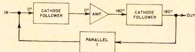
Fig. 6. Parallel-T selective audio amplifier circuit arrangement.
