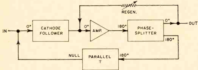
Fig. 8. Selective audio amplifier with controlled regeneration.
