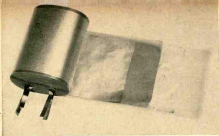
Fig. 4. (A) Paper capacitor element made with inserted contact tabs. (B) Paper capacitor element extended foil construction.
