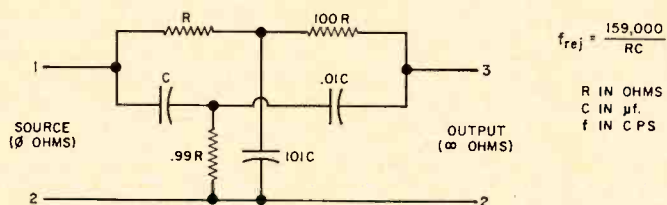
Fig. 3. The circuit constants that are used in parallel-T network.
