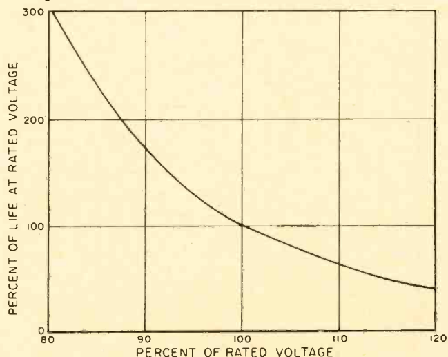
Fig. 5. How voltage affects the life of a paper capacitor.
