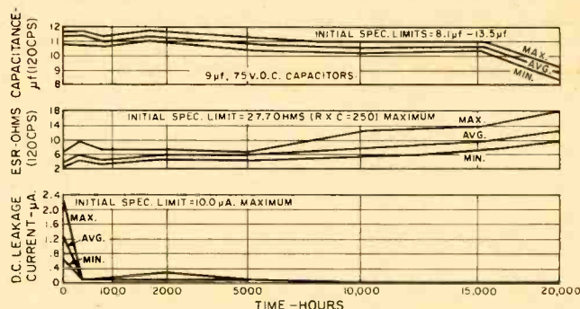
Fig. 4. Typical life test for one particular type of premium-grade can-type aluminum electrolytic unit with axial leads.
