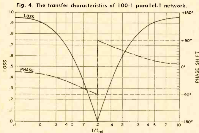
Fig. 4. The transfer characteristics of 100:1 parallel-T network.
