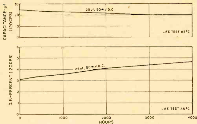
Fig. 2. A typical life test for one specific type of industrial-grade can-type aluminum electrolytic with axial leads.
