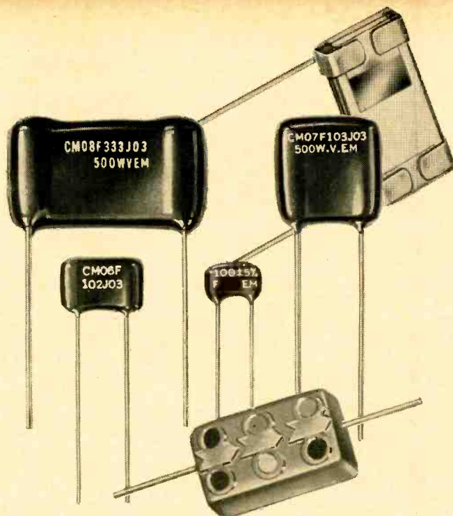
Fig. 2. An assortment of mica capacitors. Silvered mica capacitor (upper right) is shown before application of coating.
