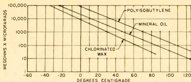
Fig. 2. Insulation resistance characteristics of paper capacitors showing effects of the various types of impregnants.
