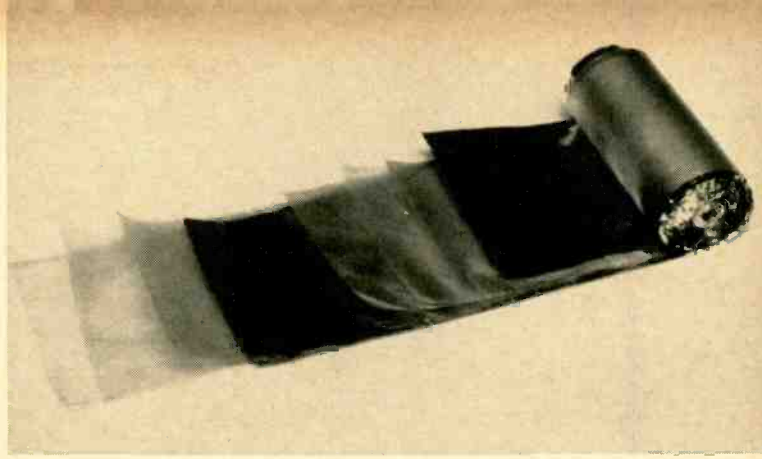
Fig. 4. (A) Paper capacitor element made with inserted contact tabs. (B) Paper capacitor element extended foil construction.
