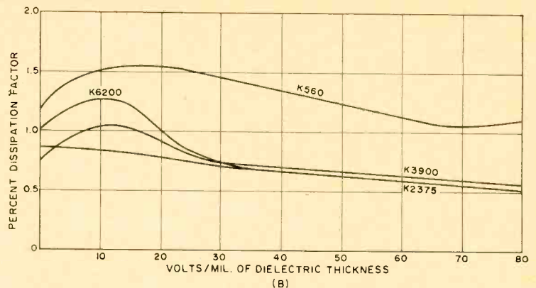
Fig. 4. The a.c. voltage coefficient of dissipation factor at 25°C and 1 kc. (B) The d.c. voltage coefficient.
