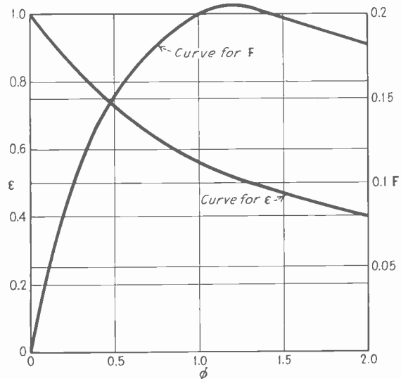
Fig. 2—Curves for F and \epsilon , referred to in text.
