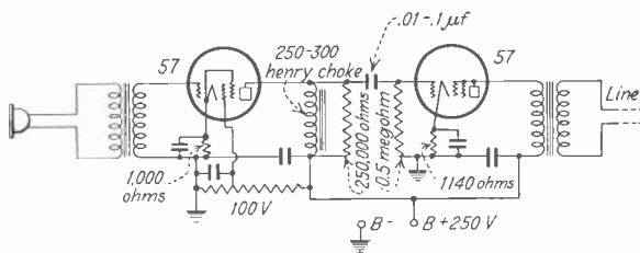
Fig. 3—A pentode amplifier using two 57 type tubes with an over-all gain of 70 db.
