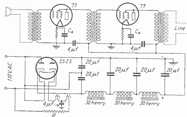
Fig. 2—Compact a.c. operated amplifier employing a voltage doubling tube
