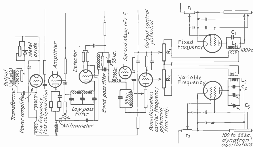
The extremely stable operation of this heterodyne oscillator results from detuning the band-pass filter.
