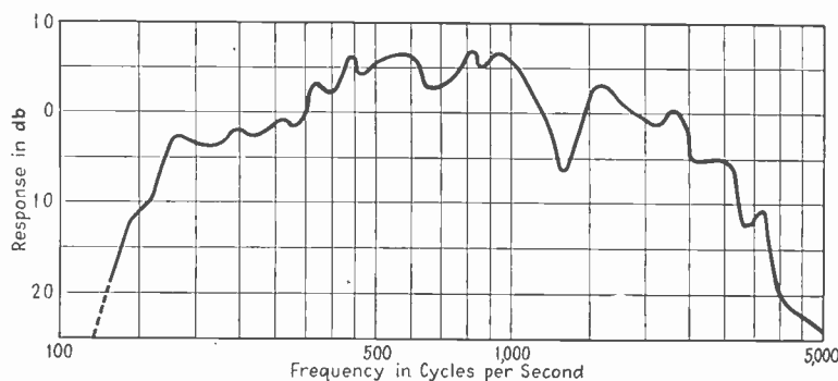
Typical response characteristic of a modern "inexpensive" receiver. Effort toward high-fidelity on the part of broadcasters is of no avail unless receivers are improved.
