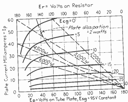
Fig. 2—Pentode curves.
