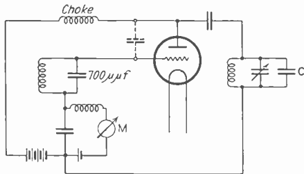
Resonant circuit for measuring capacity changes resulting from minute displacements between plates.
