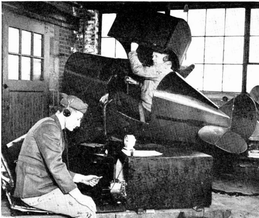
The equivalent of miniature radio beams serve to guide the pilot during his indoor instructional "blind flight"
