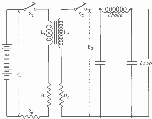
Fig. 1—Circuit for vibrator power supply.
