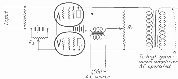
Fig. 8—Circuit for detecting and recording very small voltage changes.
