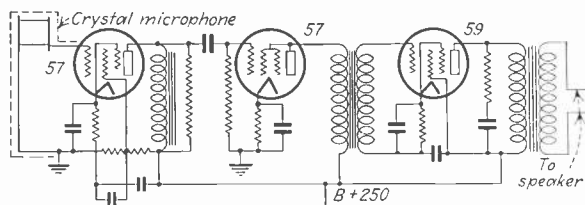
Fig. 7—Amplifier used in Zoology Department of the Connecticut State College for listening to heart beats and other cavity noises. Crystal microphone is mounted in sponge rubber.
