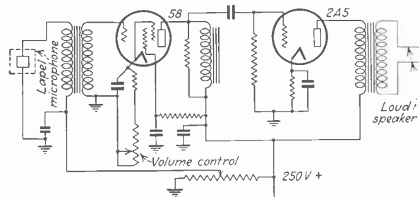
Fig. 4—Public address amplifier with an output of 3 watts operated from a lapele microphone.
