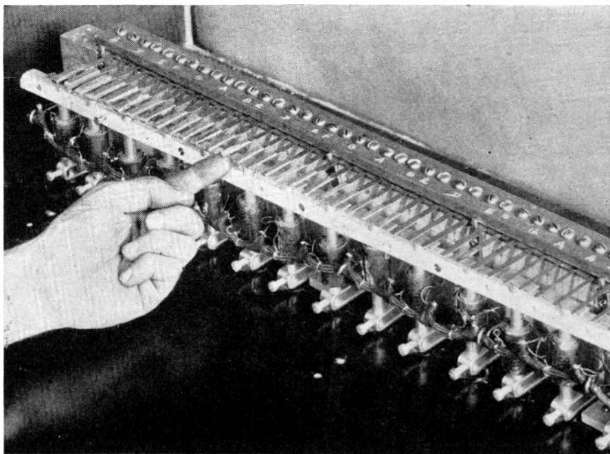
The row of tuned steel reeds, vibration of which sets up oscillatory currents which are then amplified to produce an output of 30 acoustic watts
