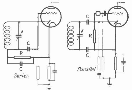
Alternative circuits for use with the binode detector.
