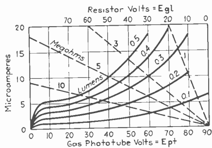
Fig. 3—Phototube curves.
