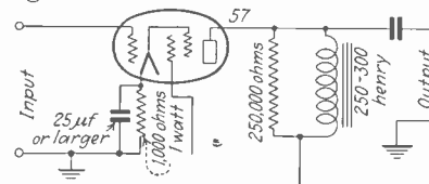
Fig. 5—Impedance coupled amplifier for high gain.
