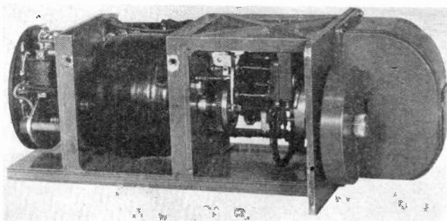
View of Finch mobile printer for police radio, inter-fleet communication or aircraft.
