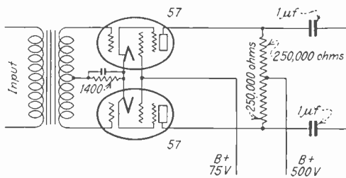
Fig. 6—Amplifier for high gain, low distortion, low noise and low hum.
