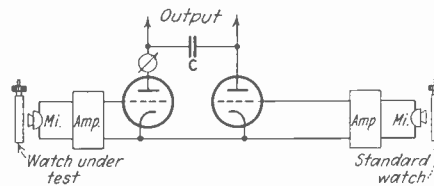
Quick and accurate regulation of watches is made possible by the use of two microphones.
