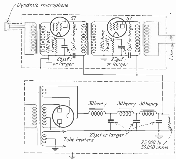
Fig. 1—A ribbon or dynamic amplifier for operation from a.c. supply
