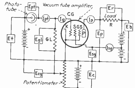
Fig. 1—Phototube amplifier circuit.
