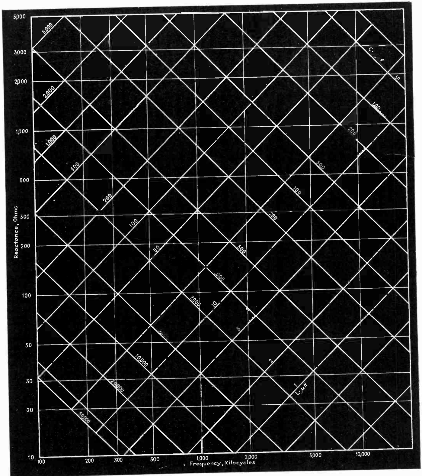
Reactance values corresponding to given values of capacitance and inductance throughout the range of the middle radio frequencies are assembled conveniently in the above chart, compiled by Edmund A. Laport. Associated with each diagonal line is a value of capacitance (C) or inductance (L), the reactance of which at any frequency can be read on the vertical scale. The intersection of two diagonal lines indicates the resonant frequency for the given value of inductance and capacity at that point.
