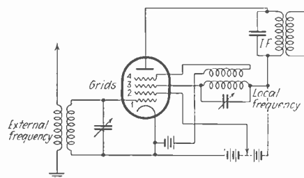
Mixing hexode connected for use at audio frequencies.
