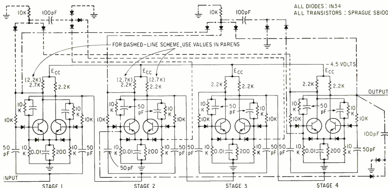
TWO DECADE SCHEMES are shown here, one in dotted lines, the other in dashed lines—Fig. 2
