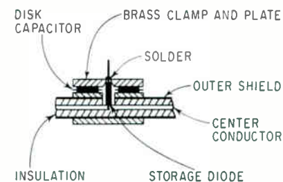
MOUNTING of charge-storage diode is provided by generator coaxial cable—Fig. 2
