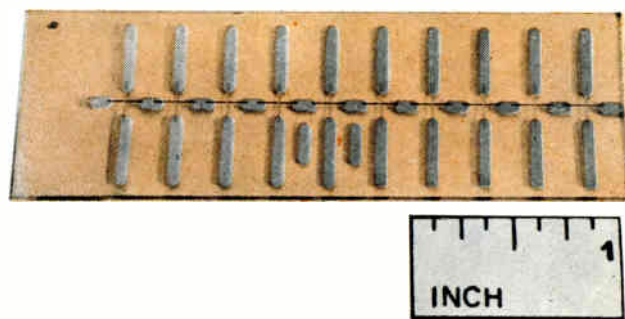
TUNNEL-EMISSION device fabrication program at Burroughs Laboratories has produced these diodes with 30-40-angstrom-thick oxide layers. Current density of 175 amp/cm 2 can be maintained and devices have worked with 35 ma d-c
