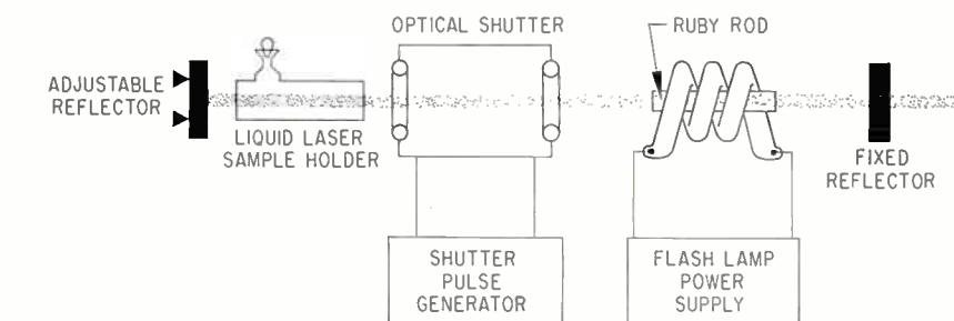
LIQUID LASER diagram shows physical arrangement of liquid sample holder, optical shutter, and ruby laser used for triggering the liquid lasing action
