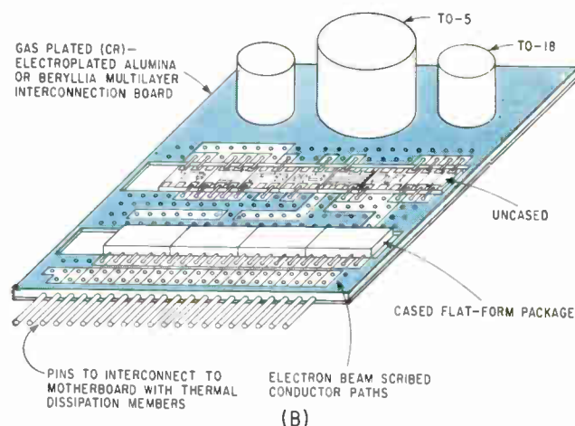
CONCEPTUAL illustration of unencapsulated hermetic header for intra-interconnection of semiconductor integrated circuits (A) and interconnection—packaging system for joining cased and uncased circuits and assembling systems (B) under study at Hamilton Standard div. of United Aircraft for ASD—Fig. 8
