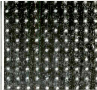
Grid screen of .003" diameter holes on .010" centers drilled in .020" stainless steel sheet.
