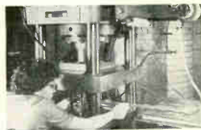
CIRCUIT CONFIGURATIONS are stamped out of copper ribbon by heated die in low-cost, mass-production process
