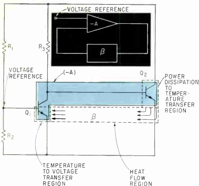
HOW THERMAL FEEDBACK reduces temperature variation of a voltage reference for analog-to-digital conversion in the telemetry encoder Texas Instruments is building for ASD—Fig. 6
