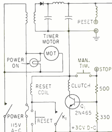
CIRCUIT DIAGRAM using transistor for timer triggering—Fig. 2
