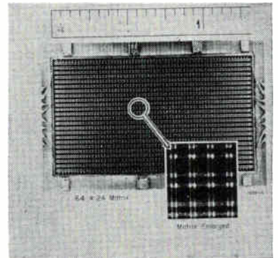
EVAPORATED memory array
