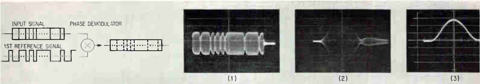
SCOPE PHOTOS showing the output of the phase modulator (1), output of the narrow-band filter (2) and the linear-detector output (3) for zero-delay correlation detection as in Fig. 3A—Fig. 4
