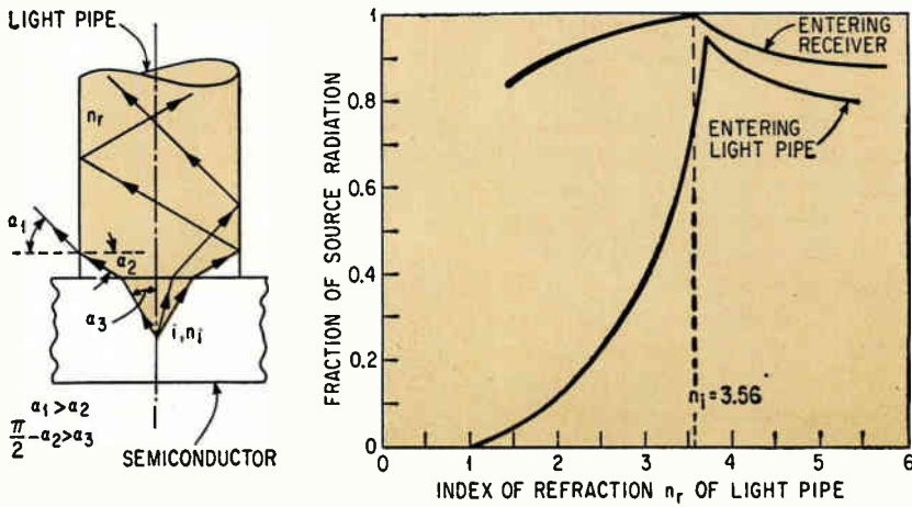
LIGHT PATHS from semiconductor source into light pipe (left) and curves showing fraction of light entering pipe from source and that reentering a receiving medium of same refractive index, as function of light-pipe refractive index—Fig. 2
