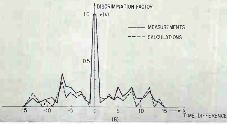
WAVEFORMS corresponding to the detection scheme shown in Fig. 3B, where photos 1 and 4 show the output of the phase modulator, 2 and 5 are narrow-band filter outputs and 3 and 6 are linear detector outputs (A) and ambiguity diagram showing discrimination factor vs time difference (B)—Fig. 5
