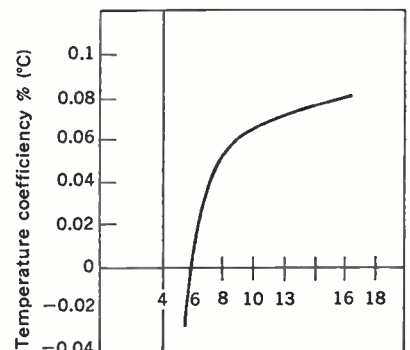
SZ-200 Temperature Coefficiency
