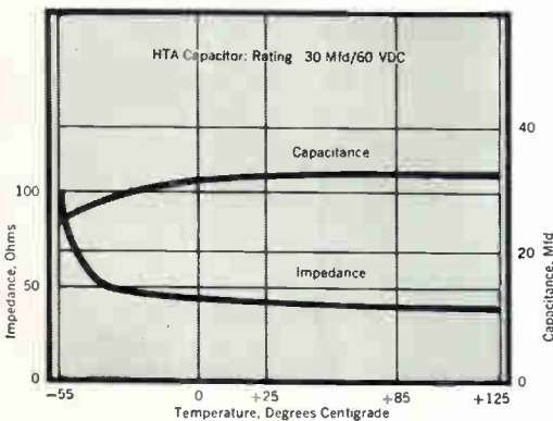
TYPICAL PERFORMANCE DATA—TYPE HTA
