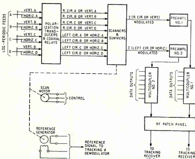
R-F (VHF) SUBSYSTEM covers from 135 to 265-Mc using orthogonal log-periodic dipole feeds; uhf r-f subsystem is almost identical—Fig. 4
