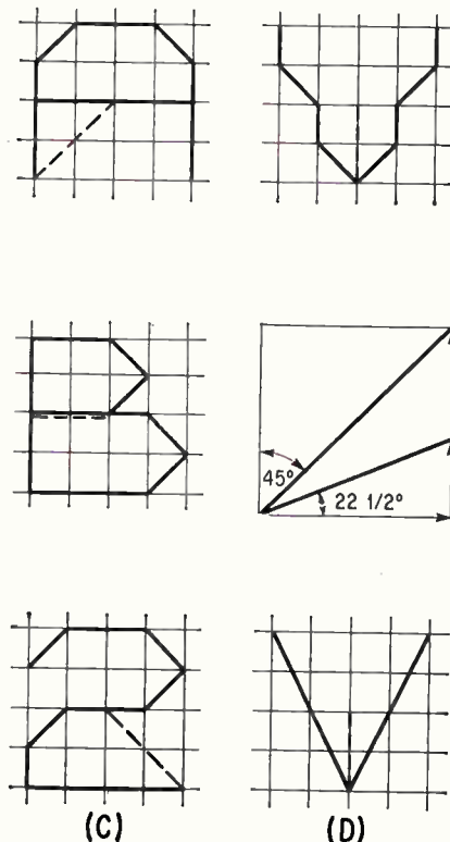
CHARGING a capacitor at constant rate from positive and negative sources (A) generates character writing waveforms (B) to produce written symbols (C). Changing the gain of one of the waveform amplifiers allows the jagged V at top of (D) to be written as straight sided V as at bottom of (D)—Fig. 4
