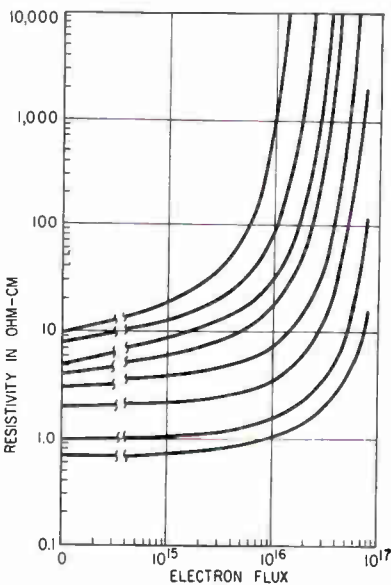
RESISTIVITY change of n-type silicon under irradiation, Fig. 3
