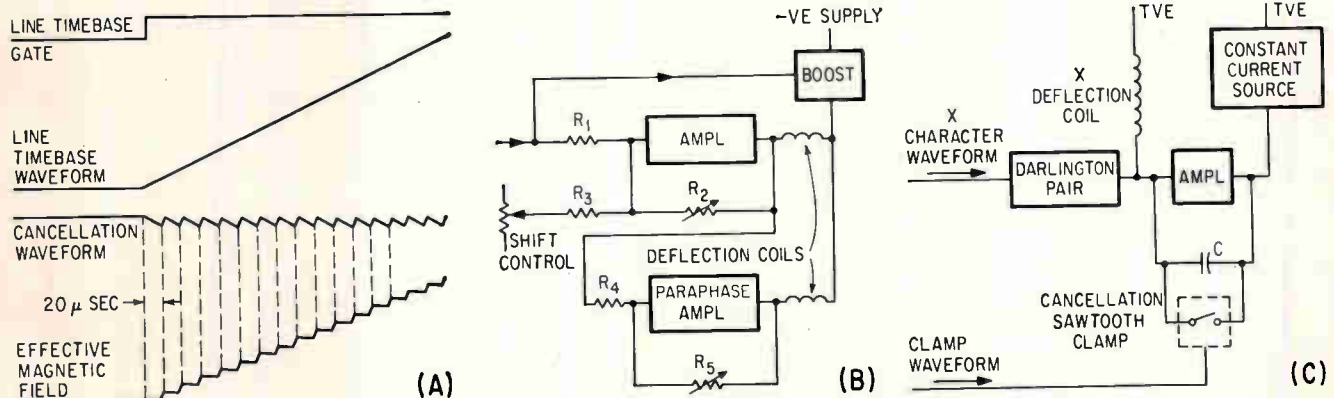
WHEN CANCELLATION sawtooth is added to line timebase wave, a staircase or stepping type magnetic deflection field is obtained (A). Main and auxiliary amplifiers in simplified form (B) and (C)—Fig. 6
