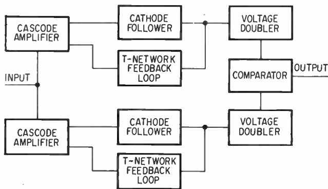
COMPLETE discriminator—Fig. 1
