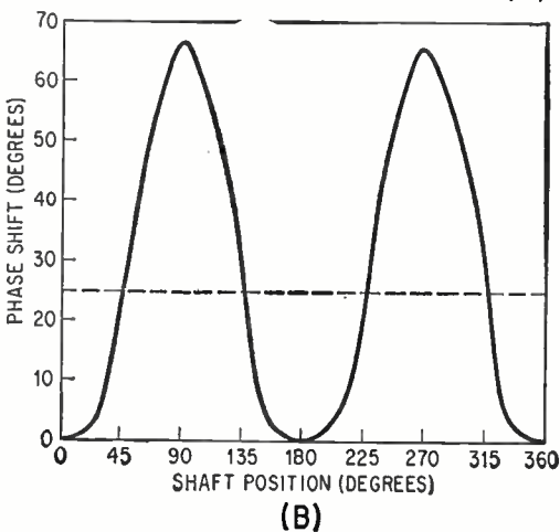
DIFFERENTIAL phase shift (A) across a greater than 3:1 band. Relative phase shift versus shaft rotation (B) at 500-Mc—Fig. 3
