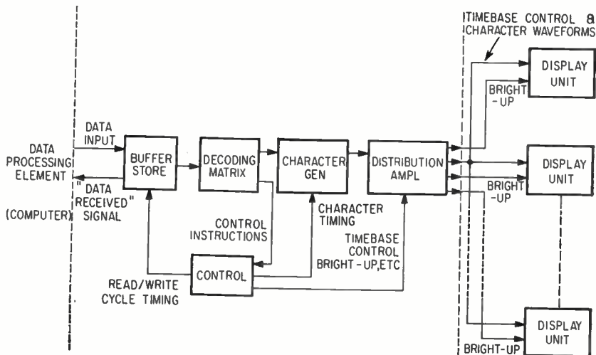
CHARACTER WAVEFORM generator and system control is in central equipment. Display units—monitors—are kept as simple as possible—Fig. 1
