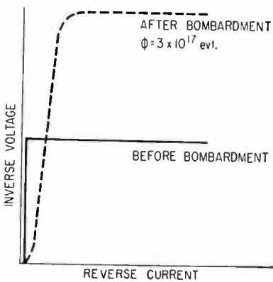
BEHAVIOR of diode's reverse characteristics under electron bombardment, Fig. 2
