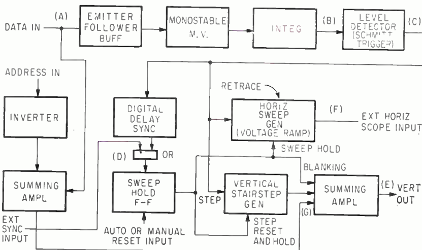
ONE MAJOR function of the circuit is to detect the 2-bit gap between words, which is accomplished by the integrator and the level detector—Fig. 2
