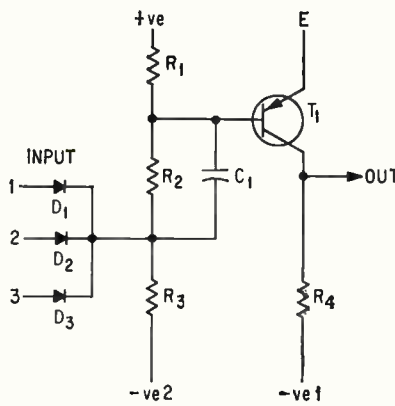
BASIC LOGIC element used in decoding circuits—Fig. 3
