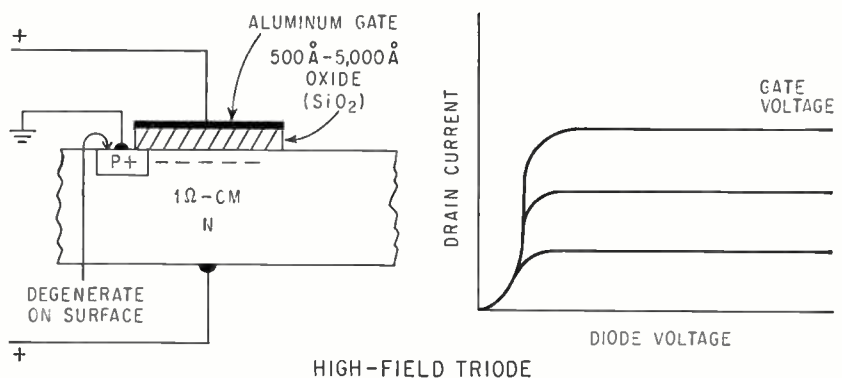
COMPARISON OF regular Westinghouse surface-controlled oxide unipolar transistor (SCOUT) and high-field triode
