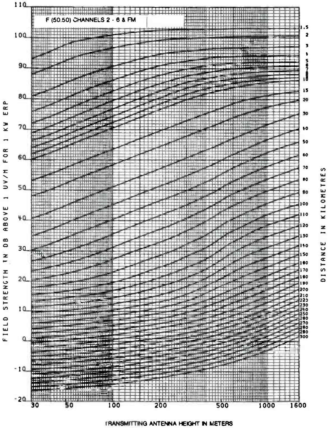
FCC 73.699 Figure 9
