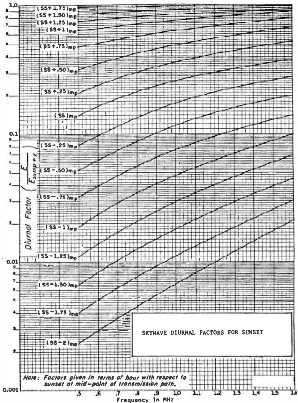
FCC §73.190 Figure 13
