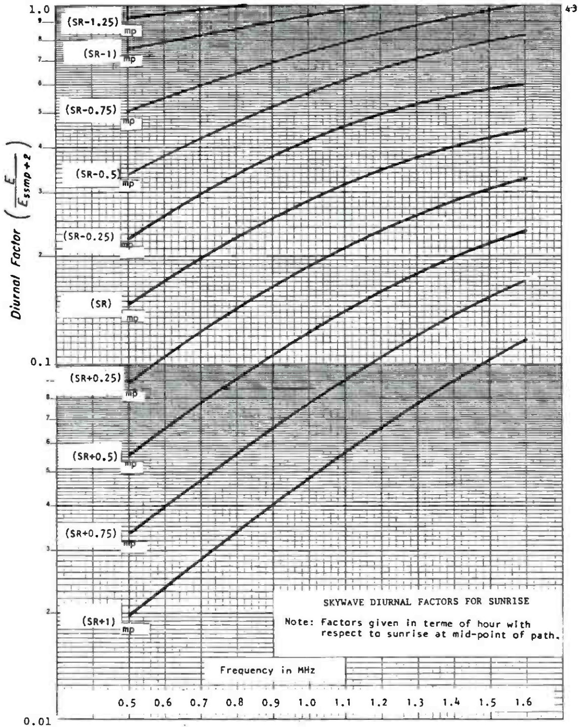
FCC §73.190 Figure 12
