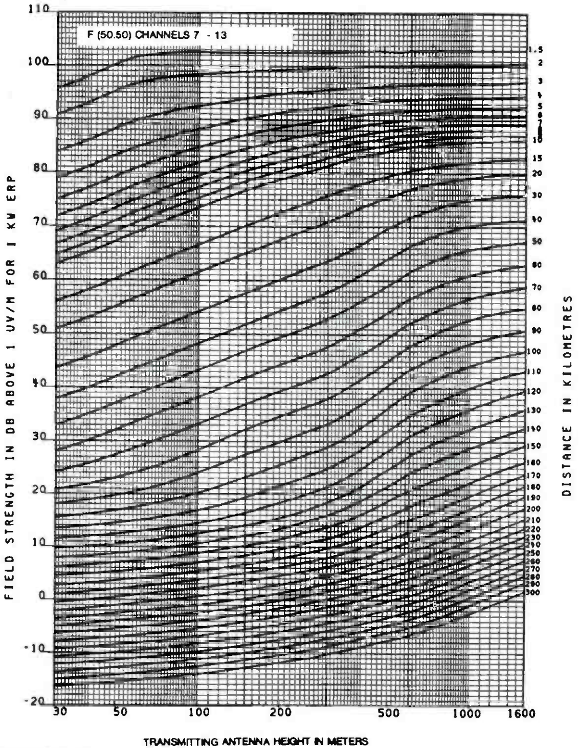
FCC 73.699 Figure 10
