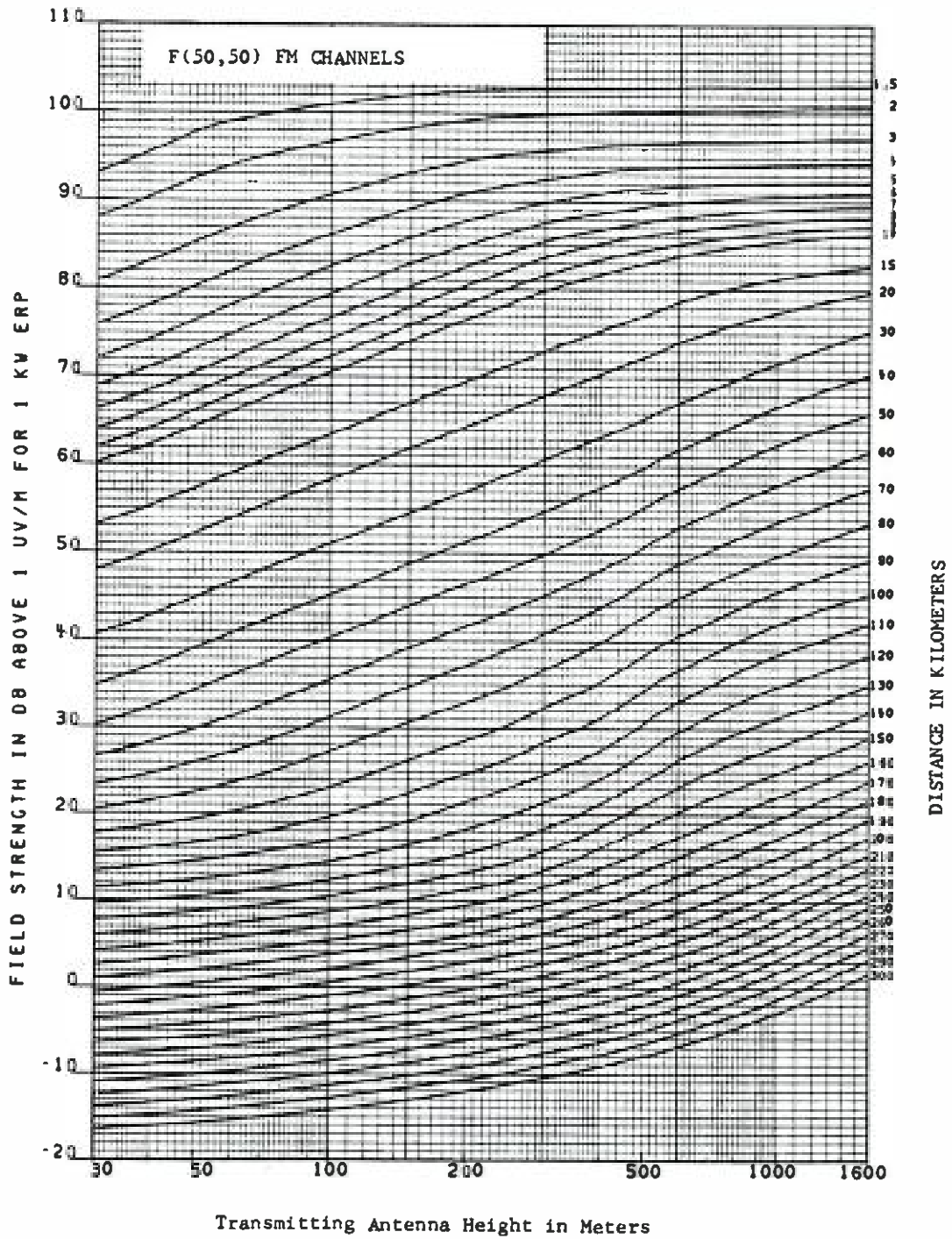
FCC §73.333 FIGURE 1
