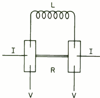
Fig. 3—Idealized Persistor memory element.
