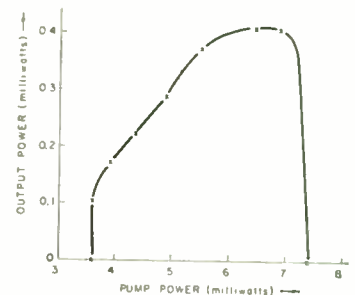
Fig. 2—Subharmonic power output vs incident pump power.
