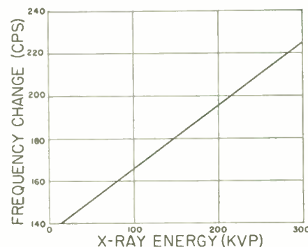
Fig. 2—Change in frequency vs X-ray energy at 300,000 R total dose.
