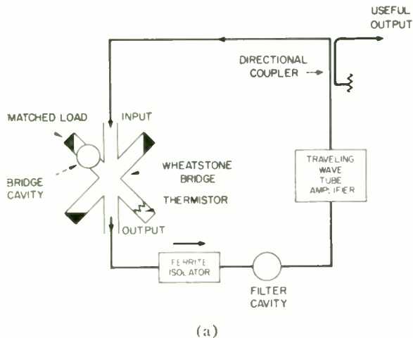
Fig. 3—Microwave Meacham bridge oscillator. (a) Basic schematic diagram. (b) Photograph of the experimental oscillator.
