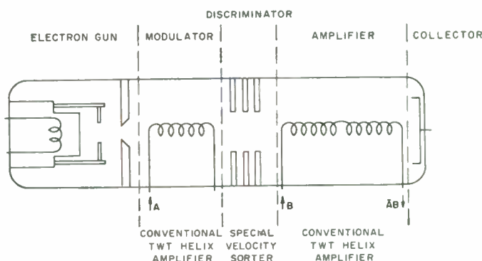
Fig. 1—Elements of switching device (IAST).
