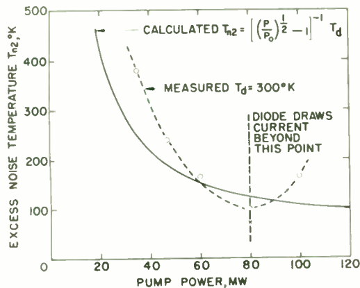
Fig. 2—Double-channel noise temperature vs pump power.
