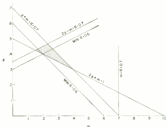
Fig. 23—Diagram delineating permissible operating range for a two-dimensional array.
