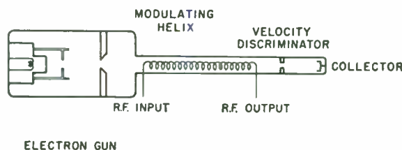
Fig. 3—Schematic of RF switch (RFS).
