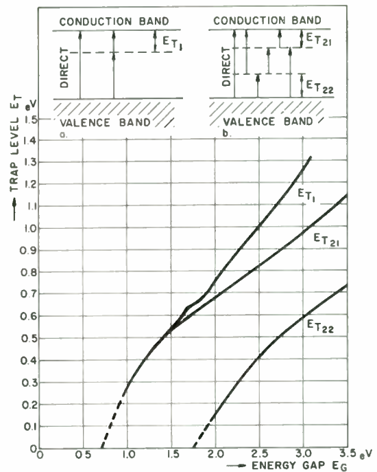
Fig. 15—The trap levels leading to optimum utilization of the sun-energy as a function of the width of the energy gap: (a) energy level diagram with one trap-level; (b) energy level diagram with two trap-levels in the forbidden gap, showing all transition possibilities.
