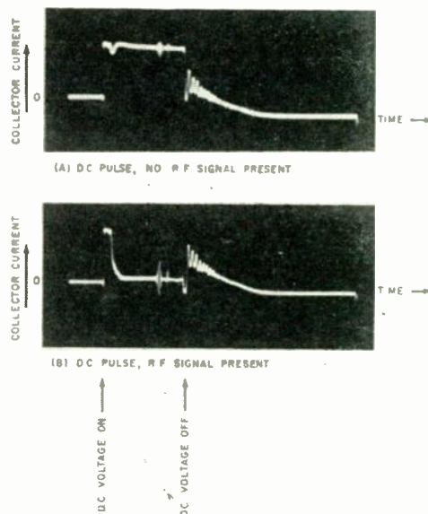
Fig. 11—DC collector current vs time for RFS showing almost complete cutoff by RF signal.
