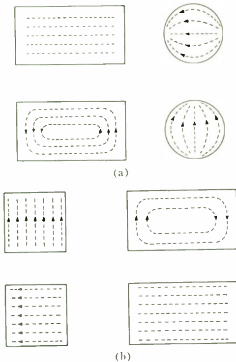
Fig. 3—(a) Radio-frequency magnetic-field configurations for the degenerate TE_{111} modes. (b) Radio-frequency magnetic-field configurations for the degenerate TE_{111} and TE_{101} modes.
