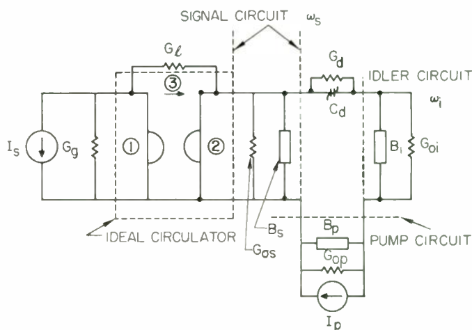
Fig. 1—Lumped-circuit model with circulator.
