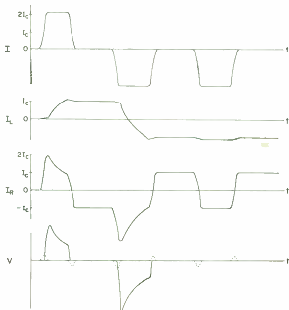
Fig. 4—Behavior of current and voltage as a function of time for an idealized Persistor memory element operated singly (not in an array).
