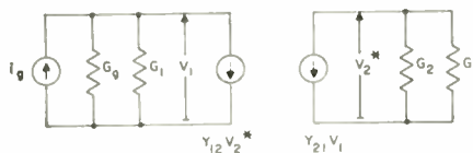
Fig. 4—Equivalent circuit of the up converter at resonance.
