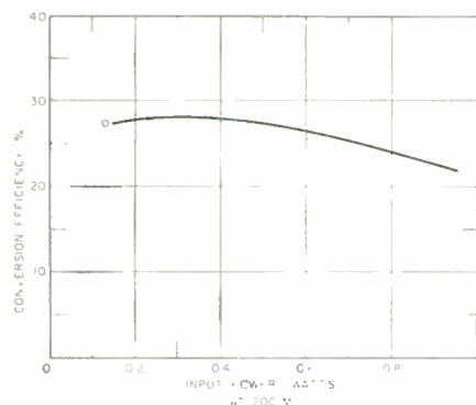
Fig. 3—218-mc-1090-mc harmonic generator, measured values of conversion efficiency.
