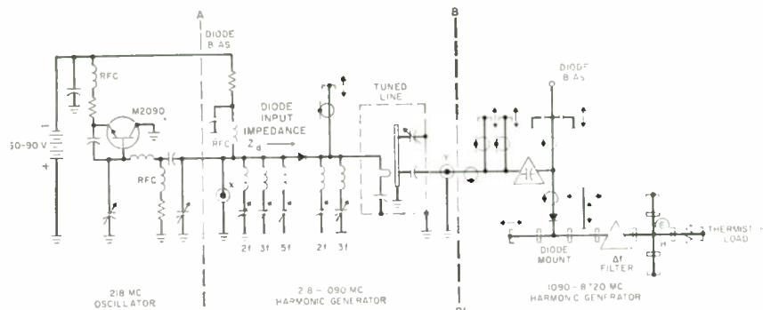
Fig. 1—Solid-state X-band source.
