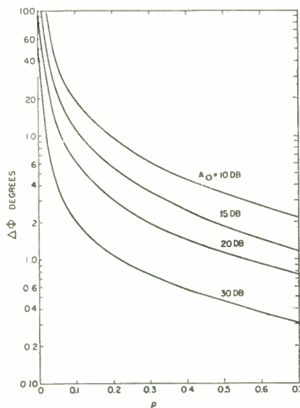
Fig. 4—Phase shift that produces a 3-db increase in gain.
