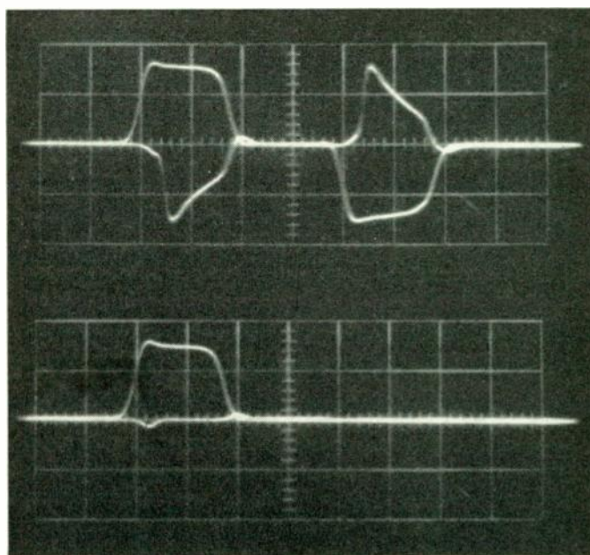
Fig. 9—Response of Persistor adjusted for slow pulses to show detail. (Time scale: 0.1 \mu\text{sec} per large division.)
