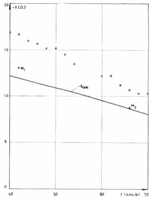
Fig. 9—Imaginary part of the impedance of the semiconductor slab of Fig. 7 as dependent on frequency. Curve calculated; circles and triangles measured as in Fig. 8.
