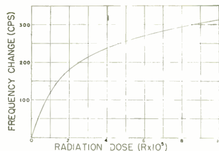
Fig. 1—Change in frequency vs accumulated dose for 300 kvp X radiation.
