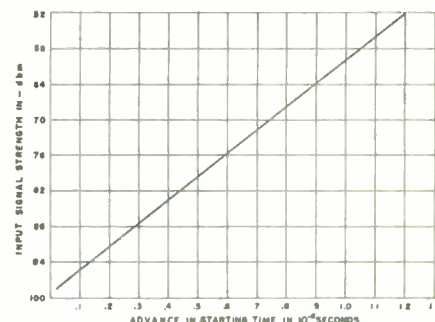
Fig. 3—Advance in oscillation starting time as a function of input signal strength.
