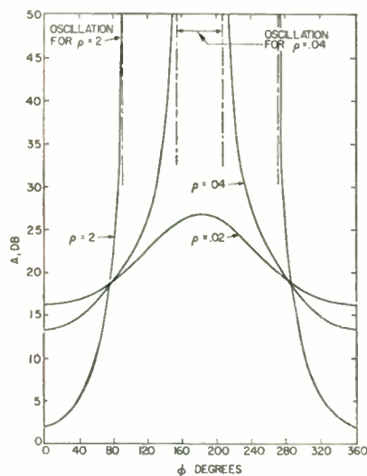
Fig. 5—Gain vs phase for three values of reflection coefficient for an initial gain A_0=20 db.
