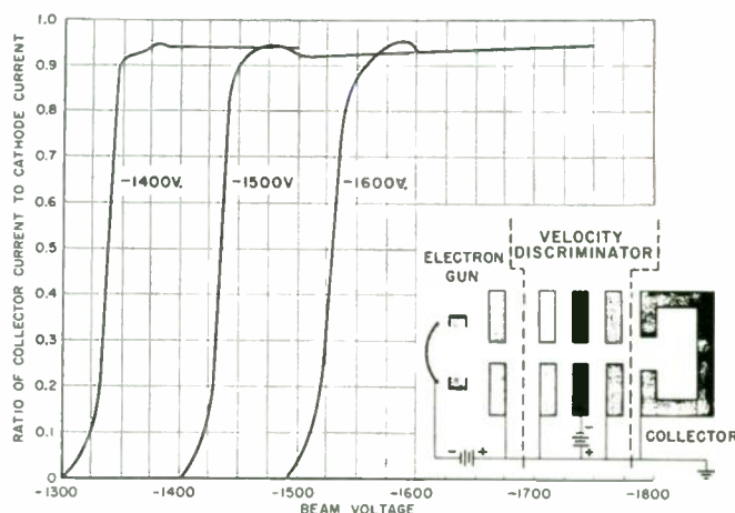
Fig. 2—Cutoff characteristics of velocity discriminator for various values of discriminator potential, and schematic of device used to determine characteristics (VDT).
