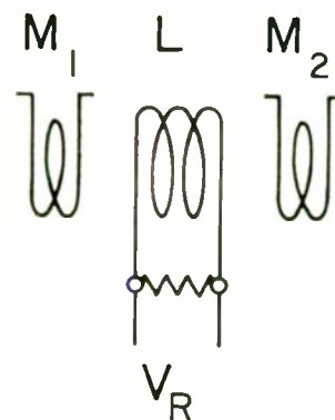
Fig. 21—Schematic diagram of mutual inductance drive for a Persistor memory element.
