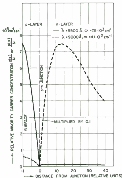
Fig. 5—Relative minority carrier distributions in the p - and n -layer at 2 different wavelengths of incident radiation: \lambda = 5500 Å, solid line; and \lambda = 9000 Å, dashed line. The distance from the surface to the p - n junction was chosen as the unit for the abscissa. Note the change of scale on the abscissa at the p - n junction, as well as the compression by a factor of 10 of the hole-distribution in the n -layer for \lambda = 5500 Å. The distributions were calculated for cell #3-329, which had the following parameters: x_j = 2.8 \cdot 10^{-4} cm; d = 5 \cdot 10^{-2} cm; \tau_p = 4.2 \cdot 10^{-6} second; \tau_n = 10^{-8} second; \mu_p = 500 cm 2 /volt sec; \mu_n = 80 cm 2 /volt sec; s = 10^3 cm second -1 .
