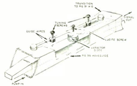
Fig. 1—Subharmonic oscillator for 34.3-kmc pump.
