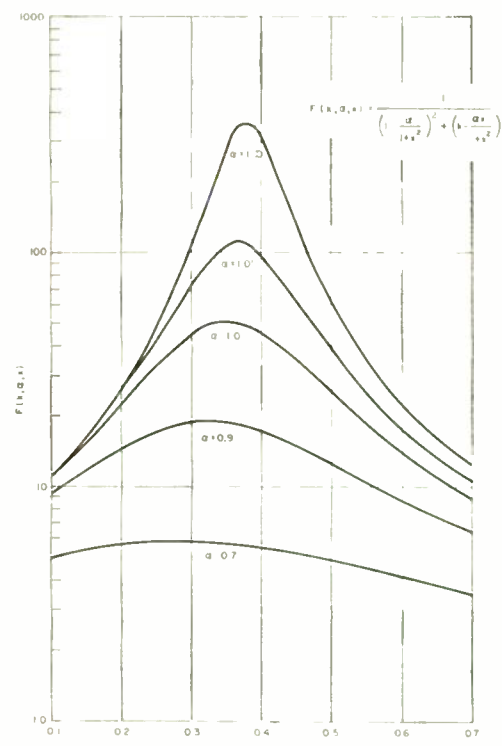
Fig. 3—Regenerative gain of straight-through amplifier as a function of the normalized idler frequency and of the stability parameter \alpha for k = 0.4 , where k denotes the normalized input susceptance.
