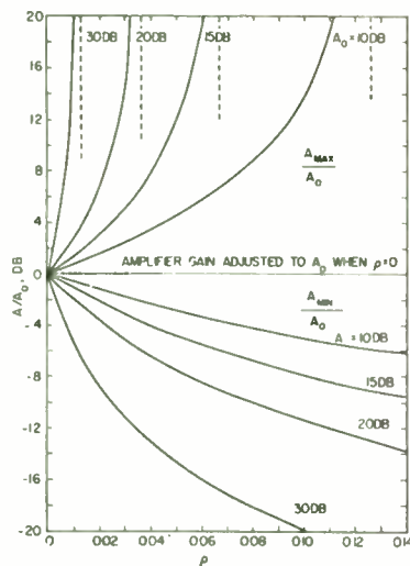
Fig. 2—Maximum and minimum gains as a function of reflection coefficient \rho . (Amplifier gain is adjusted to A_0 when \rho=0 ).
