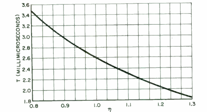
Fig. 7—Time delay of output pulse vs \eta for TWT amplifier.
