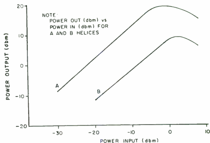
Fig. 15—Drive curves for longitudinal velocity sorting tube.
