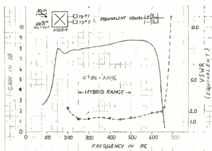
Fig. 2—Frequency response and equivalent input VSWR of hybrid coupled tunnel-diode amplifier.
