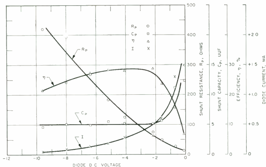
Fig. 2—218-mc-1090-mc harmonic generator, measured values of efficiency, input impedance and diode current (170-mw input power).
