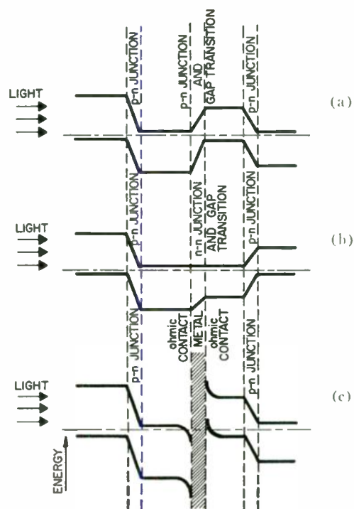
Fig. 12—Energy level diagrams for 3 possible 2-layer arrangements: (a) p - n - p arrangement (barrier for electron and hole flow); (b) p - n - n - p arrangement (light currents in both junctions opposing each other); (c) p - n -ohmic contact-metal-ohmic contact- p - n arrangement.
