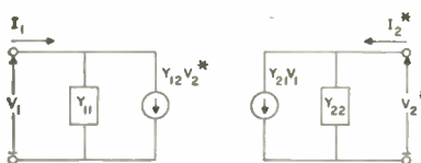
Fig. 3—Equivalent circuit of parametric diode.
