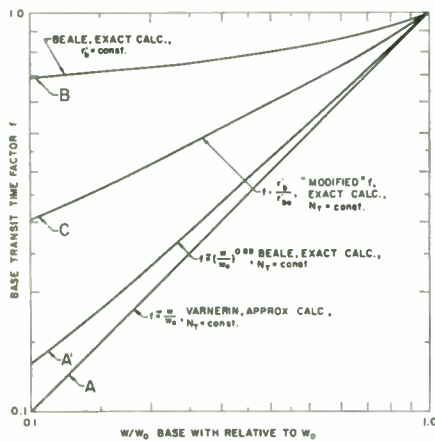
Fig. 2—Base transit time factor as a function of base thickness. Curve A, Varnierin approximate calculation for constant number of donors per \text{cm}^2 , N_T ; constant. Curve A', same case but using Beale exact calculation; curve B, Beale exact calculation for constant base resistance, r_b ; constant. Curve C, "modified" or "figure of merit" base transit time factor, f \cdot (r_b/r_{b0}) , based on Beale exact calculation.
