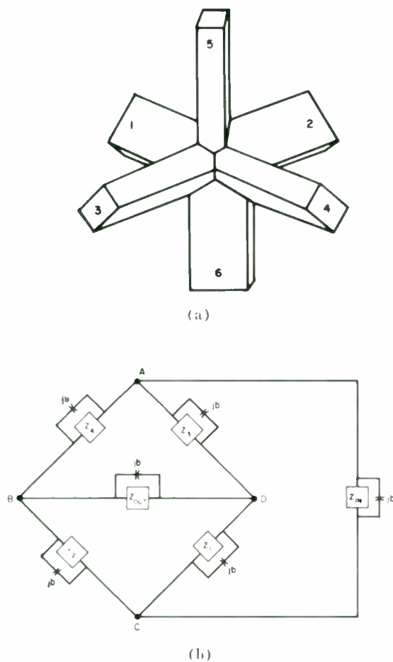
Fig. 2—Microwave Wheatstone bridge. (a) The waveguide junction. (b) Equivalent circuit.
