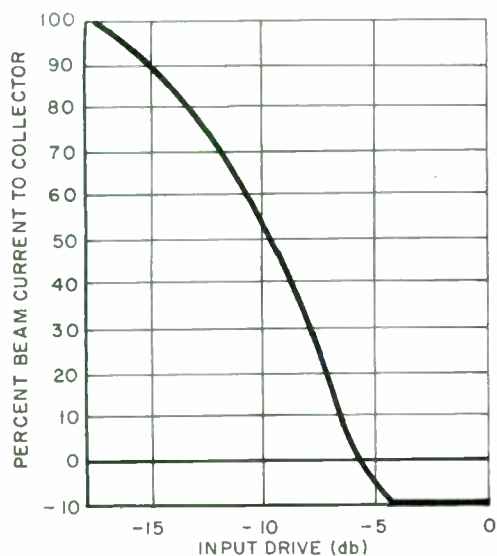
Fig. 13—Percentage of beam transmitted to collector vs input drive level for RF switch.
