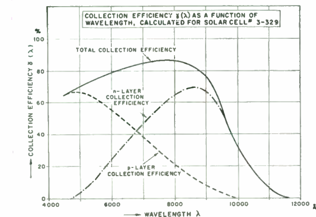
Fig. 6—Collection efficiency vs wavelength for cell #3-329 from Fig. 5. Collection efficiency from the p -layer alone (dashed), from the n -layer alone (dashed-dotted) and from the sum of both (solid) are shown.
