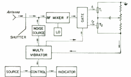
Fig. 1—Block diagram—direct reading noise figure measuring device.
