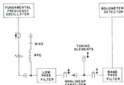
Fig. 1—Tuned harmonic generator.
