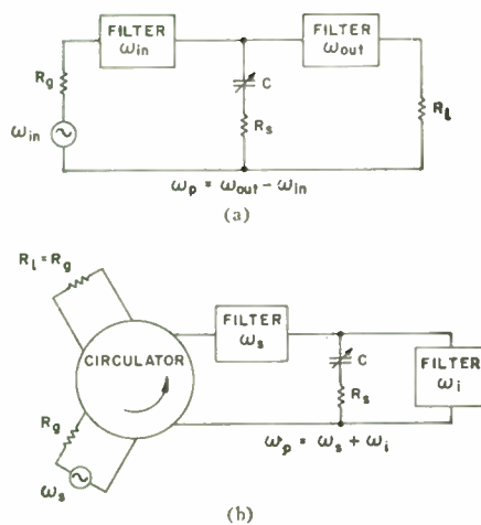
Fig. 1—Circuit models used in analysis of up-converter and negative-resistance amplifier. (a) Up-converter. (b) Negative-resistance amplifier.
