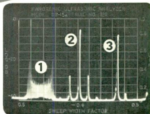
Lab setup shows SB-15a versatility. (1) FM display measures dynamic deviation. (2) & (3) are AM and SSB signals, respectively, with sine wave modulation.
