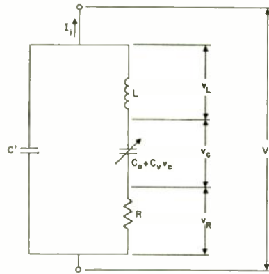
Fig. 1—Equivalent circuit of diode.
