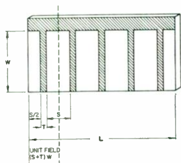
Fig. 9—Configuration of a contact grid structure.
