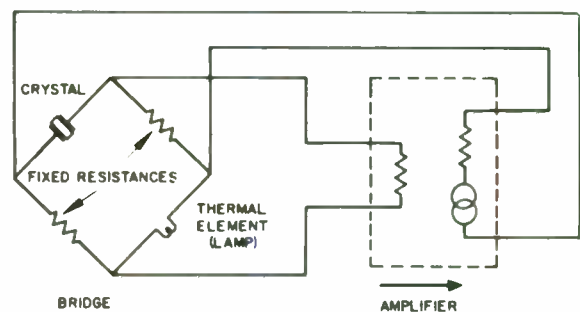
Fig. 1—Low-frequency Meacham bridge quartz-crystal oscillator.
