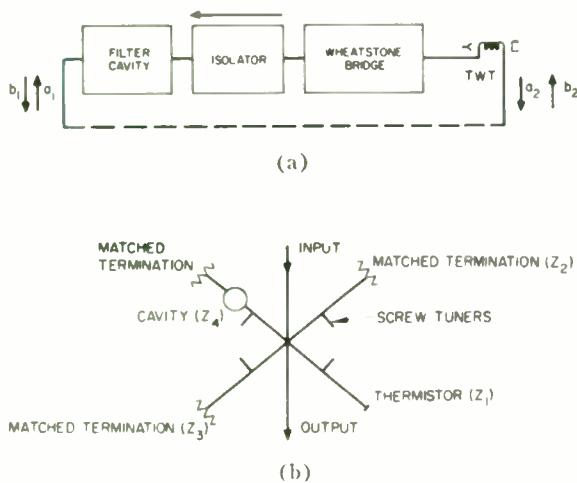
Fig. 4—Microwave Meacham bridge circuit representation used in the analysis. (a) Incident and reflected wave representation. (b) Details of microwave bridge.
