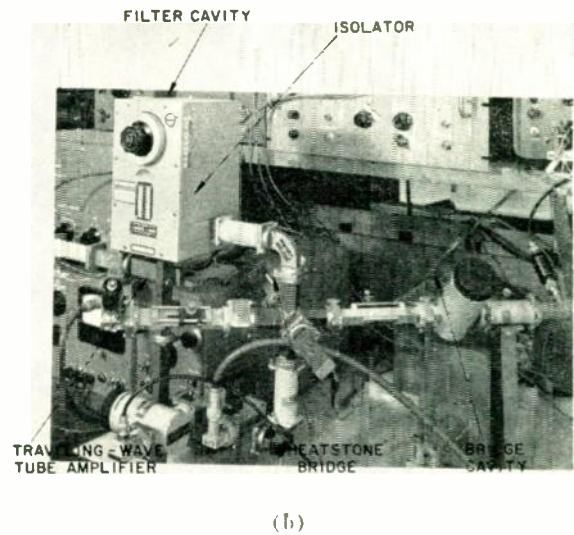
Fig. 3—Microwave Meacham bridge oscillator. (a) Basic schematic diagram. (b) Photograph of the experimental oscillator.
