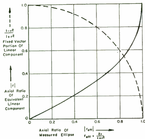
Fig. 4— |r| and \frac{1-r^2}{1+r^2} vs |r_{\text{eff}}| .
