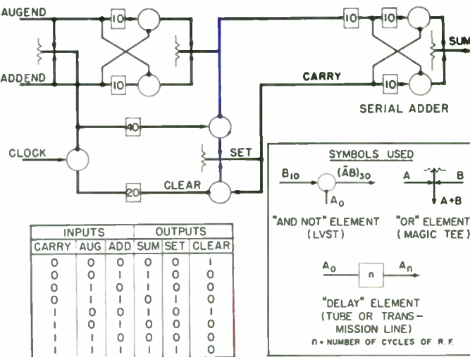
Fig. 9—Example of computer application of an LVST taking delay times into account ("and not" element) with an inherent delay of 30 cycles of RF.
