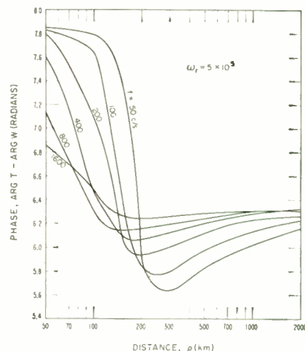
Fig. 2—The phase (lag) of the impedance ratio W/T as a function of distance \rho , h=90 km.
