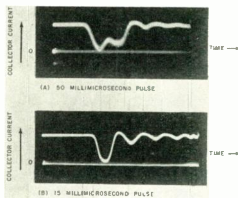
Fig. 12—Collector current vs time for RFS with short RF pulses; scale: m \mu sec/div.
