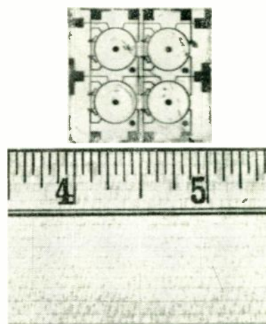
Fig. 8—A 2×2 Persistor array produced by vapor deposition.
