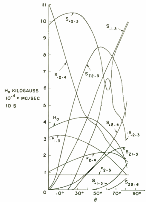
Fig. 8—Curves of the operating parameters for ruby with the two intermediate levels as amplifying levels.
