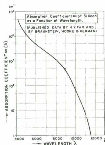
Fig. 2—Absorption coefficient \alpha vs wavelength \lambda for silicon in the range of interest for solar energy conversion. (Published data by H. Y. Fan, M. L. Shepherd and W. Spitzer, "Intra-Red Absorption and Energy-Band Structure of Germanium and Silicon," John Wiley and Sons, Inc., New York, N. Y.; 1956, and by R. Braunstein, A. R. Moore and F. Herman, "Intrinsic optical absorption in germanium-silicon alloys," Phys. Rev. , vol. 109, p. 695; February 1, 1958.)
